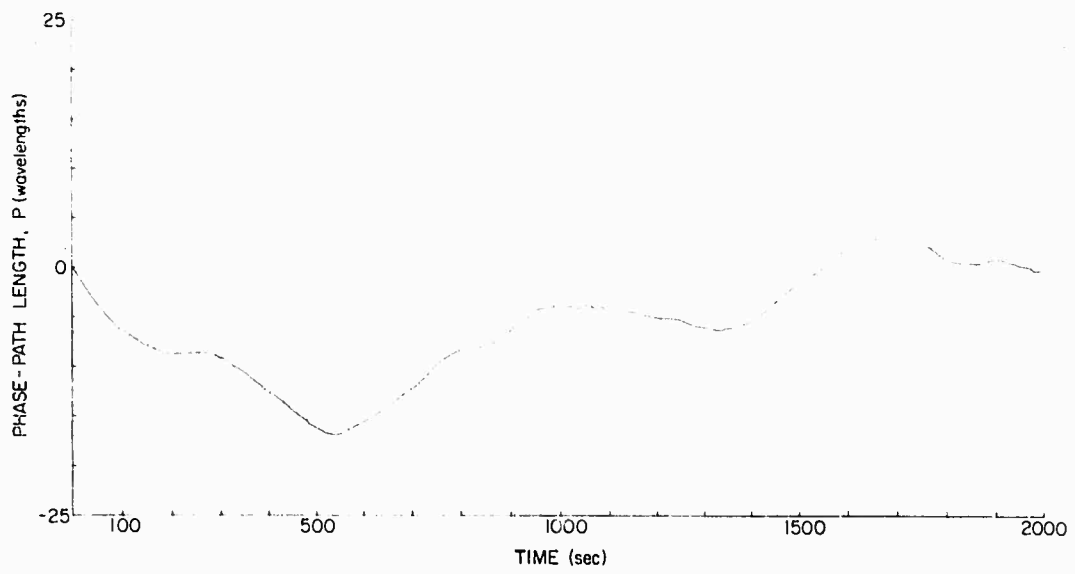
Figure 16. Phase-path length measurement for very quiet ionospheric conditions.
