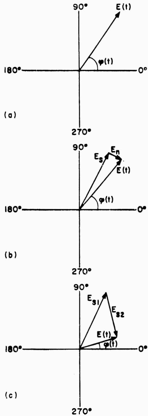
Figure 4. Vector representation of received signals.
