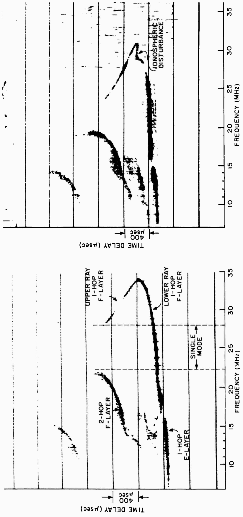
(a) Quiet ionosphere. (b) Disturbed ionosphere.
