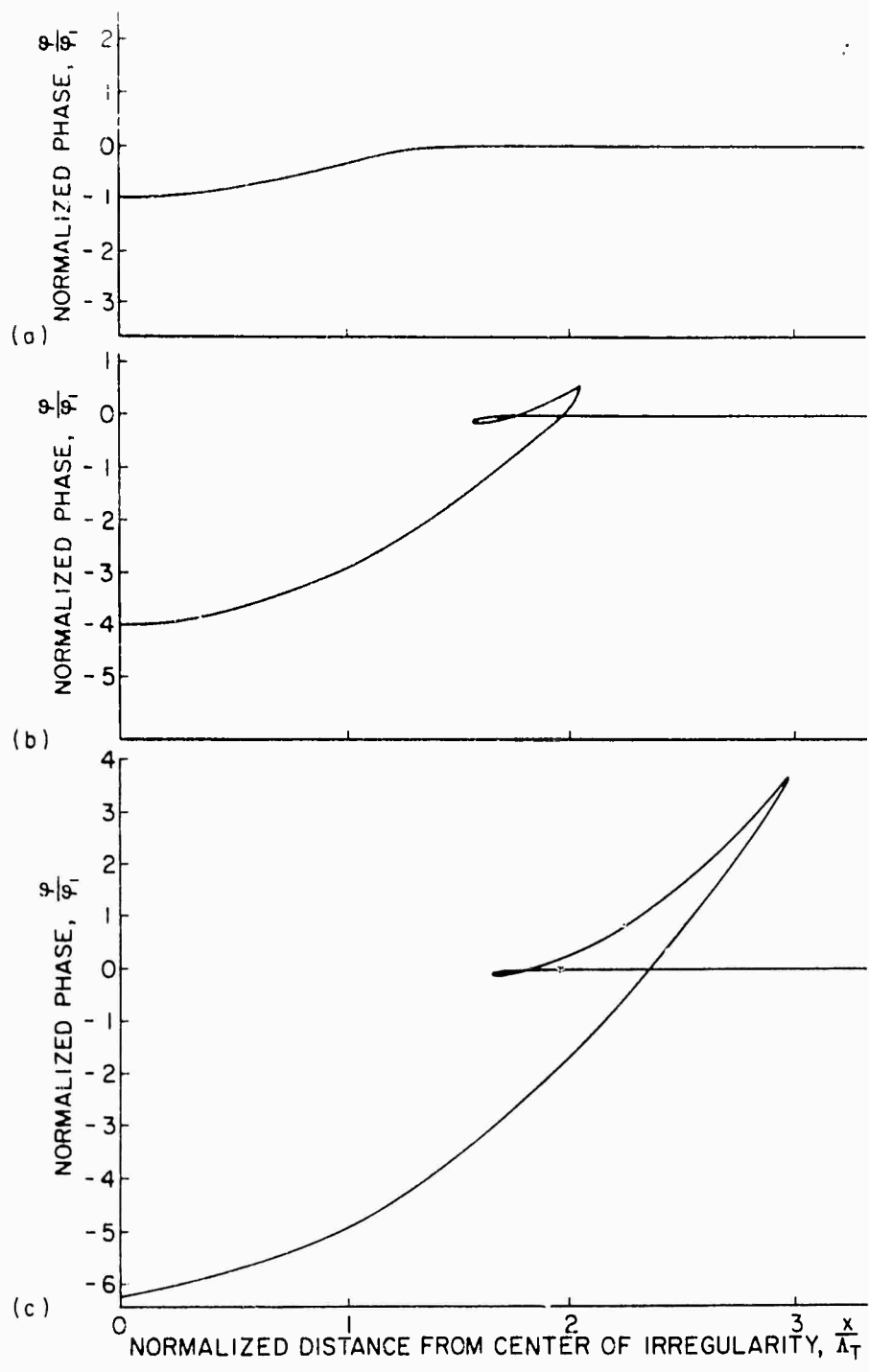
Figure 12. Computed received wavefronts for waves propagating through a gaussian irregularity.
