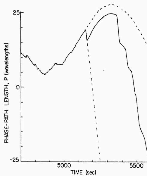
Figure 18. Phase-path length measurement alternately captured by two rays of comparable amplitude.
