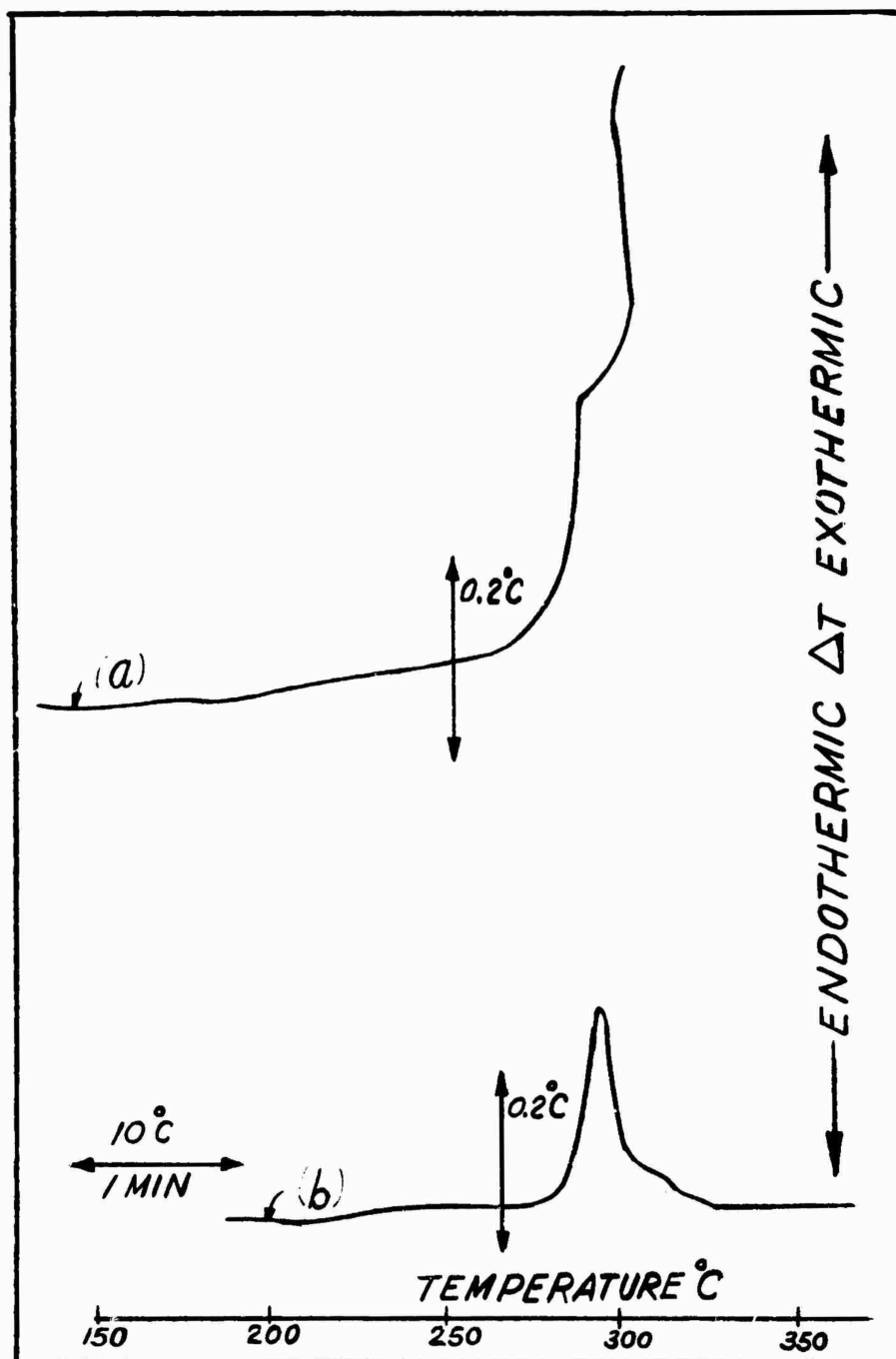
DTA CURVES FOR LEAD AZIDE (a) SAMPLE DETONATED (b) SAMPLE DECOMPOSED TO FORM OXIDES OF LEAD
