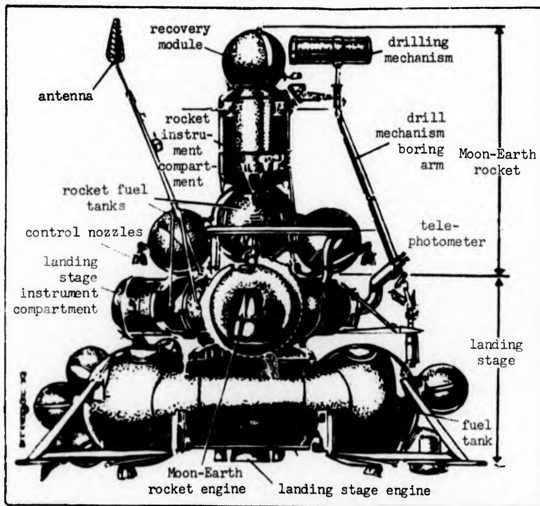
The station Luna-16
