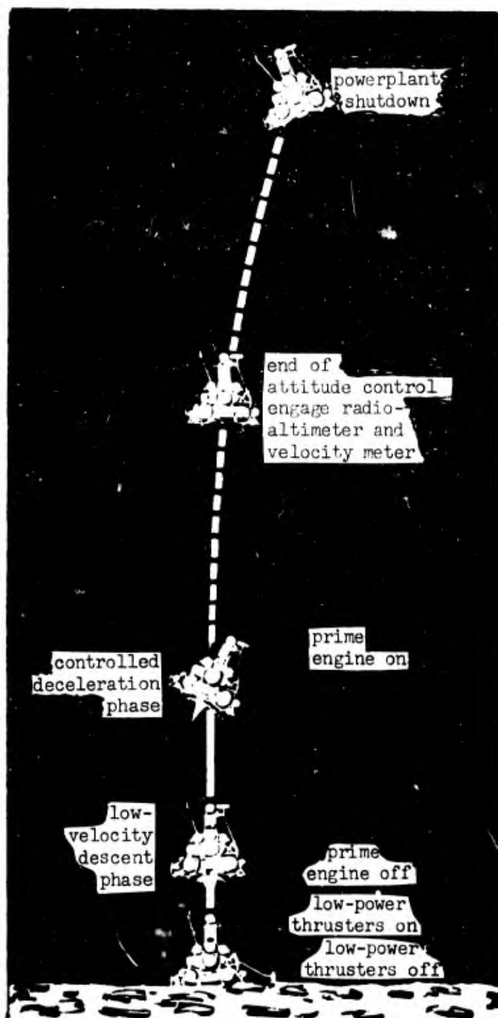
Diagram of the landing of Luna-16 on the Moon
