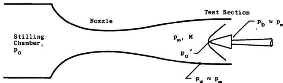
Fig. 1 Location of Extreme Pressures in a Typical Wind Tunnel
