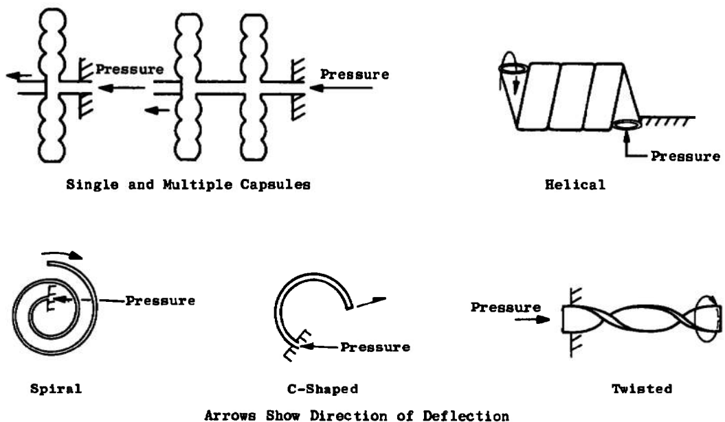
Fig. 5 Potentiometric Transducer Force-Summing Members
