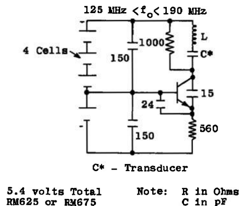
Fig. 73 Clapp Oscillator
