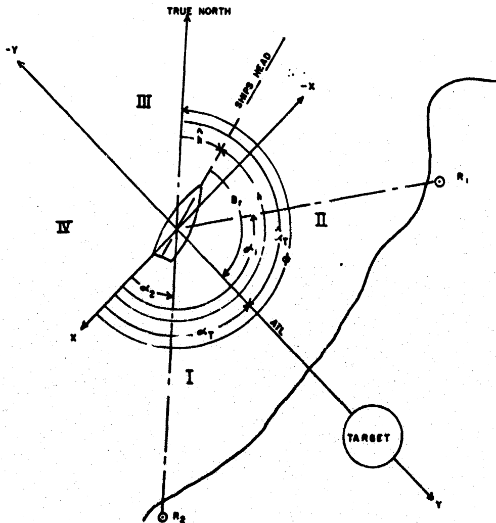
FIG. 1(c) RELATIONSHIP BETWEEN COORDINATE SYSTEMS
