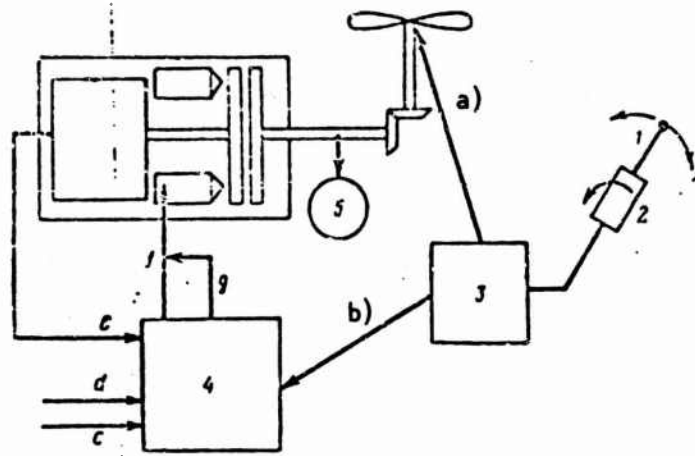
Figure 49. Diagram of Pitch-Gas System for Helicopter with Gas Turbine Engine: 1, "Pitch-Gas" lever; 2, Turbine compressor operating mode corrector; 3, Mechanism coupling operating modes of engine and rotor; 4, Rotating speed regulator for turbine compressor; 5, Free turbine rpm indicator: a, Signal to change rotor pitch; b, Signal to change engine operating mode; c, Signal indicating pressure of surrounding medium; d, Signal indicating temperature of surrounding medium; e, Signal indicating rotating speed of turbine compressor; f, Fuel supply to engine; g, Fuel pressure rise limiter.
