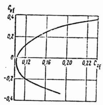
Figure 27. Polar Diagram of Mi-6 Helicopter Fuselage.
