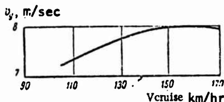
Figure 64. Vertical Rate of Climb as a Function of Flying Speed of Mi-6 Helicopter with Cargo Suspended Externally at Nominal Engine Operating Mode: G = 37 T , H = 450 m, P = 760 mm Hg, t_{1r} = 10^{\circ}C , \eta_{1r} = 83\% .
