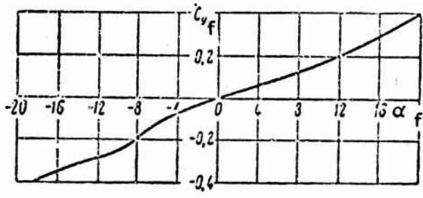
Figure 26. Lift Factor of Fuselage of Helicopter as the Function of Angle of Attack.
