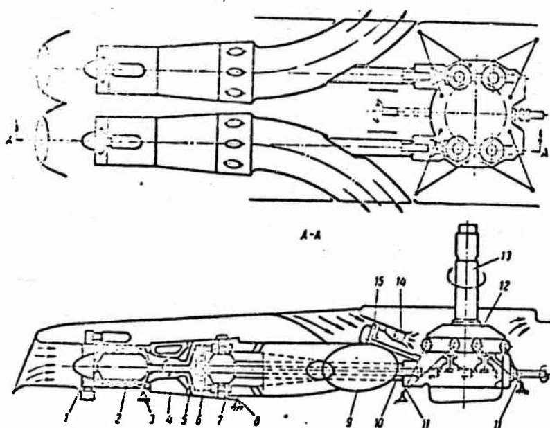
Figure 9. Diagram of Power Plant of Mi-6 Helicopter: 1, compressor intake body; 2, compressor; 3, front motor support; 4, combustion chamber; 5, compressor turbine; 6, free turbine (rotor turbine); 7, body of rotor turbine; 8, rear engine support; 9, exhaust pipe; 10, transmission; 11, reducing gear fastening points; 12, main reducing gear; 13, lifting rotor shaft; 14, radiator; 15, fan.
