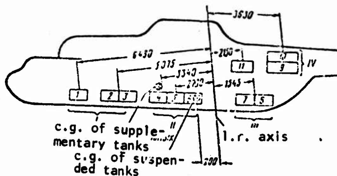
Figure 90. Diagram of Placement of Fuel Tanks on Mi-6 Helicopter.
