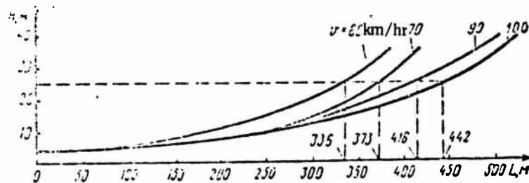
Figure 58. Flying Distance with Vertical Takeoff of Mi-6 Helicopter as a Function of Climbing Speed at Altitude 25 m: G_{\text{av}} = 38,500 \text{ kg} ; UPRT reading--85%; n_{1r} = 83\% ; W = 2-3 \text{ m/sec} (head wind); t = 22^{\circ}\text{C} ; P_{\text{H}} = 742 \text{ mm Hg} .
