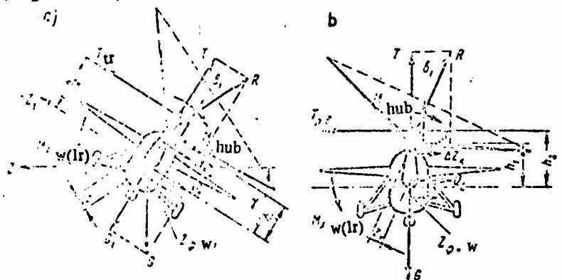
Figure 94. Transverse Balancing of the Mi-6 Helicopter.
