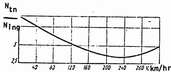
Figure 41. Engine Power Losses in the Tail Rotor.
