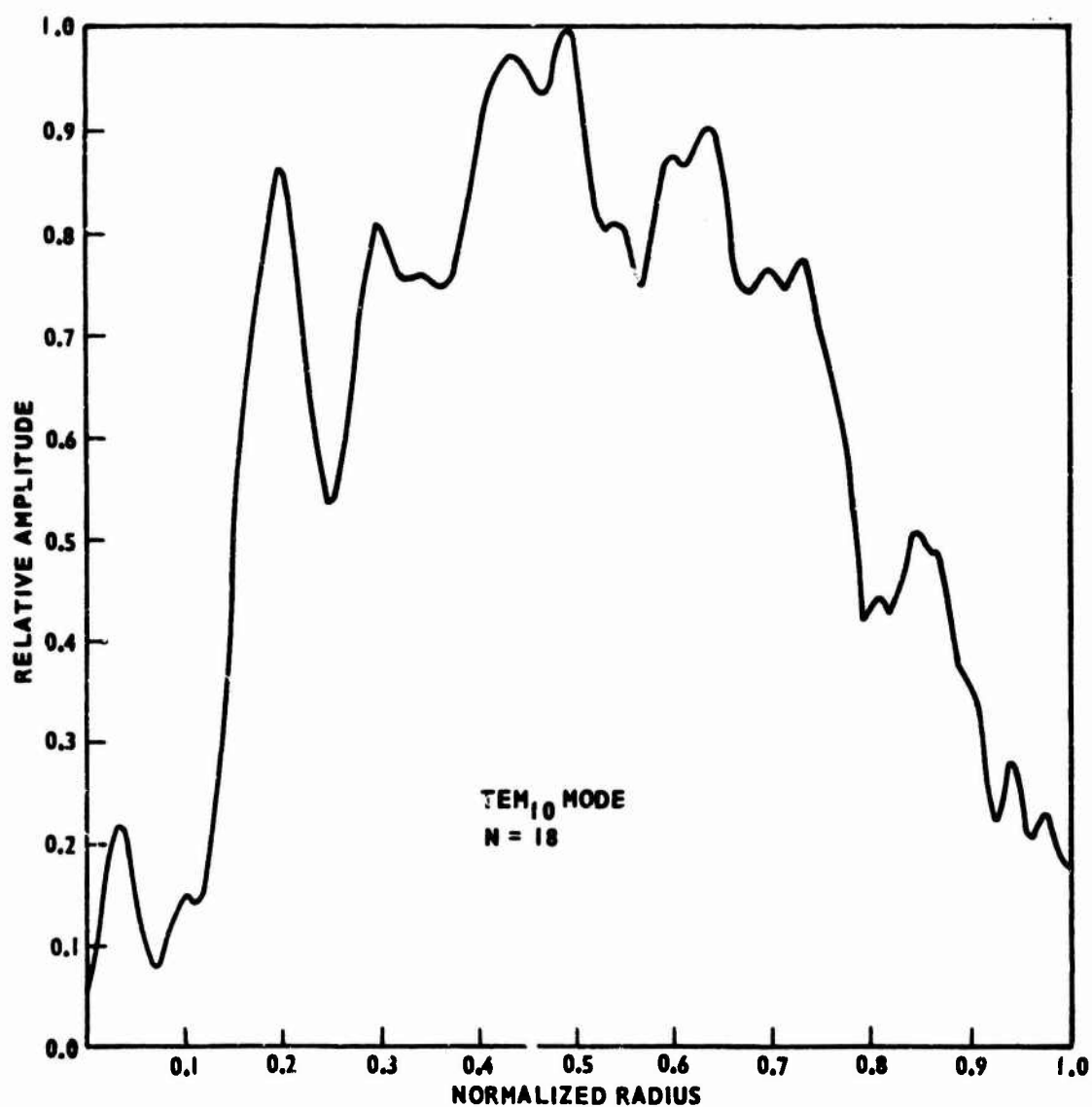
Figure 22. Relative Amplitude of the TEM 10 Mode on the Input Mirror; Resonator Fresnel Number = 18, Output Mirror Zoned, Reflectivity of Transmission Zones = 0.500 (13 half-period zones, 7 transmission)
