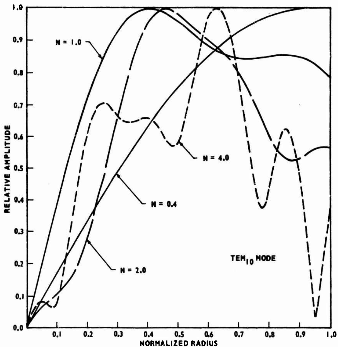
Figure 27. Relative Amplitude of the TEM_{10} Mode on the Input Mirror for Various Values of Resonator Fresnel Number; Output Mirror Divided into 13 Half-Period Zones, 7 Transmission
