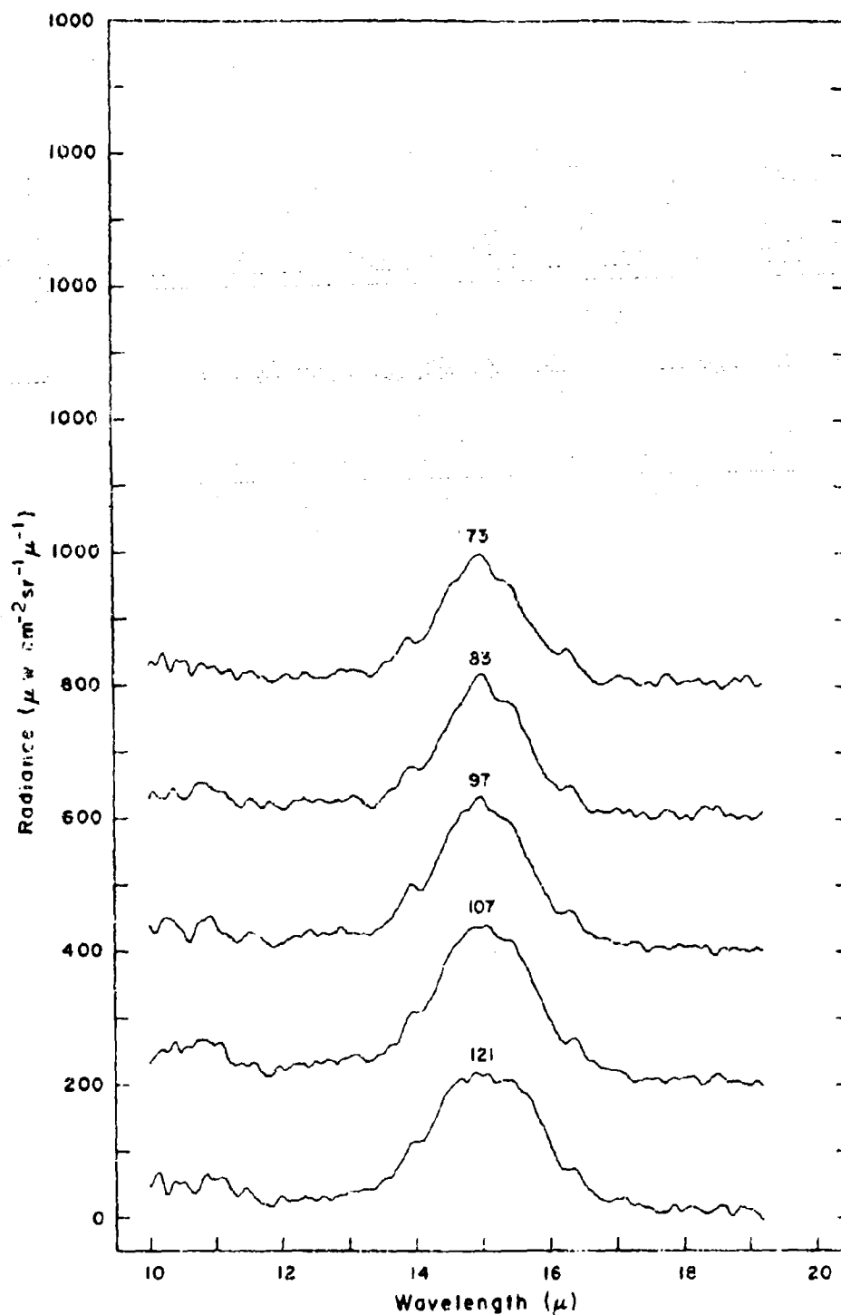
Figure 119 Spectral radiance vs. altitude for balloon flight 1114, 23 June 1968. (See Table 111)
