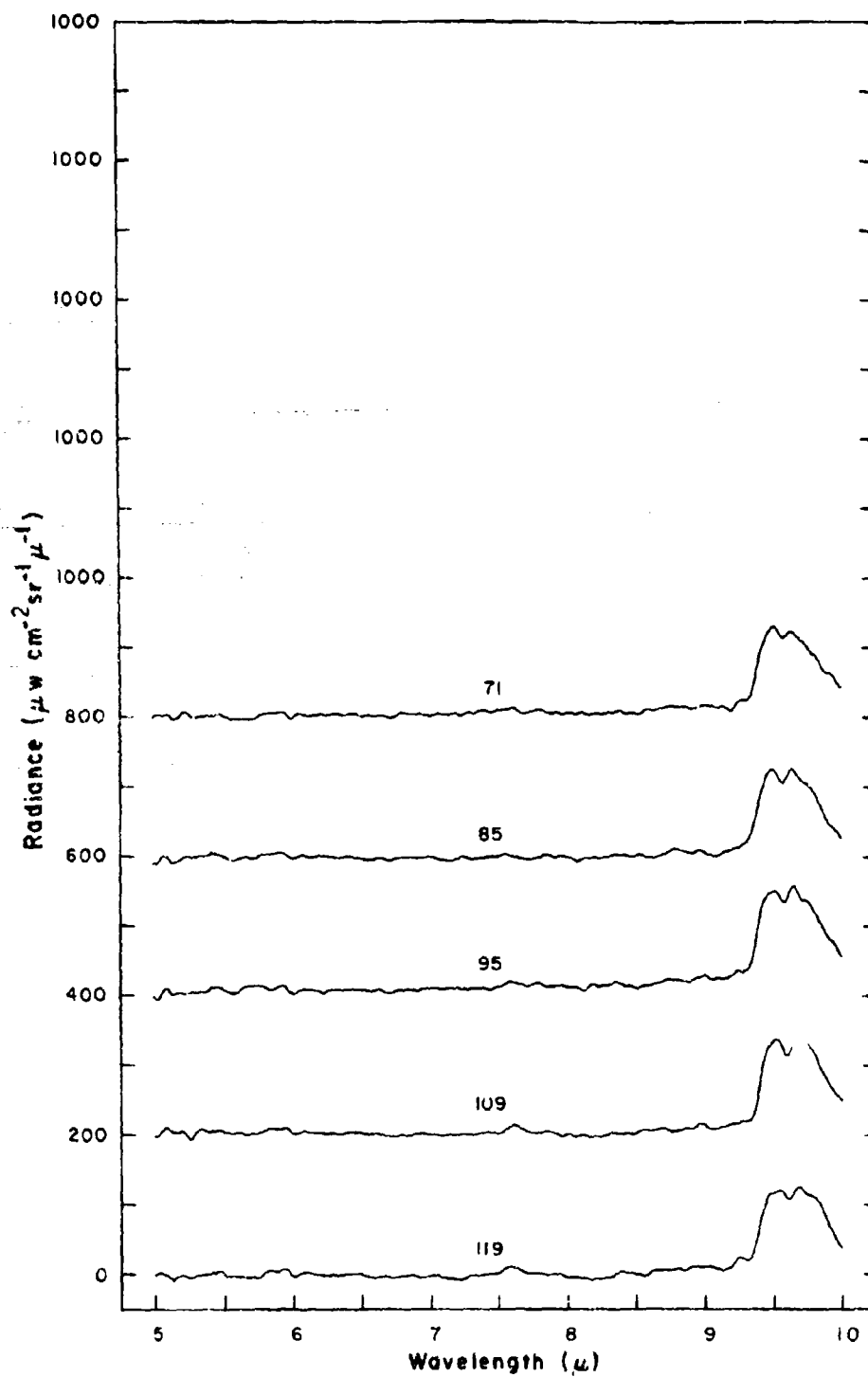
Figure 69 Spectral radiance vs altitude for balloon flight 25 June 1966. (See Table III.)
