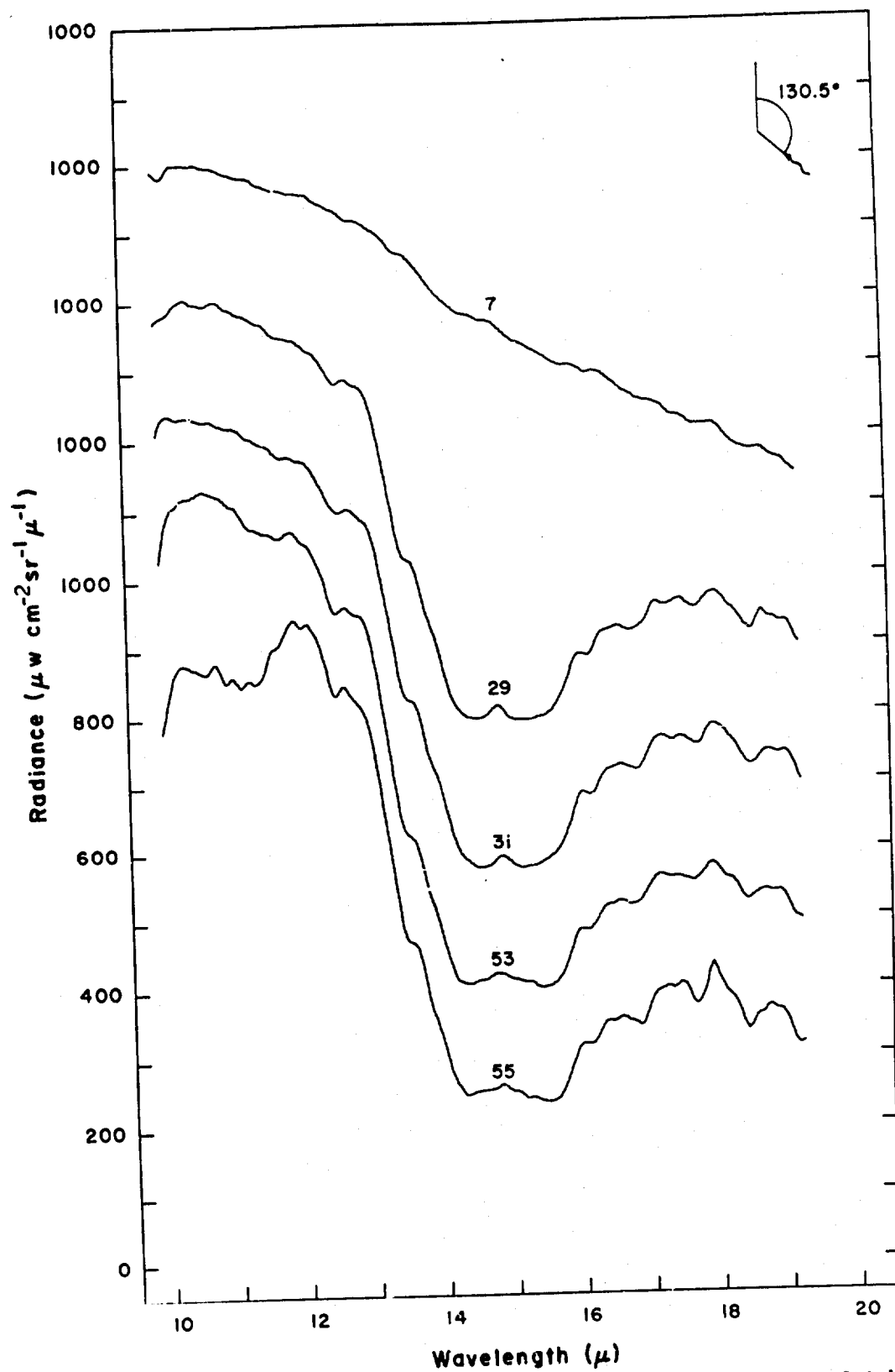
Figure 83 Spectral radiance vs altitude for balloon flight 25 June 1968. (See Table III)
