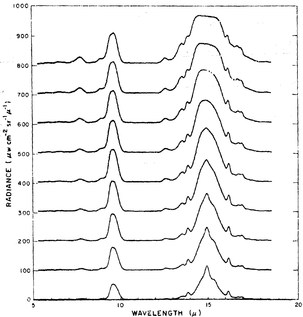
Figure 180. Calculated spectral radiance from 5 to 18 \mu vs altitude for 2 km intervals from 16 to 32 km (top to bottom) at a zenith observation angle of 82.0° (sec = 8) for 30 November 1967. Successive records have a 100 \mu\text{W cm}^{-2} \text{sr}^{-1} \mu^{-1} offset for clarity.
