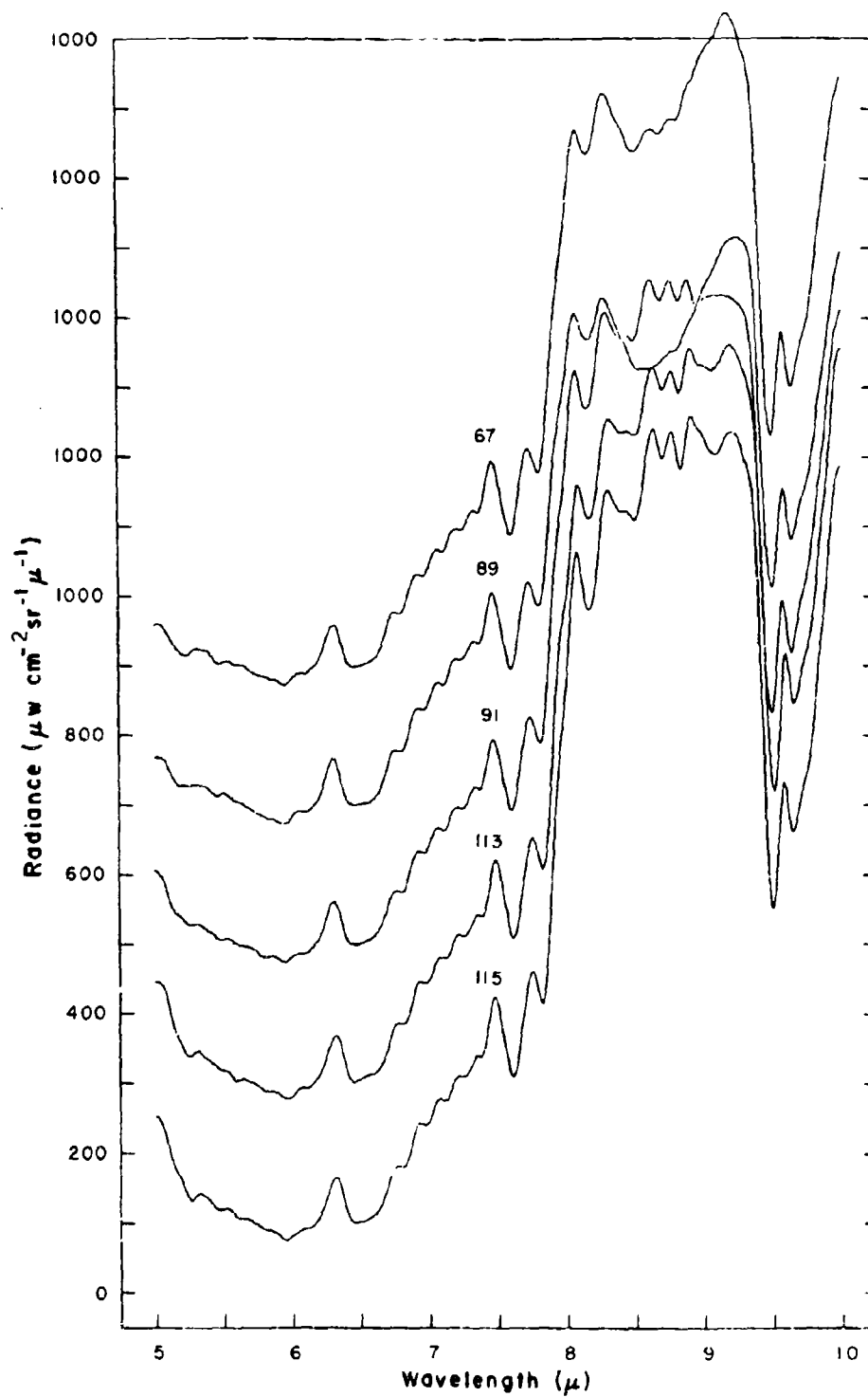
Figure 61 Spectral radiance vs. altitude for balloon flight 25 June 1968. (See Table 111)
