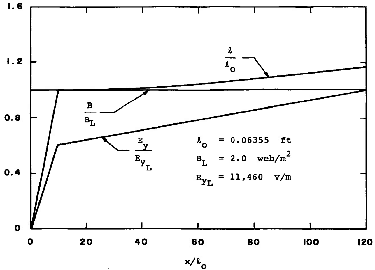
Fig. 4 Streamwise Variation of Channel Flow Parameters using Physically Realistic Recombination Rate and Energy-Loss Factor
