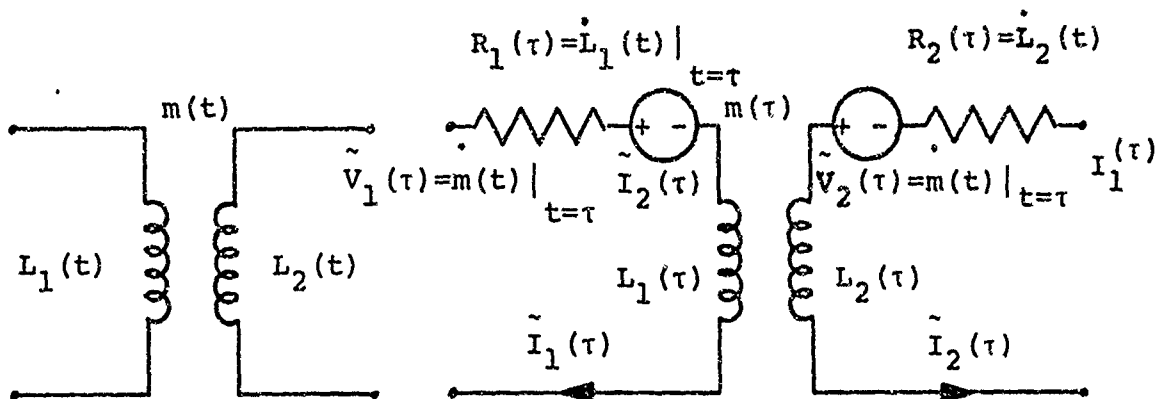
Figure 3: Adjoint Transformation of Time Varying Elements a) Capacitor b) Inductor c) Coupled Inductors
