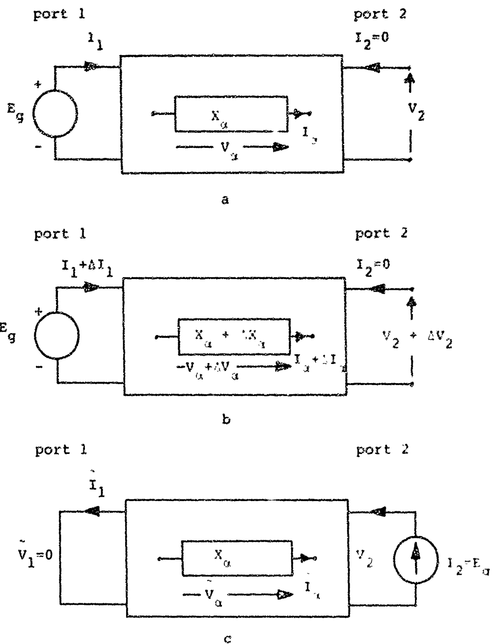
Figure 6: Reciprocal Two Port Networks a) Original Network, N b) Augmented Original Network c) Mutual Reciprocal Adjoint Network, N
