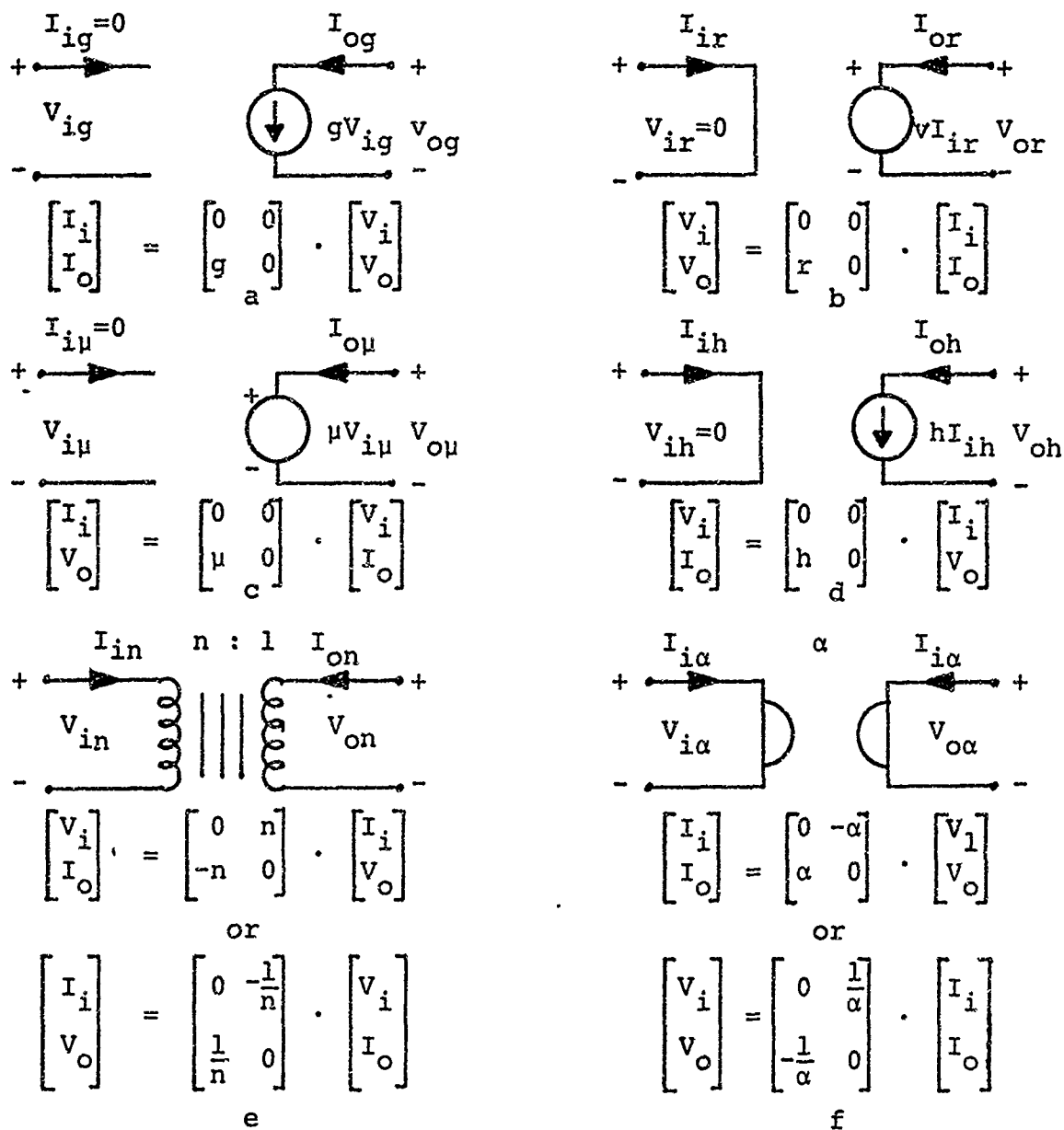
Figure 1: Two-Port Elements and their Matrix Characterization a) Voltage Dependent Current Source b) Current Dependent Voltage Source c) Voltage Dependent Voltage Source d) Current Dependent Current Source e) Ideal Transformer f) Gyrator
