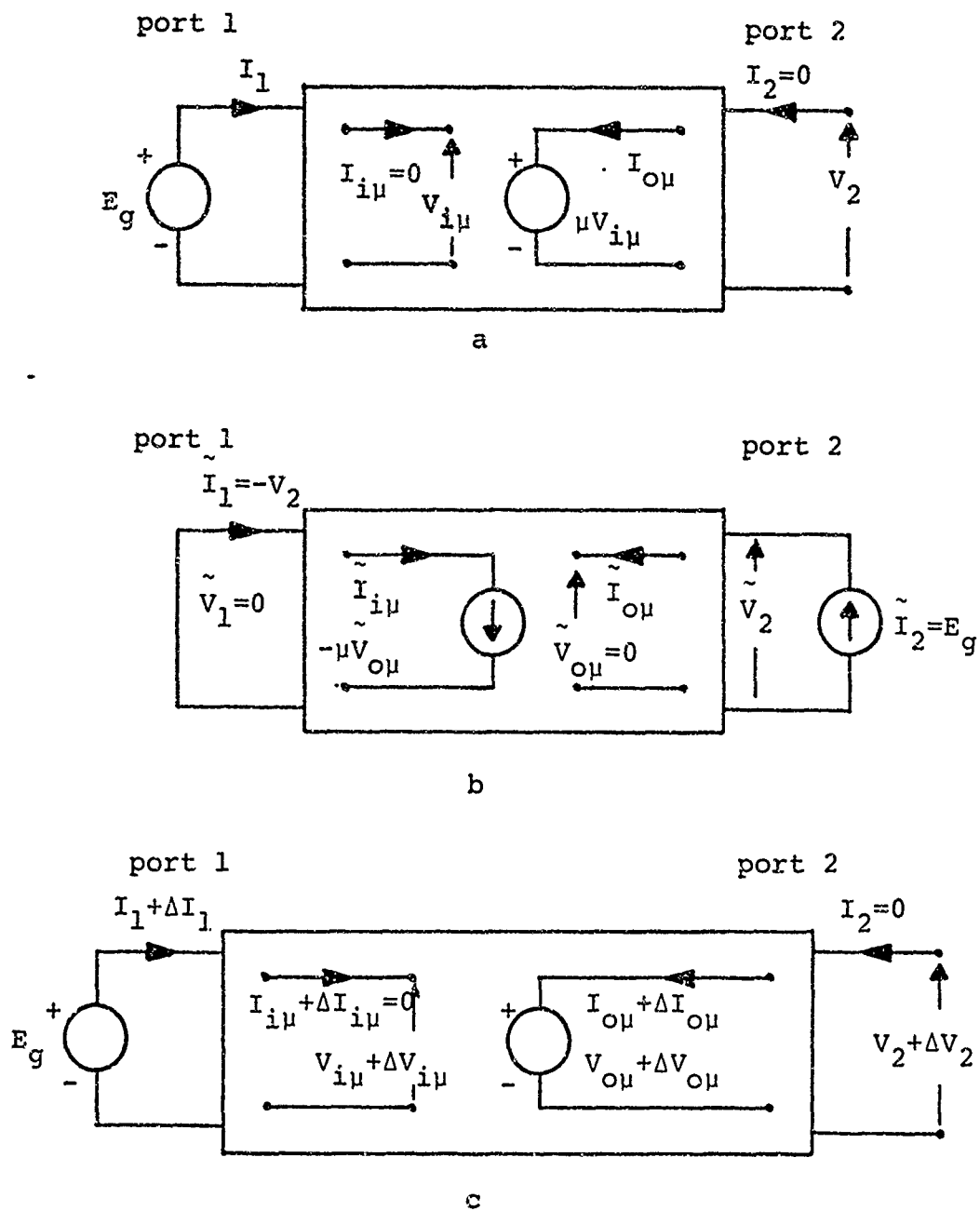
Figure 7: Reciprocal Two Port Networks Containing Voltage Dependent Voltage Sources a) Original Network, N b) Mutual Reciprocal Adjoint Network, \tilde{N} c) Augmented Original Network
