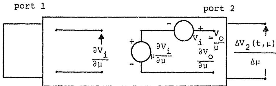
Figure 9: Sensitivity Models Derived by Application of Tellegen's Theorem and the Mutual Reciprocal Adjoint Network a) For One-Port Passive Parameters b) Voltage Dependent Voltage Source
