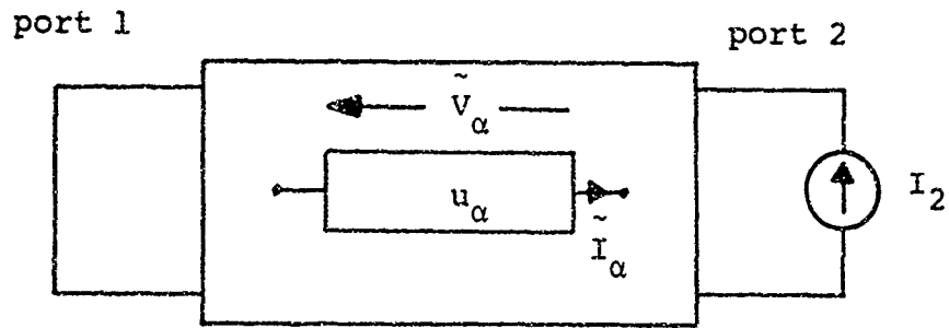
Figure 8: General Interreciprocal Network
