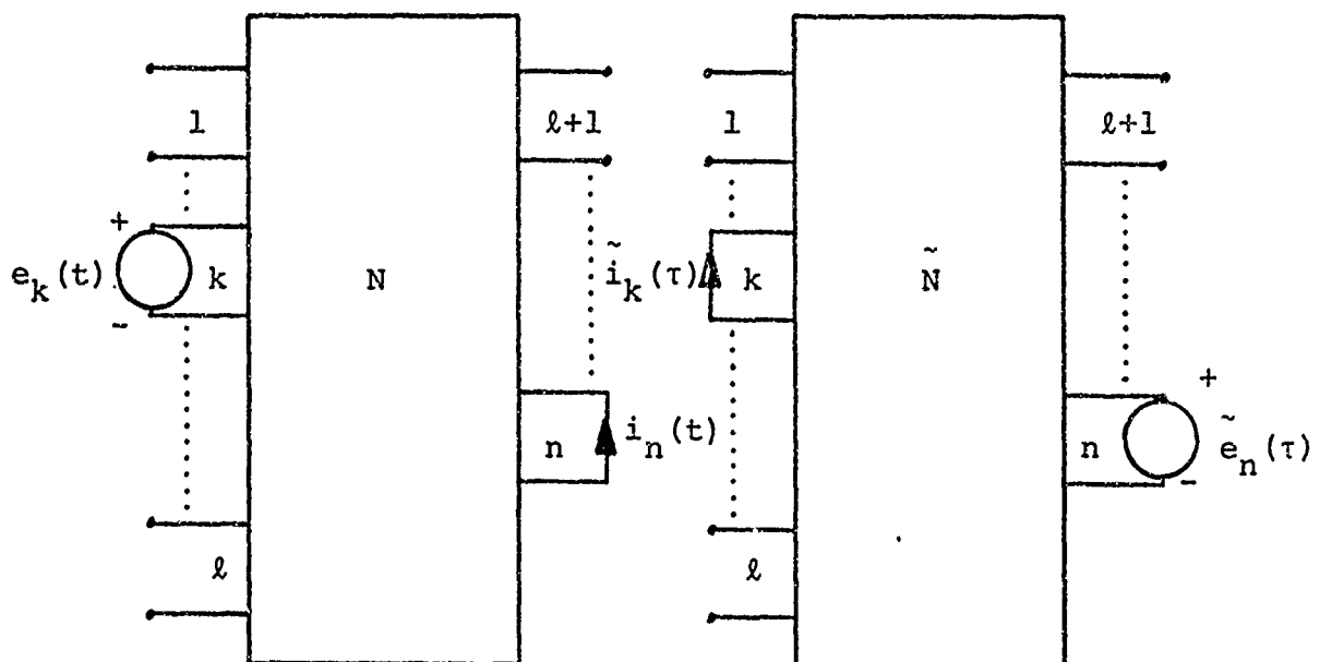
Figure 5: Original Network N and its Adjoint \tilde{N} excited in Reciprocal Manner. Time Domain Case
