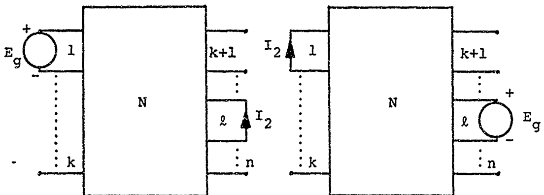
Figure 4: Multiple port Network with Reciprocal Excitation
