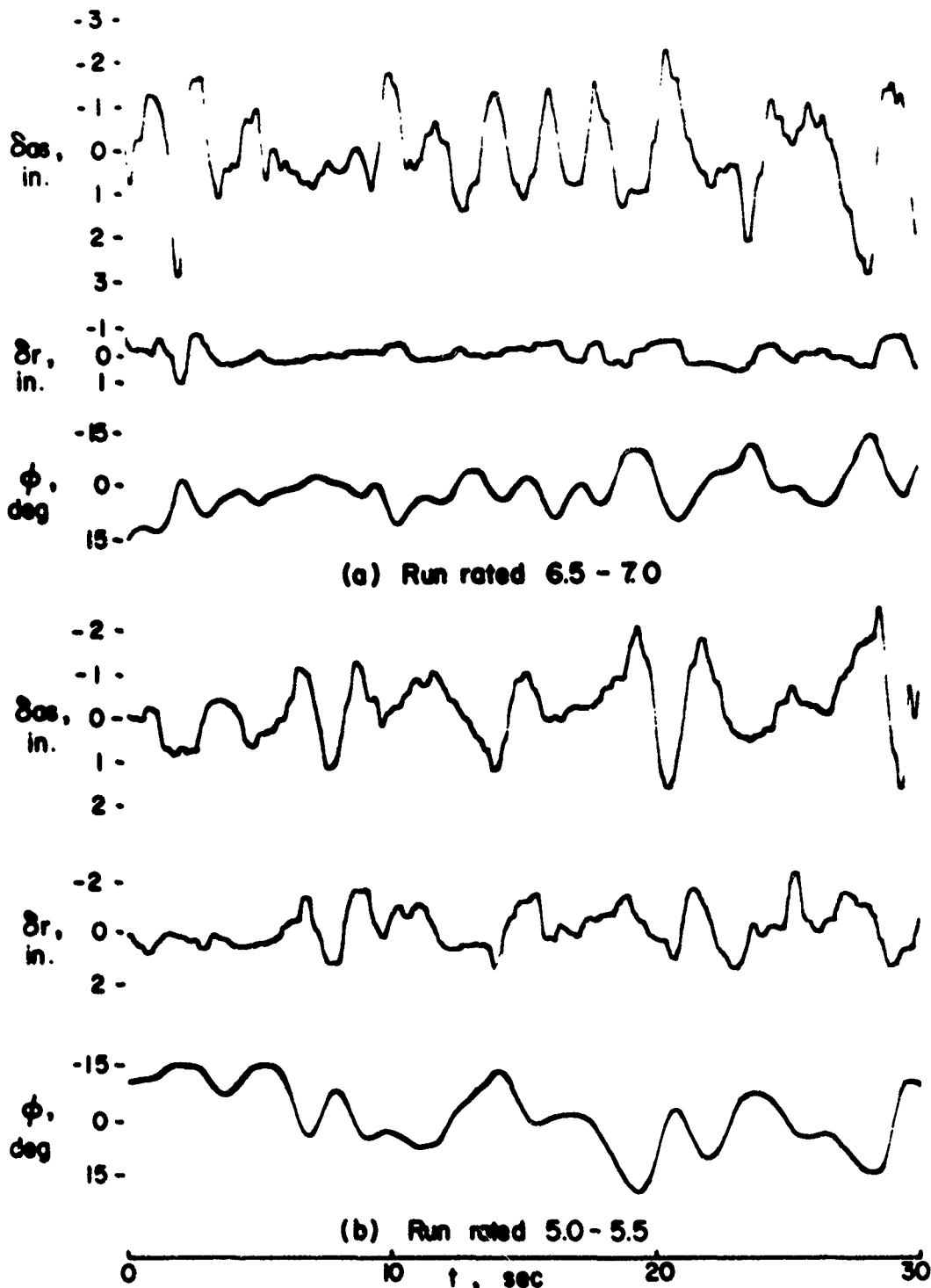
FIGURE III - 13 EFFECTS OF COMBINED LOW ROLL SENSITIVITY AND LOW ROLL DAMPING, \delta_{os} , \delta_r AND \phi VS TIME
