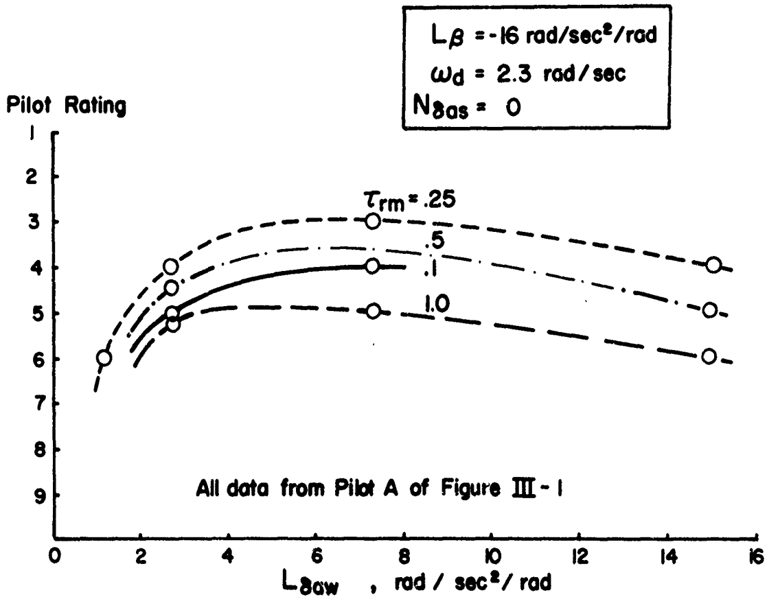
FIGURE III - 2 PILOT RATING AS A FUNCTION OF ROLL SENSITIVITY, L_{\delta ow} . WHEEL CONTROL.
