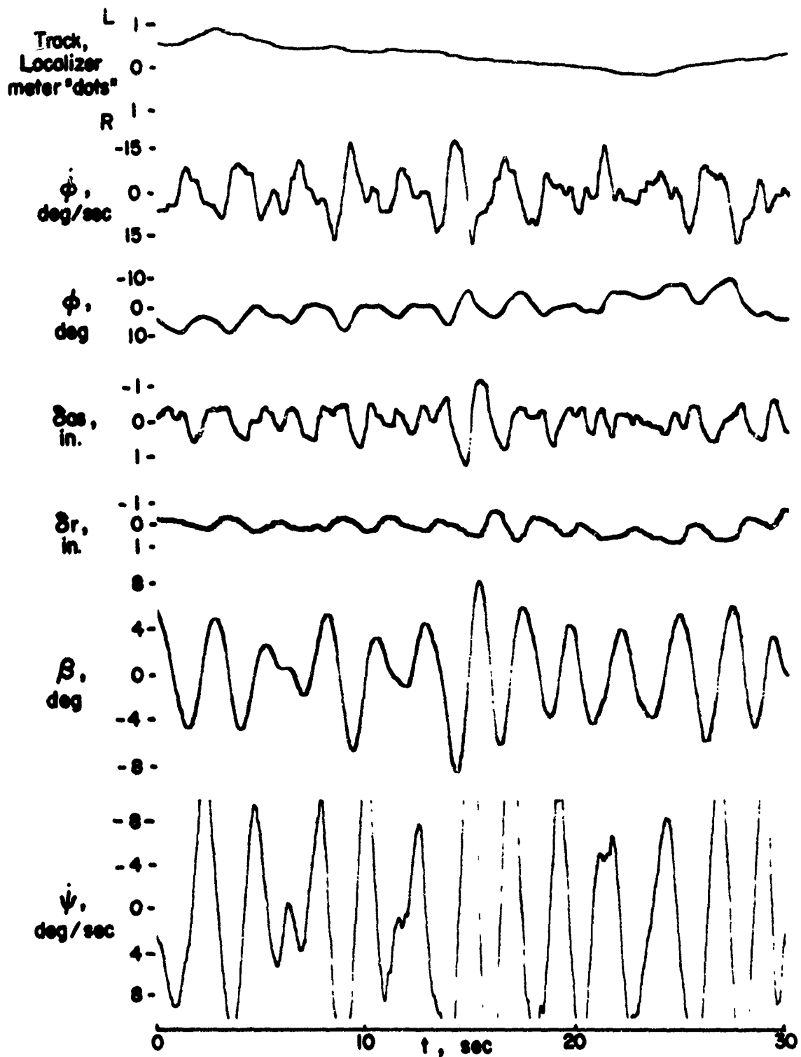
FIGURE IX-7a EFFECTS OF LARGE + N_{B0} , \omega_d = 2.3 RAD/SEC
