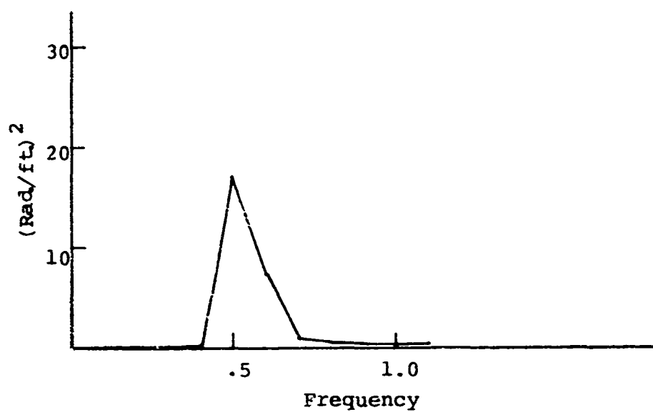
FIGURE 28. Pitch Transfer Functions by Newman's Theory
