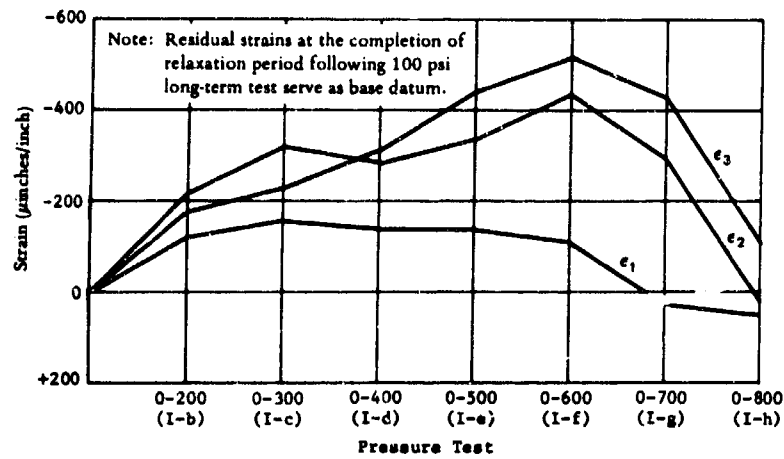
Figure 22b. Residual strains on the interior surface of steel bottom plate flange; Rosette 4B under short-term loading to 800 psi.
