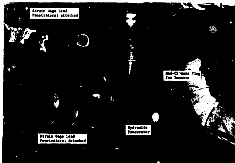
Figure 12. Pressure vessel head plug for accommodating electrical and hydraulic penetrators during hydrostatic testing of NEMO.
