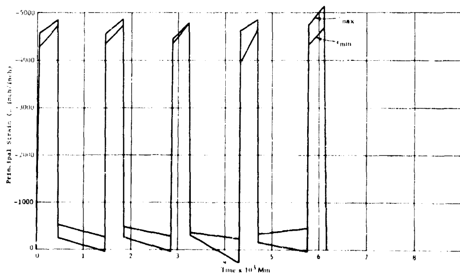
Figure 25b. Cyclic strains on the interior surface of the acrylic hull in equatorial region; Rosette 10B under pressure cycles of 500 psi magnitude and 6-hour duration.
