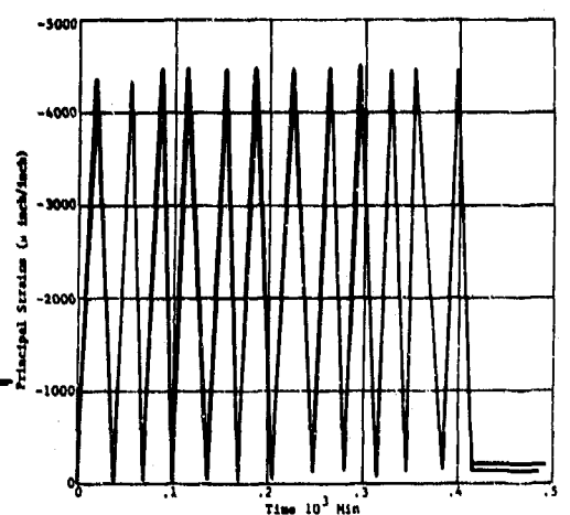
Figure 31d. Comparison of maximum and minimum strains for cycles 1 and 12 on the interior surface of the acrylic hull in equatorial region; Rosette 10B under pressure cycles of 500 psi magnitude and 2-minute duration.
