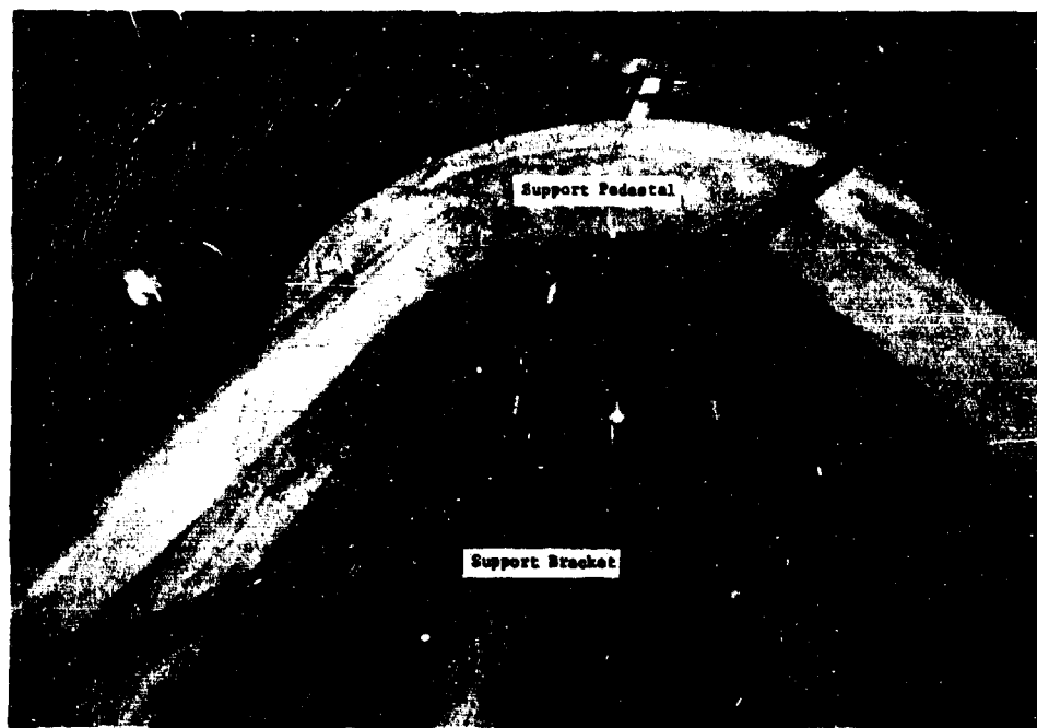
Figure 11. An exterior view of the bottom steel plate showing the support pedestal as well as the penetrators and cables for strain gages located on the interior of the capsule.
