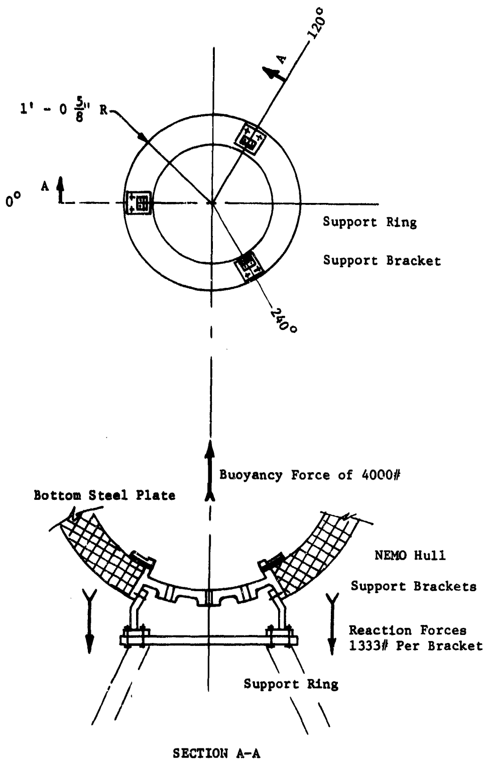
Figure 5. Method of attaching capsule's bottom steel plate to cage support pedestal.
