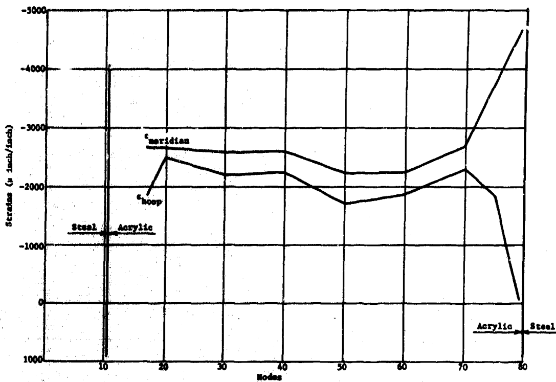
Figure 32a. Distribution of hoop and meridional strains on the exterior surface of acrylic hull at the midpoint of the second 2-minute pressure cycle at 500 psi.
