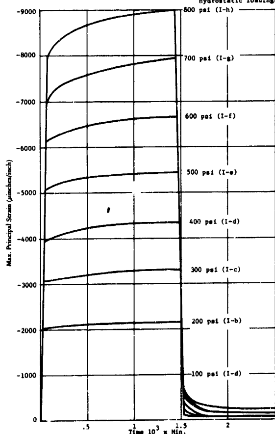
Figure 23b. Time dependent strain on the interior surface of the acrylic hull in the equatorial region; Rosette 12B under long-term hydrostatic loadings to different pressures.
