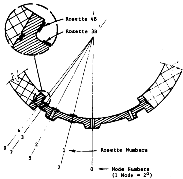
Figure 7. Location of and numbering system for rosettes on the stainless steel plate portion of the capsule.
