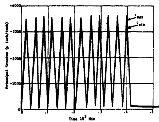
Figure 31c. Comparison of maximum and minimum strains for cycles 1 and 12 on the exterior surface of the acrylic hull in equatorial region; Rosette 10A under pressure cycles of 500 psi magnitude and 2-minute duration.
