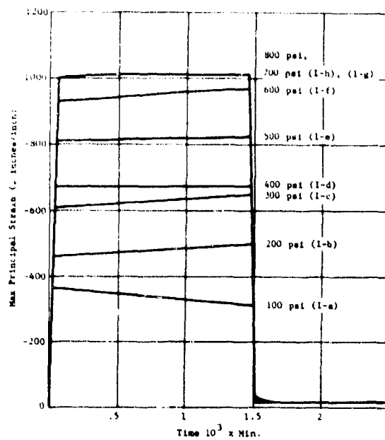
Figure 2a. Time dependent strain on the internal surface of the bottom steel plate; Rosette 3B under long-term hydrostatic loadings to different pressures.
