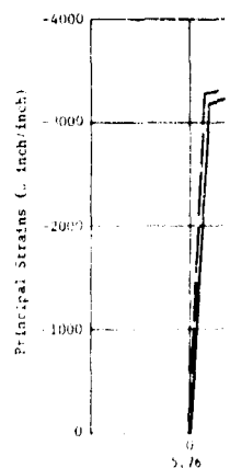
Figure 25d. Cyclic strains on the interior surface of the acrylic hull in equatorial region; Rosette 10C under pressure cycles of 500 psi magnitude and 6-hour duration.
