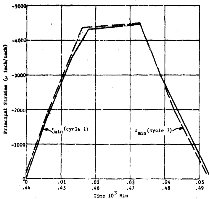
Figure 29e. Comparison of minimum strains for cycles 1 and 7 on the interior surface of the acrylic hull in equatorial region; Rosette 10B under pressure cycles of 500 psi magnitude and 15-minute duration.
