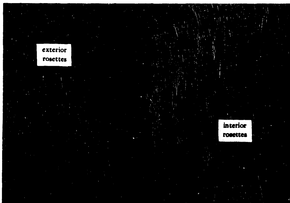
Figure 8. Typical installation of strain gage rosettes on the interior and exterior surfaces of the acrylic hull.
