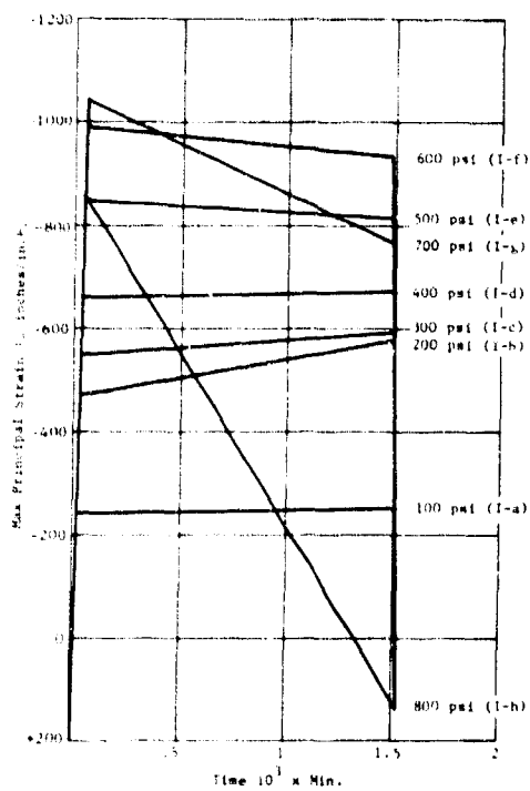
Figure 2b. Time dependent strain on the internal surface of the bottom steel plate (flange); Rosette 4B under long-term hydrostatic loadings to different pressures.
