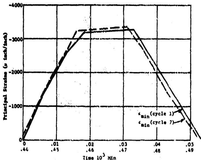
Figure 29c. Comparison of maximum and minimum strains for cycles 1 and 7 on the exterior surface of the acrylic hull in equatorial region; Rosette 10A under pressure cycles of 500 psi magnitude and 15-minute duration.
