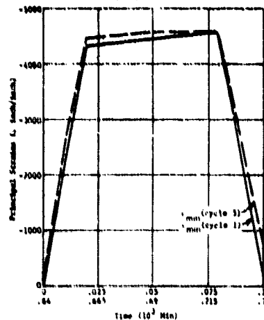
Figure 27d. Comparison of maximum and minimum strains for cycles 1 and 3 on the interior surface of the acrylic hull in equatorial region; Runette 10B under pressure cycles of 500 psi magnitude and 1-hour duration.
