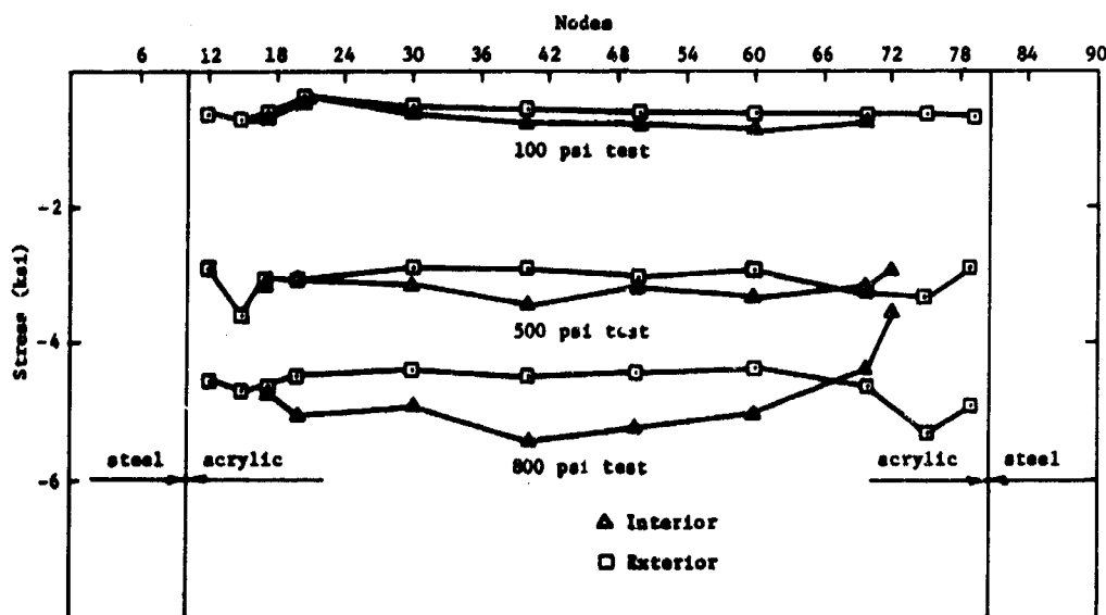
Figure 15b. Distribution of Meridional Stresses on the NEMO acrylic hull.
