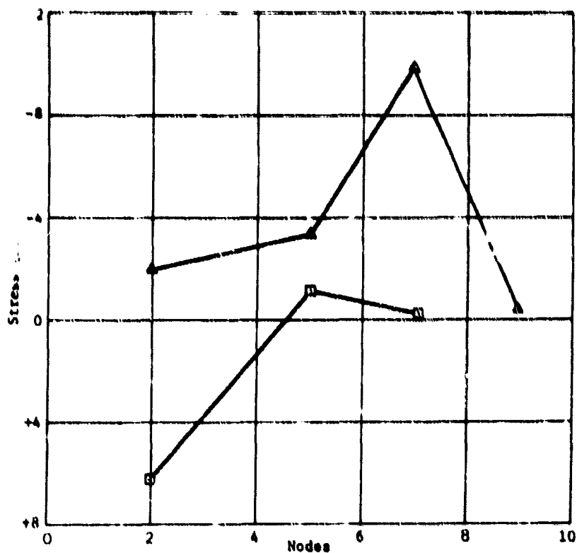
Figure 1b. Meridional Stresses on Bottom Steel Plate Under 100 psi Hydrostatic Loading.
