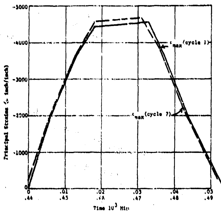
Figure 29d. Comparison of maximum strains for cycles 1 and 7 on the interior surface of the acrylic hull in equatorial region; Rosette 10B under pressure cycles of 500 psi magnitude and 15-minute duration.
