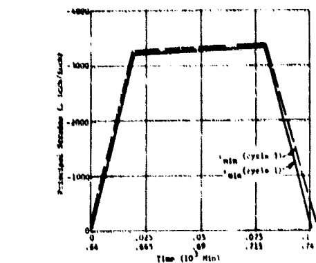
Figure 27a. Comparison of maximum and minimum strains for cycles 1 and 3 on the exterior surface of the acrylic hull in equatorial region; Runette 10A under pressure cycles of 500 psi magnitude and 1-hour duration.
