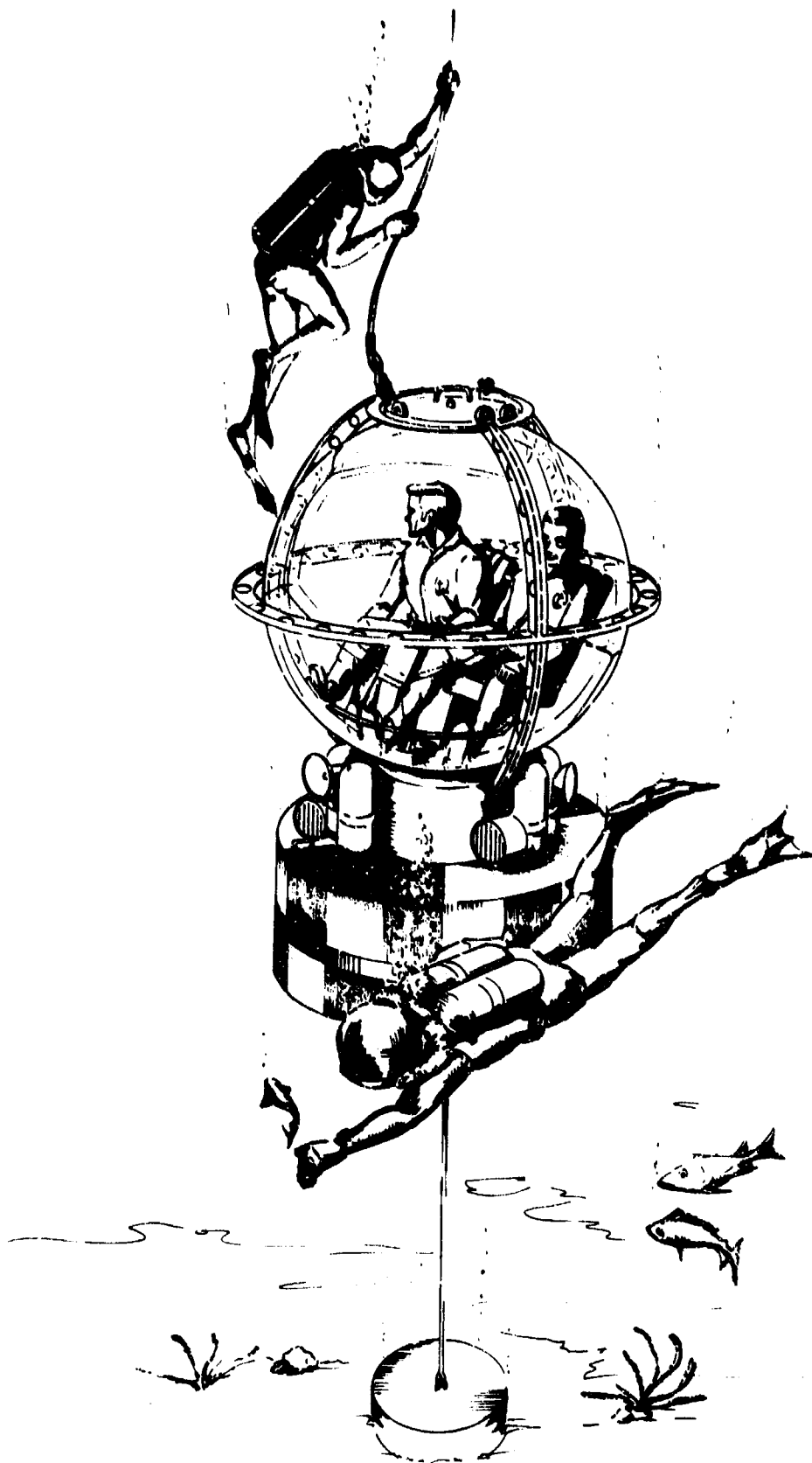
Figure 2. NEMO capsule in tethered self-winch diving control center.
