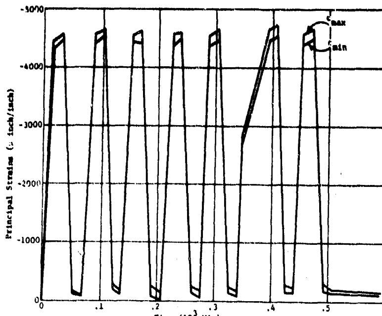
Figure 29b. Cyclic strains on the interior surface of the acrylic hull in equatorial region; Rosette 10B under pressure cycles of 5000 psi magnitude and 15-minute duration.
