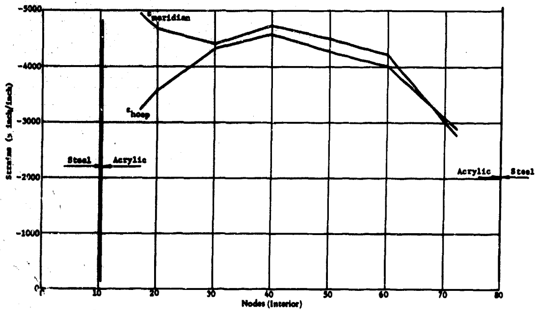
Figure 32b. Distribution of hoop and meridional strains on the interior surface of acrylic hull at the midpoint of the second 2-minute pressure cycle at 500 psi.
