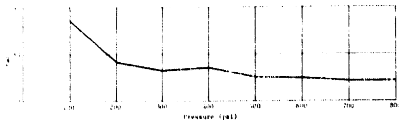
Figure 19d. Change in orientation of principal strains on the exterior surface of the acrylic hull in equatorial region; Rosette 12A under short term loading to 800 psi.
