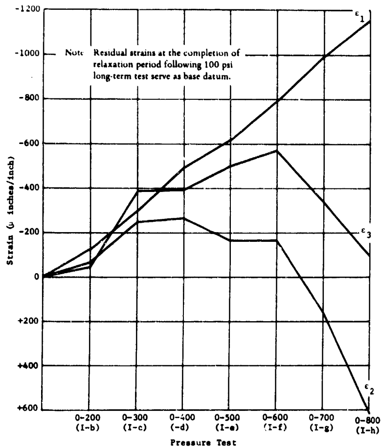
Figure 22a. Residual strains on the interior of bottom steel plate at the conclusion of each long-term test; Rosette 3h.
