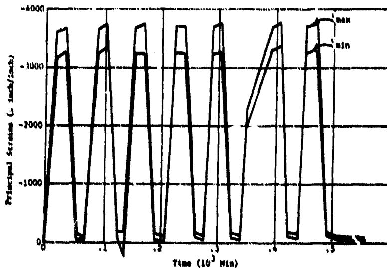
Figure 28a. Cyclic strains on the exterior surface of the acrylic hull in equatorial region; Rosette 10A under pressure cycles of 500 psi magnitude and 15-minute duration.
