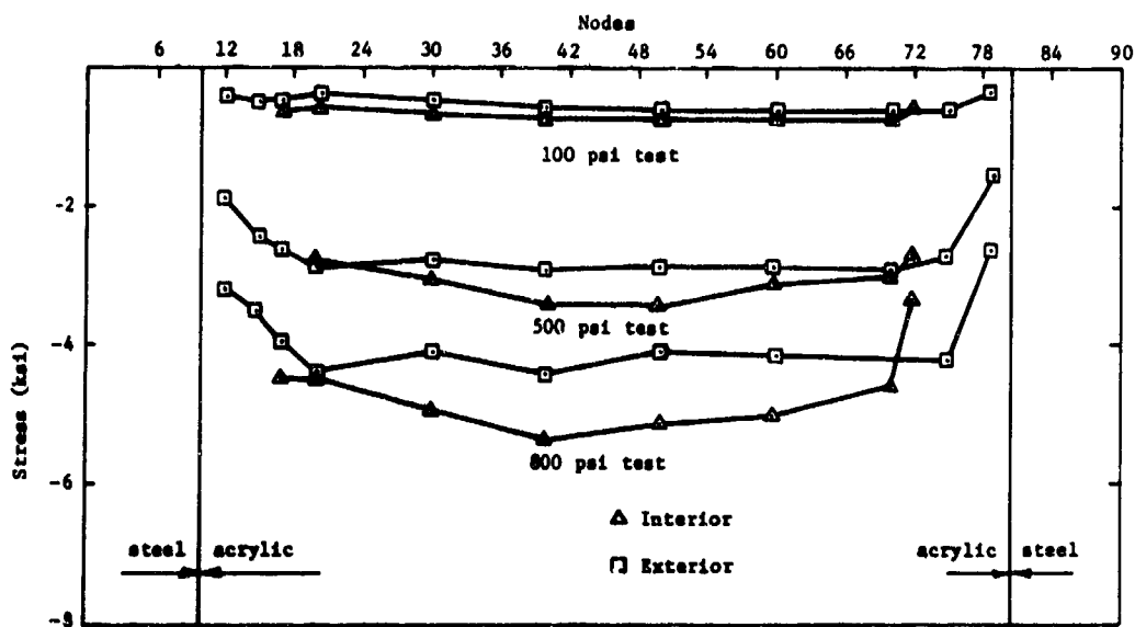
Figure 15a. Distribution of Hoop Stresses on the NEMO acrylic hull.
