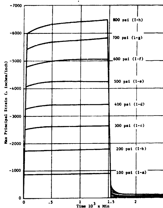
Figure 23a. Time dependent strain on the exterior surface of the acrylic hull in equatorial region; Rosette 12A under long-term hydrostatic loadings to different pressures.
