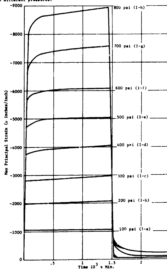
Figure 23c. Time dependent strain on the exterior surface of the acrylic hull near polar penetration; Rosette 18A under long-term hydrostatic loadings to different pressures.
