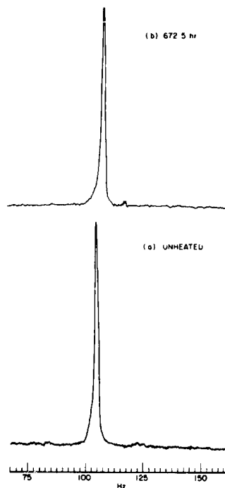
Fig. 1 - Nmr spectra of a degassed 0.20M solution of \text{Na}_2\text{HNTA} sealed under reduced pressure and heated to 200 °C
