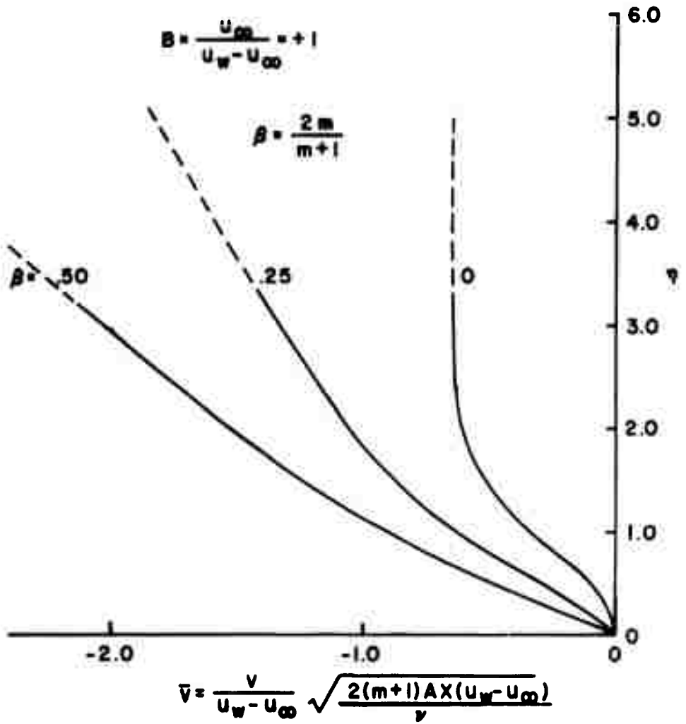
Figure 11. \bar{V} Versus \eta , B = +1 , \beta = 0, .25, .50
