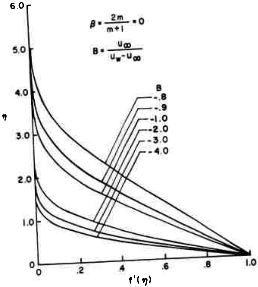
Figure 12. f' Versus \eta , B < -1/2 , B = 0
