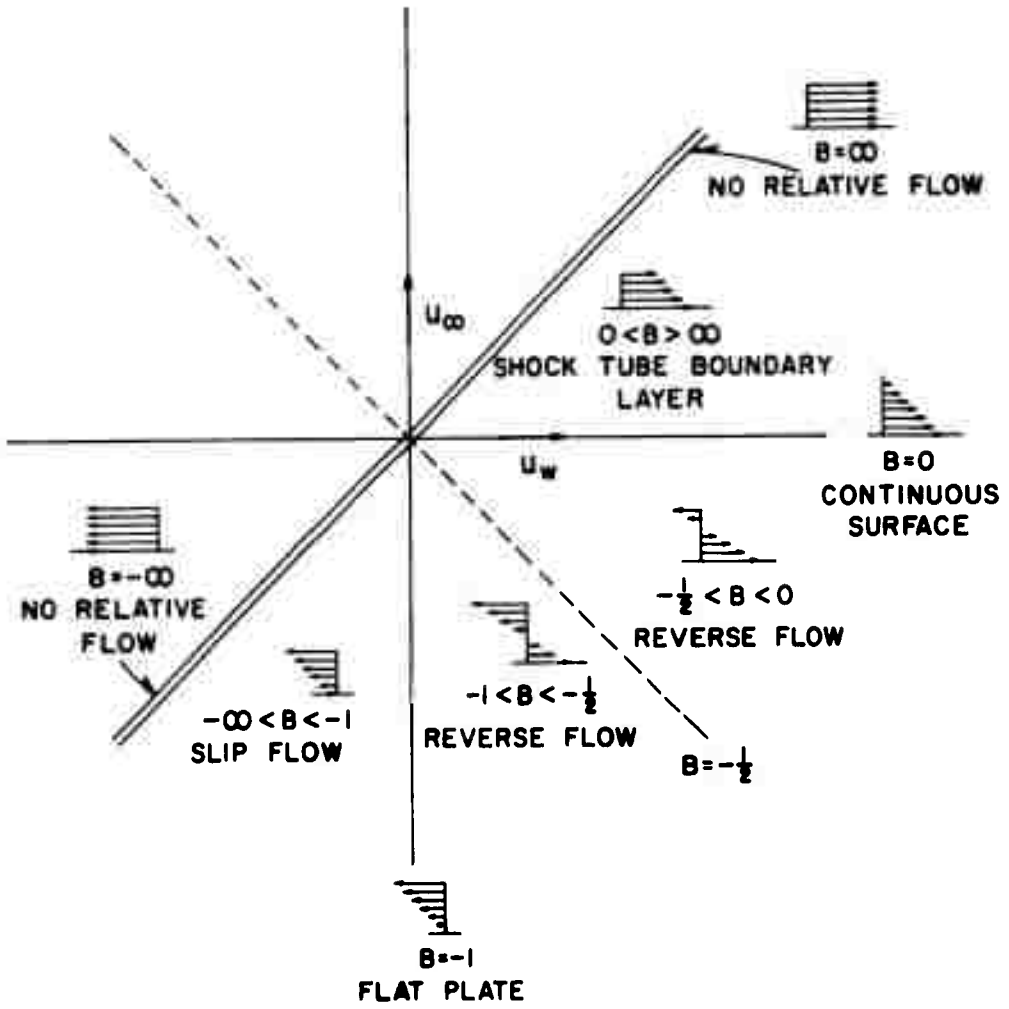
Figure 6. Flows Represented by f'' + \frac{2B+1}{|2B+1|} f'' (f + B\eta) = 0 where B = U_w / (U_w - U_\infty)
