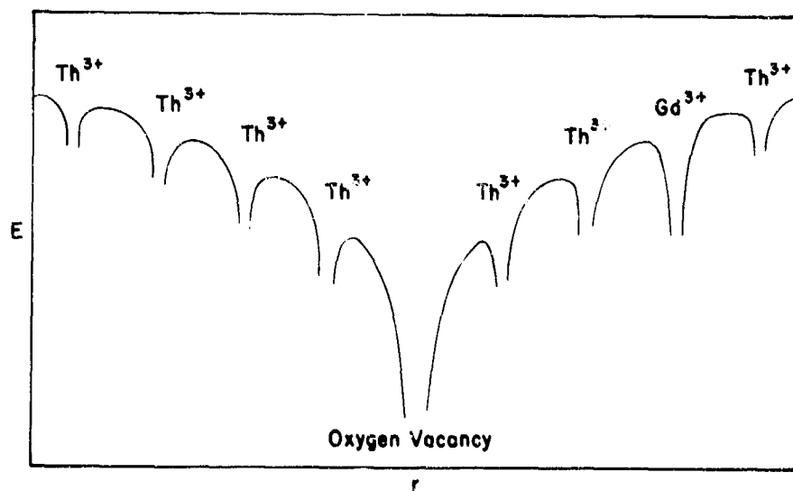
(B) Schematic of Th 3+ Energy Levels in Neighborhood of Oxygen Vacancy
