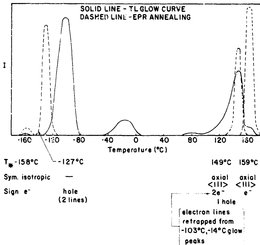
(A) Comparison of TL & EPR Properties
