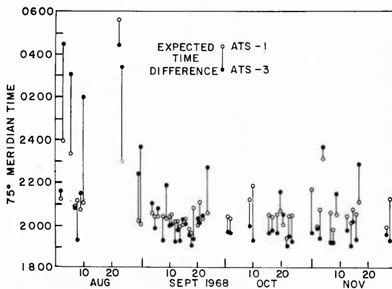
Figure 7. First Appearances of High Amplitude Scintillation ( SI > 60\% ) in ATS-1 and ATS-3 Signals on Different Nights at Huancayo, Peru. Time difference between the 350 subionospheric longitudes was approximately one hour
