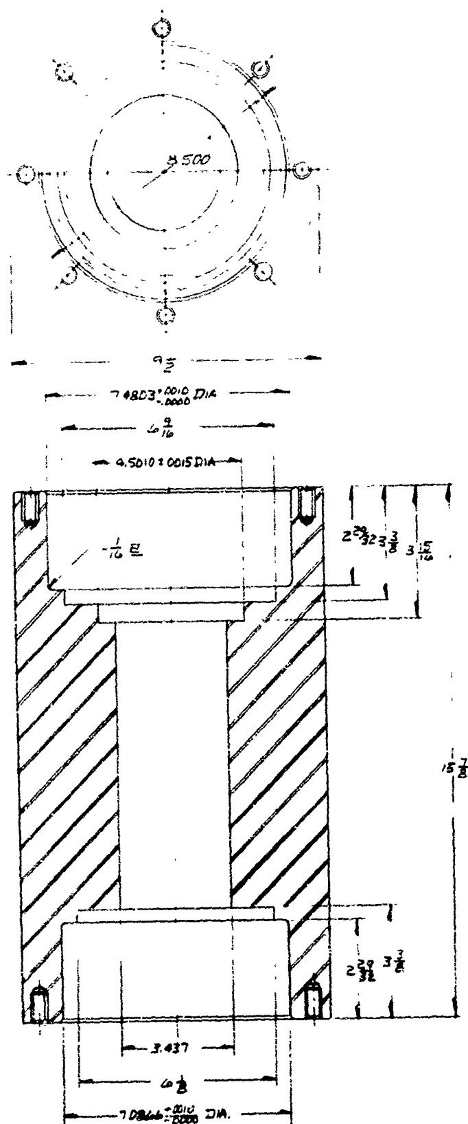
Figure 26. Bearing and Bearing Housing
