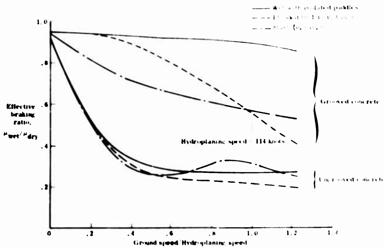
Figure 27.- Effect of runway grooves on aircraft braking performance.
