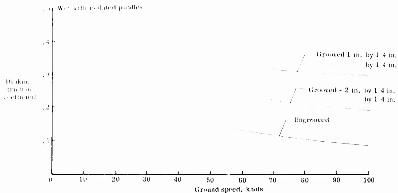
Figure 12.- Effect of runway groove configuration on C-141A aircraft braking on landing research runway at NASA Wallops Station.
