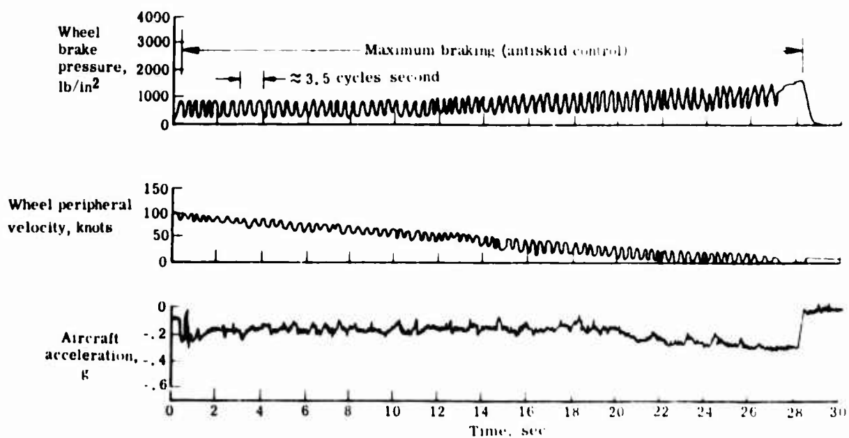
(b) Wet runway condition (low friction). Concrete runway at England AFB.
