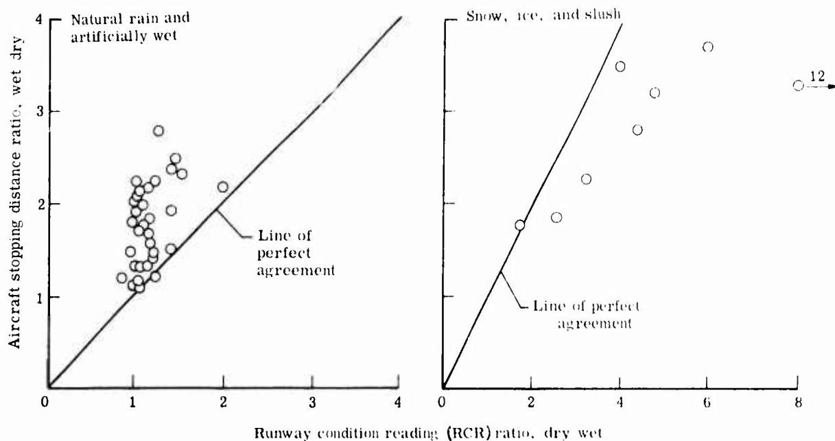
Figure 16.- Correlation between C-141A aircraft and RCR test vehicle.
