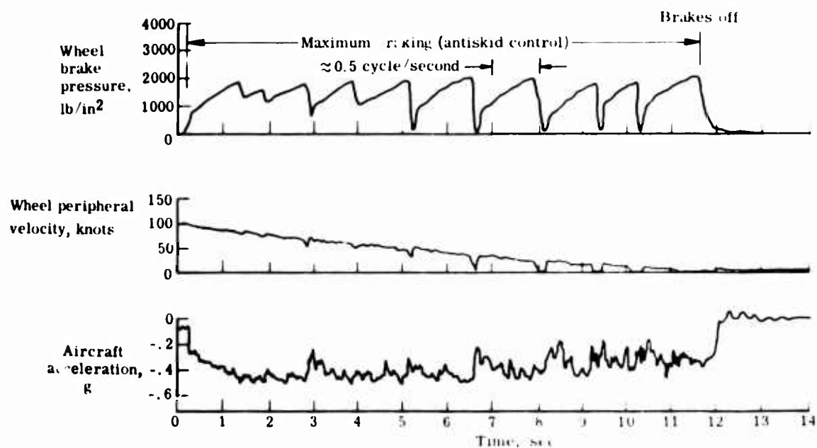
(a) Dry runway condition. Porous friction course at Marham RAFB.
