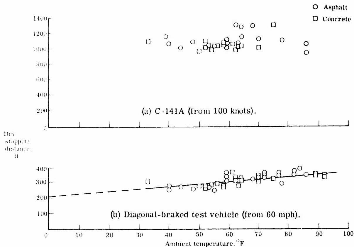
Figure 7. - Effects of runway ambient air temperature on aircraft and test vehicle dry runway stopping distance.
