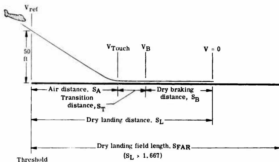
Figure 24.- Aircraft landing terminology.
