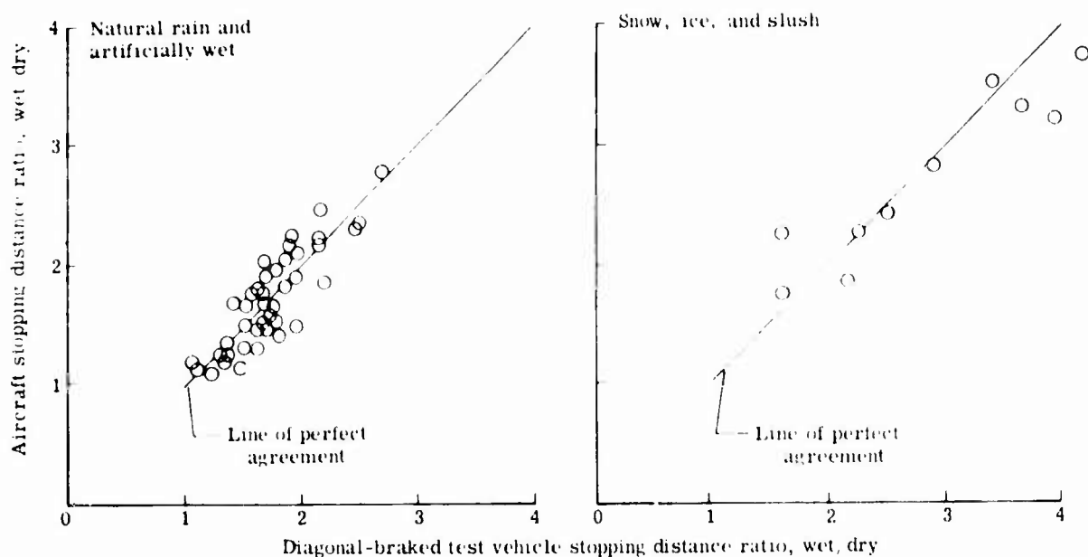
Figure 19.- Correlation between C-141A aircraft and the diagonal-braked test vehicle.
