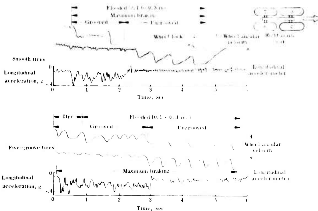
(c) Tread effects (flooded).
