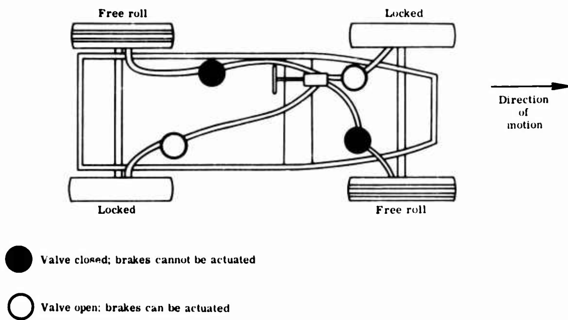
Figure 2.- Braking system for NASA diagonal-braked test vehicle.
