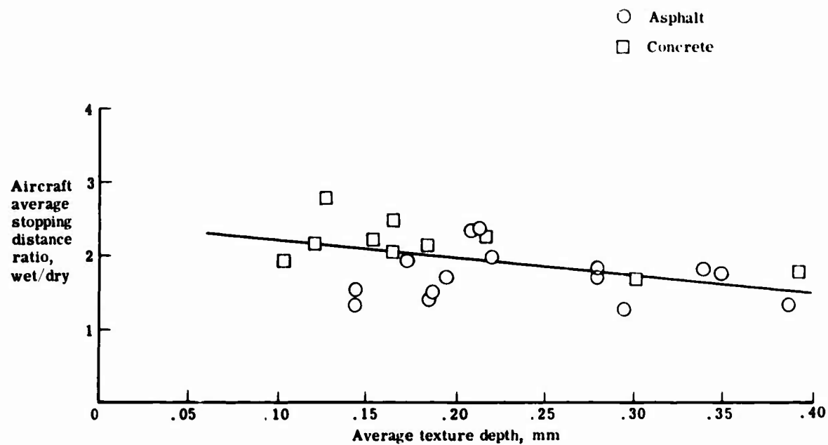
Figure 26.- Variation of aircraft wet-dry stopping distance ratio with runway surface average texture depth (NASA grease test).
