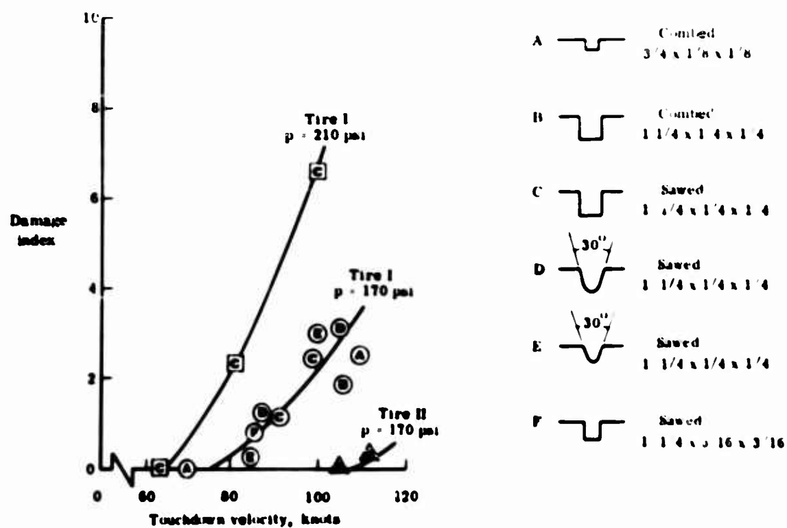
Figure 28.- Tire chevron cutting on grooved surfaces. 49 x 17 tire; vertical velocity, 2.5 ft/sec. Measurements are in inches for runway surfaces unless otherwise noted.
