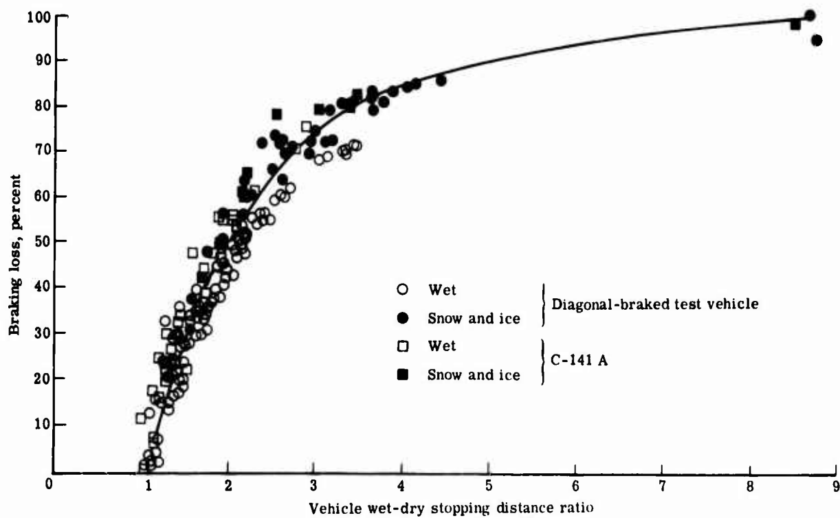
Figure 21. Effect of runway slipperiness on stopping distances and tire traction of C-141A aircraft and NASA diagonal-braked test vehicle.
