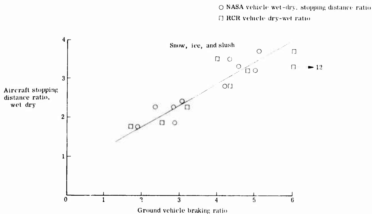
Figure 20.- Correlation between aircraft and ground vehicle braking ratio.
