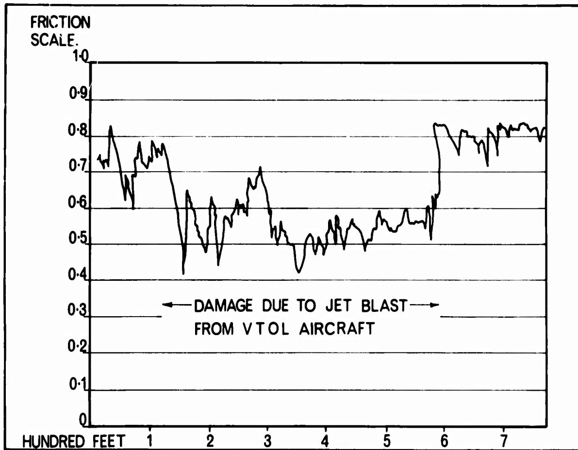
Figure D3.- Friction meter record of runway damage due to jet blast from VTOL aircraft.
