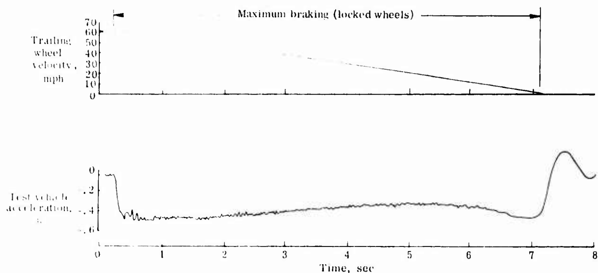
(a) Dry runway condition. Concrete runway at England AFB.
