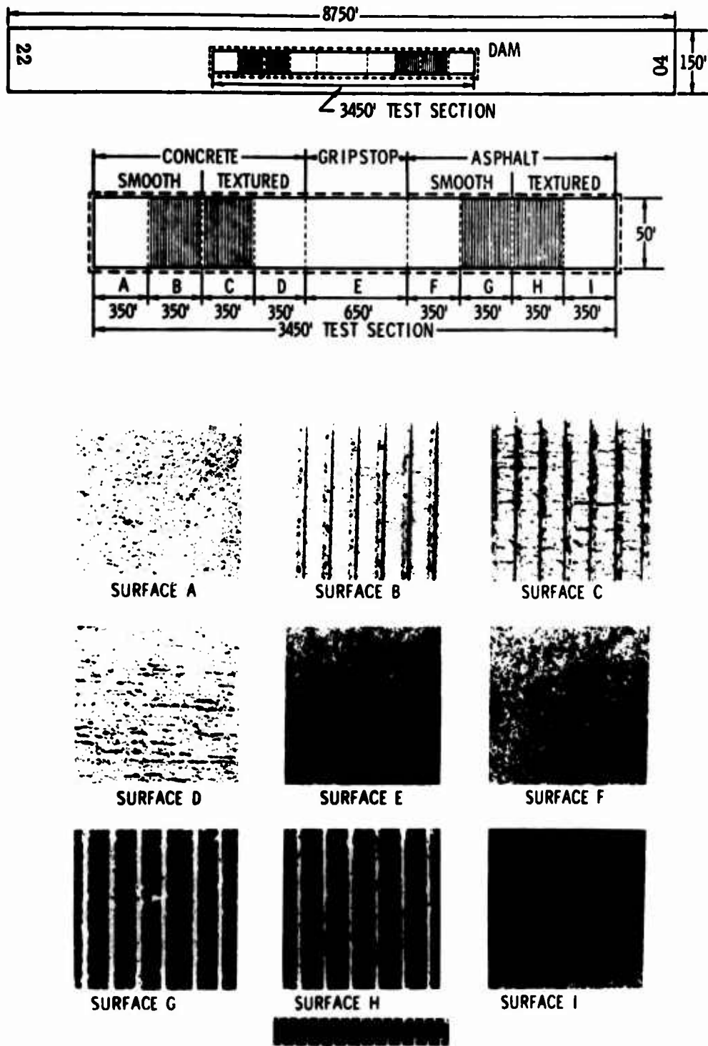
Figure C1.- Landing research runway at Wallops Station, Virginia.
