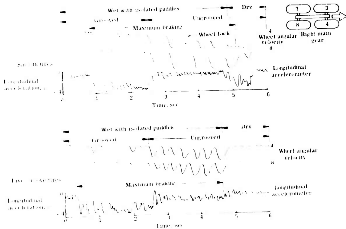
(b) Tread effects (wet).
