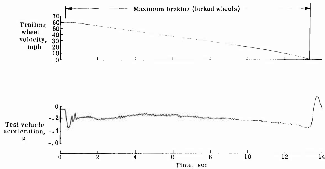
(b) Wet runway condition. Concrete runway at England AFB.
