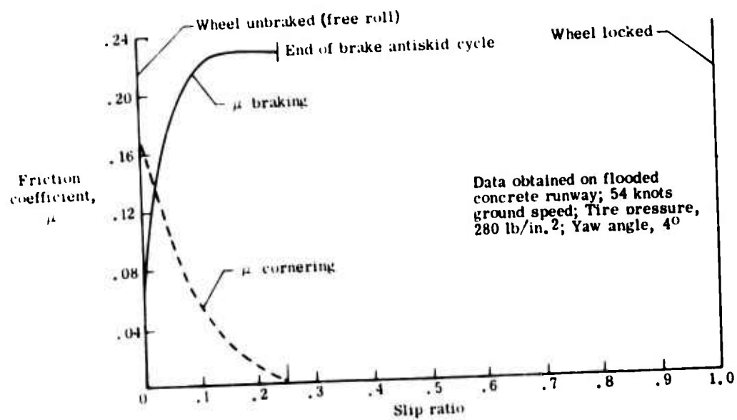
Figure 9.- Loss of cornering friction of main landing gear tire of fighter aircraft.
