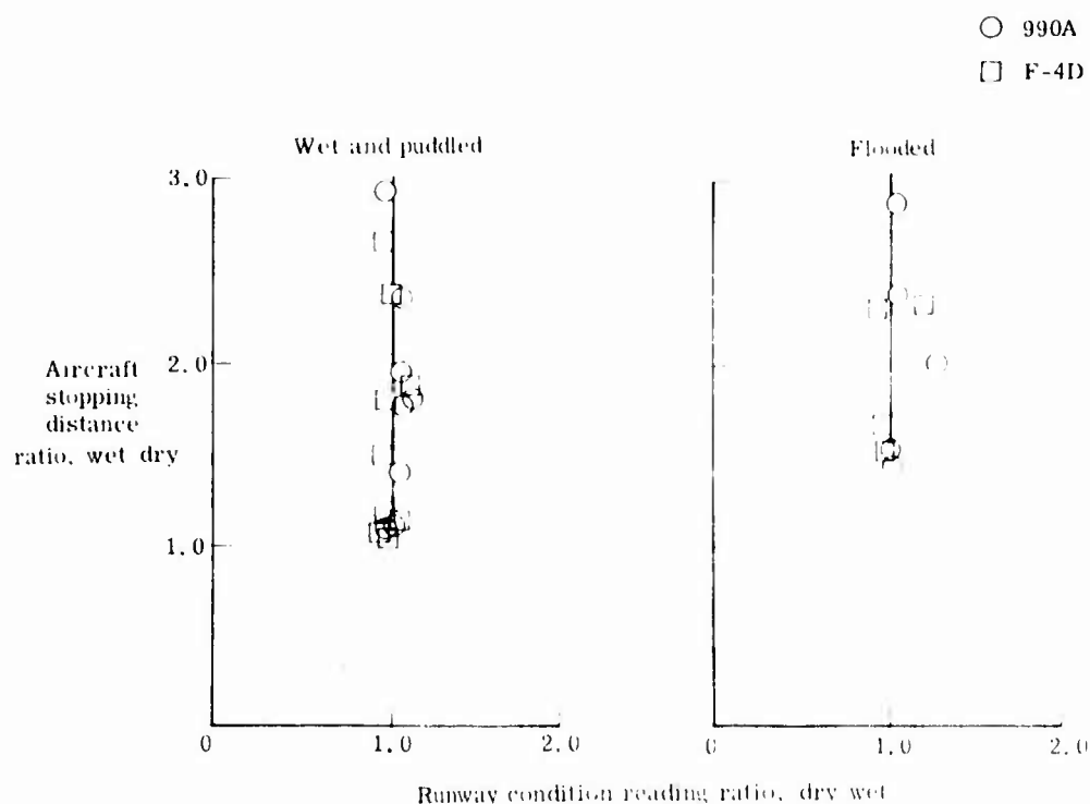
Figure 15.- Comparison of aircraft stopping distance ratios with RCR ratios.
