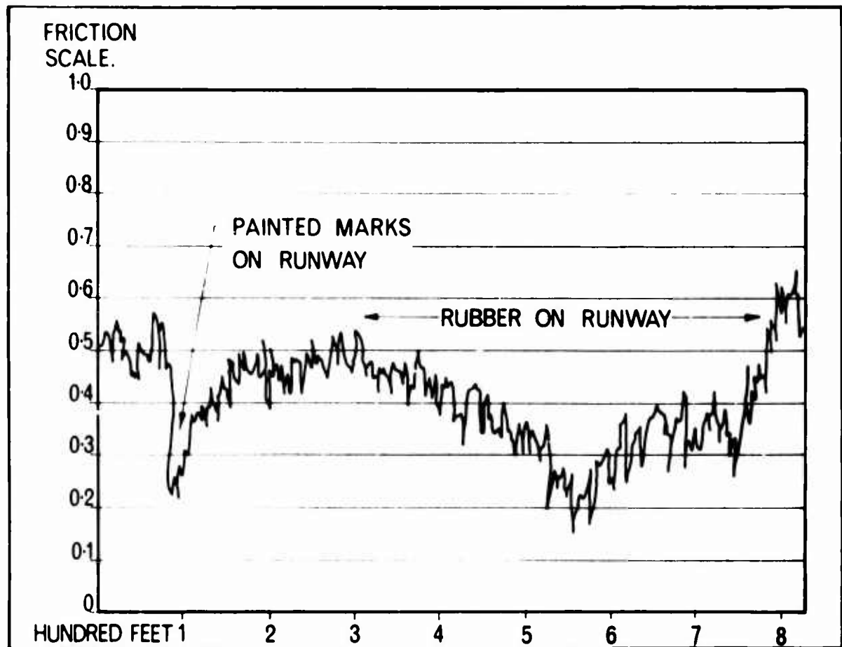
Figure D4.- Part of friction meter record showing rubber deposits in touchdown area.
