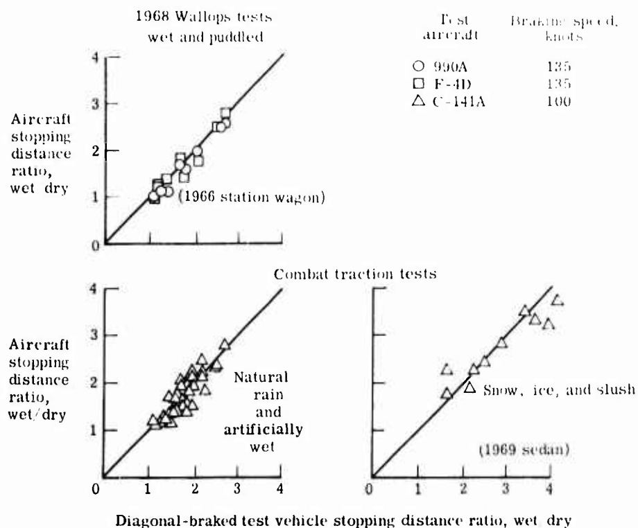
Figure 17.- Correlation between aircraft and test vehicle stopping distance ratios. The diagonal-braked test vehicle stopping distance ratio was determined by using a dry stopping distance of 302 feet for the snow, ice, and slush tests.
