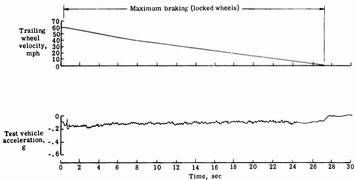
(c) Glazed-ice and snow-covered runway condition. Slurry seal runway at Loring AFB.
