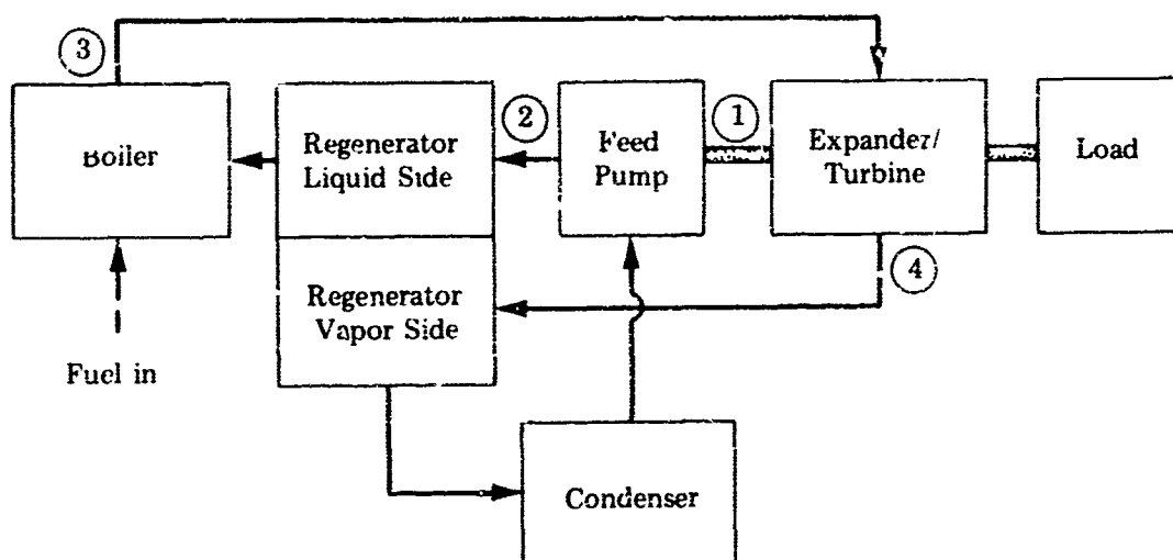
Figure 2. BASIC FLOW SCHEMATIC FOR ORGANIC RANKINE-CYCLE SYSTEM
