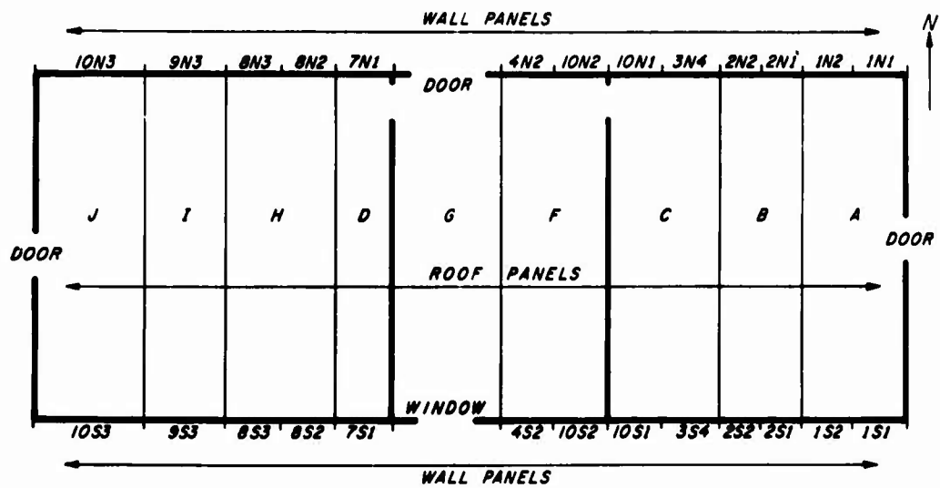
Figure 2.--Positions of numbered wall and roof panels in the sandwich experimental unit (1968).
