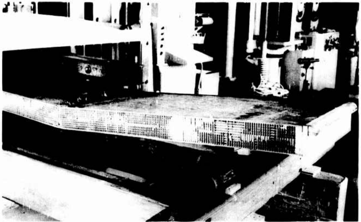
Figure 10.--Final failure of unventilated roof panel after 21 years' exposure.
