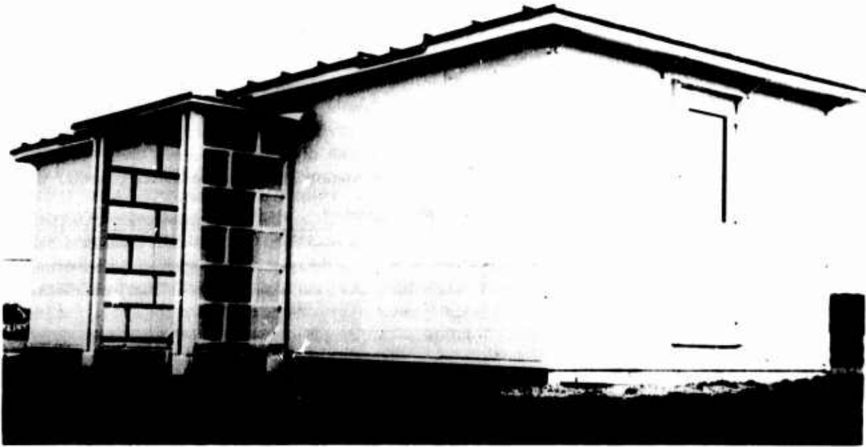
Figure 1.--Sandwich experimental unit as re-erected in 1968.
