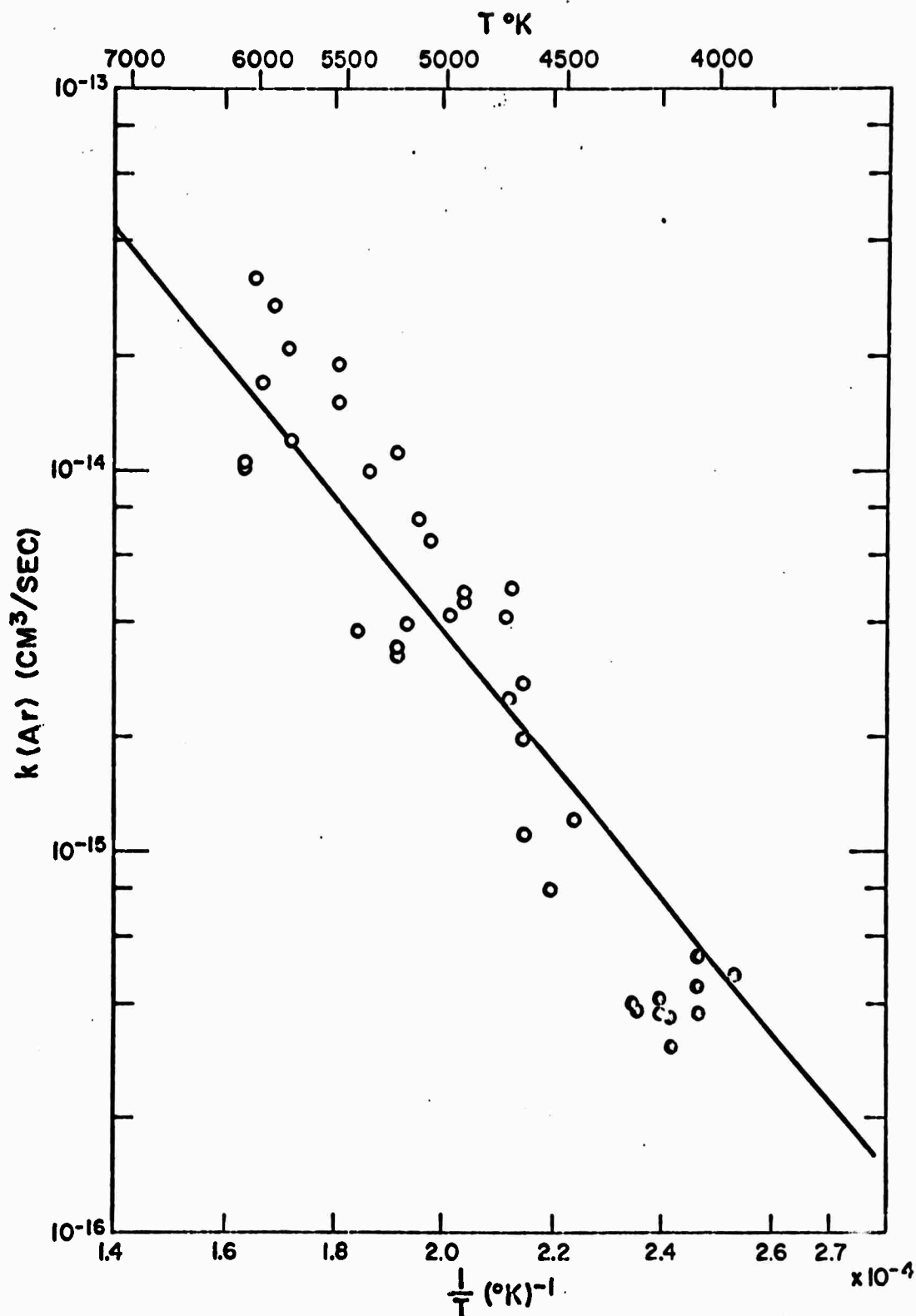
Fig. 2 The electron detachment rate of \text{F}^- assuming impact ionization by the atomic argon [ k(\text{Ar}) \text{ cm}^{-3}/\text{sec} ] as a function of 10^4 \text{ K}/T . The effect of the \text{Cs}^+ (as determined from Fig. 1) has been subtracted. The solid line shows the dependence of a detachment rate having an activation energy equal to the electron affinity of \text{F}^- . The open circles are incident shock measurements and the closed circles are reflected shock measurements.
