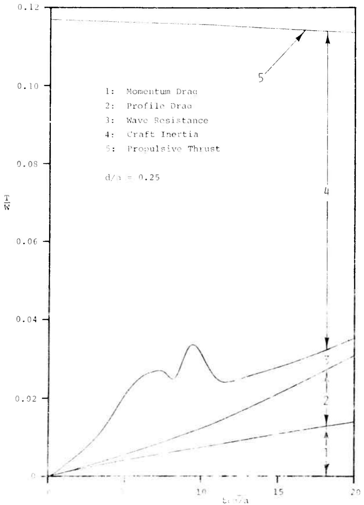
Fig. 2.10. Drag Coefficient C_D vs. W/L (for d/a = 0.25 )
