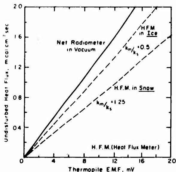
Figure 1. Response of a cylindrical thermopile 4.5 cm in diameter and 1.25 cm thick surrounded by a Perspex annulus of 15 cm outer diameter when temporarily operated as a net radiometer in vacuum and as an HFM in ice and snow of thermal conductivity 5 \times 10^{-3} and 2 \times 10^{-3} cal \text{cm}^{-1} \text{°C}^{-1} \text{sec}^{-1} respectively. The method of establishing the conductivity ratio k_m/k_s is described on p. 25-29.
