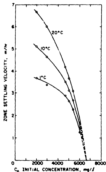
Figure 10. Zone settling velocity vs concentration (data interpolated from Fig. 9).
