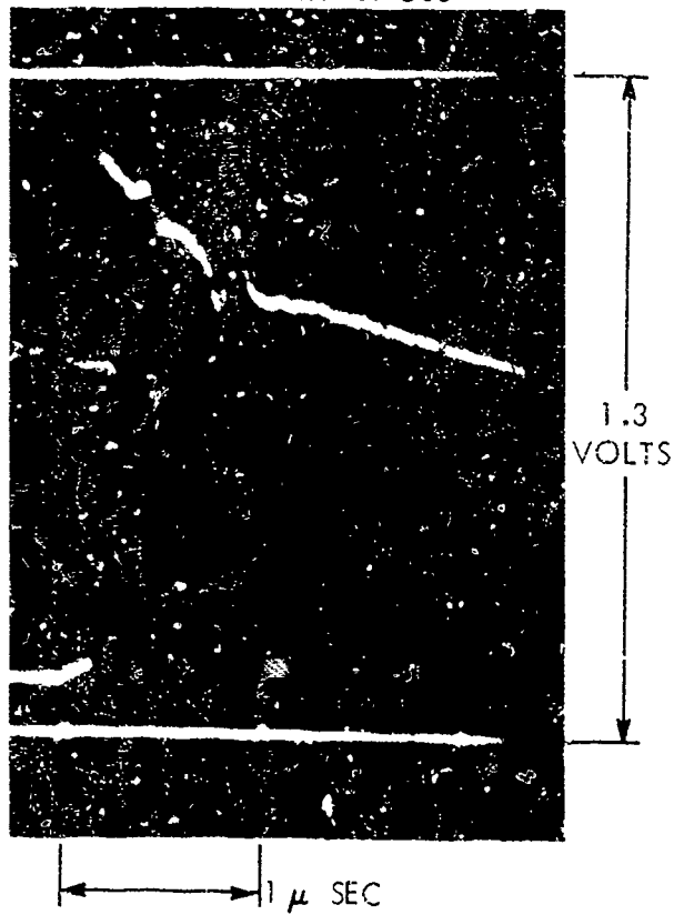
A SHOT # 92 FIELD 1020 GAUSS
