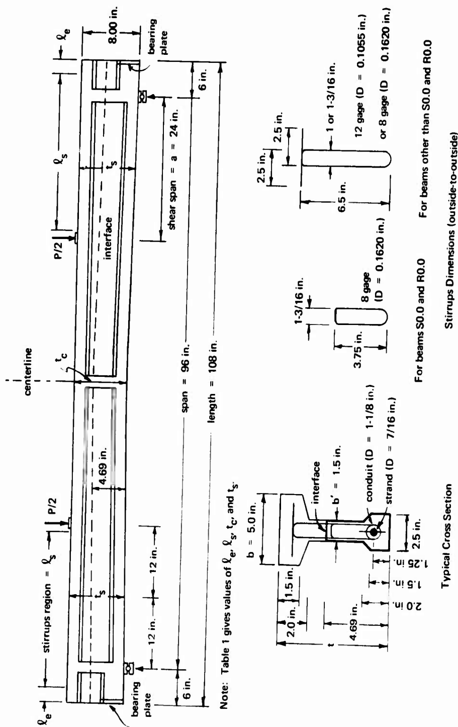
Figure 1. Details of test beams.
