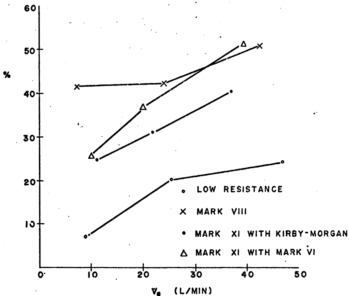
FIG. 38 - PERCENT OF TOTAL RESPIRATORY WORK DUE TO EXTRINSIC RESPIRATORY WORK BREATHING \text{SF}_6\text{-O}_2 AT DIFFERENT RESPIRATORY MINUTE VOLUMES WITH THE LOW RESISTANCE SYSTEM AND THE MARK VIII AND XI UBA
