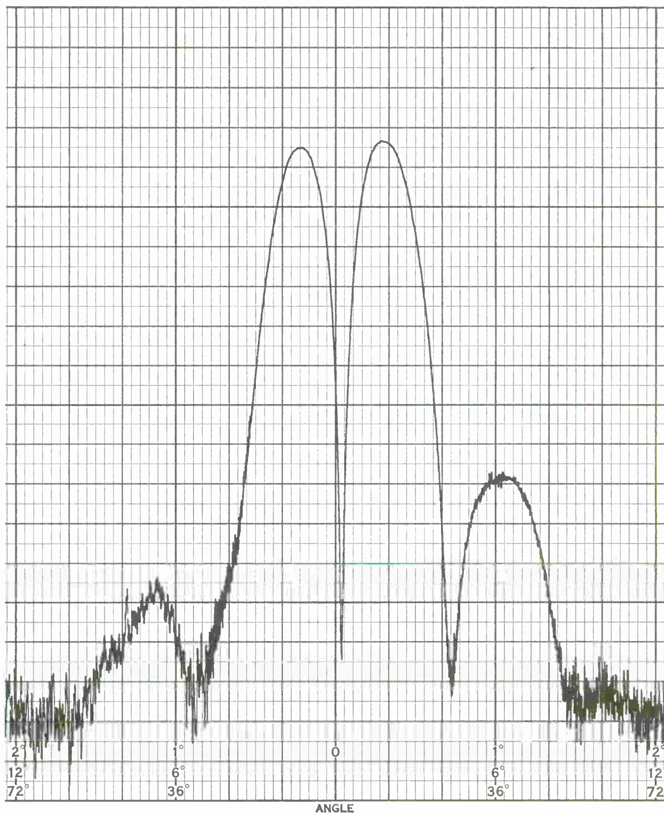
Figure C-4 Full Scale UHF Secondary Difference Patterns at 395 MHz with FSS No. 2, AZ Scan, Transmit Source - RHCP, Receive - RHCP.
