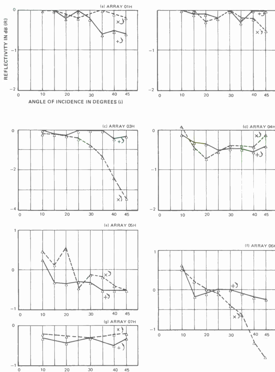
Figure A-4 Reflectivity as a Function of Angle of Incidence for Cylindrical Element Arrays
