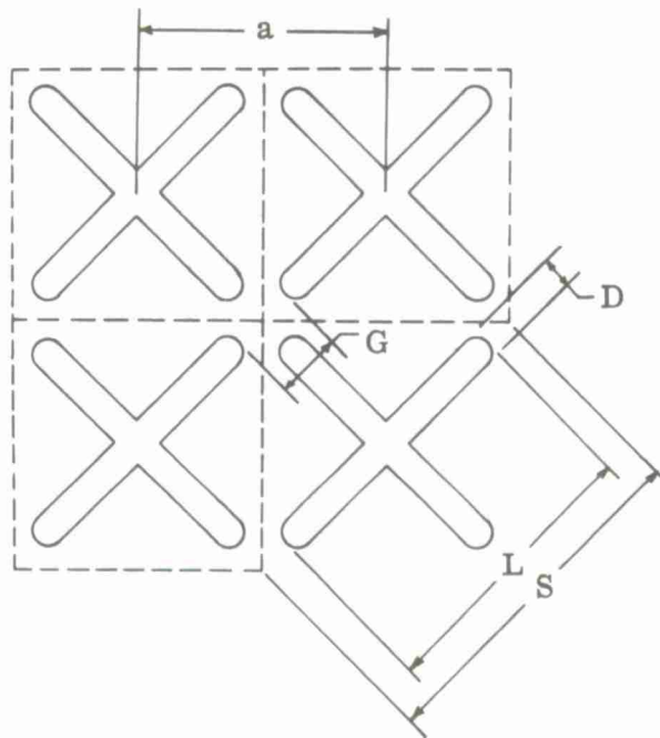
Figure 2 Array Geometry
