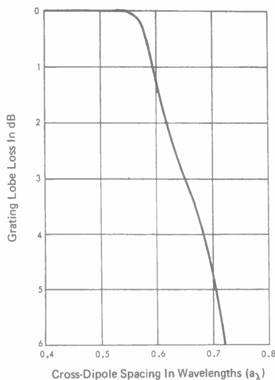
Figure 10 Grating Lobe Loss vs Cross-Dipole Spacing for a Typical Hyperbolic Reflector
