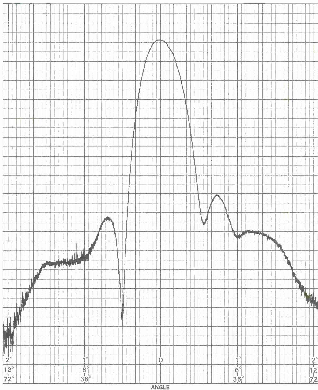
Figure C-3 Full Scale UHF Secondary Sum Patterns at 395 MHz with FSS No. 2 AZ Scan, Transmit Source- RHCP, Receive - RHCP
