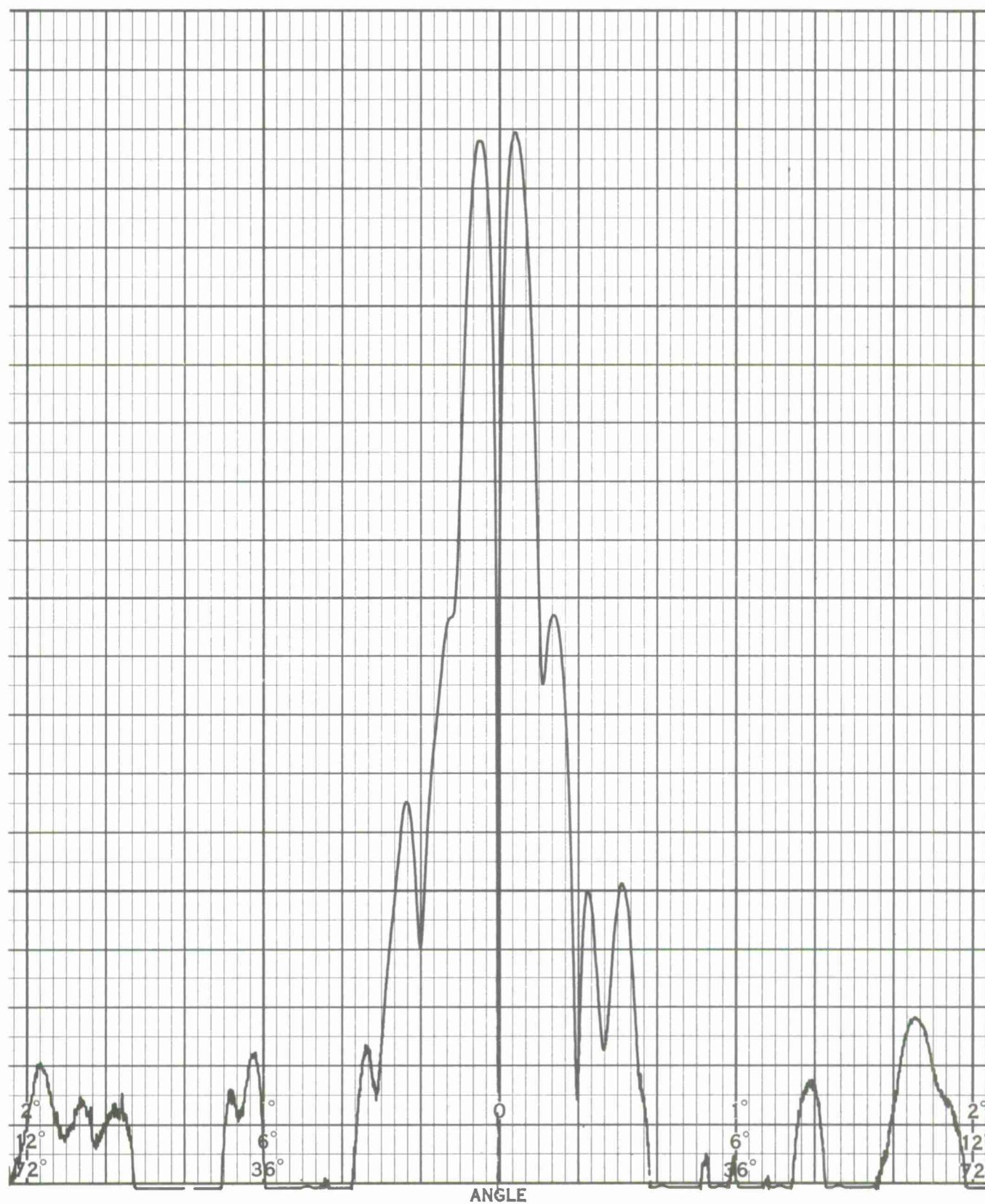
Figure C-1(a) Full Scale L-Band Secondary Difference Patterns at 1295 MHz with FSS No. 2, AZ Scan, Transmit Source - Vertical Polarization, Receive - RHCP.
