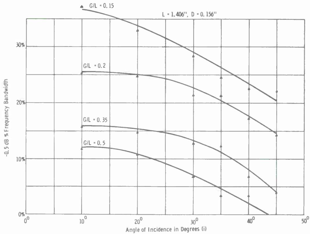
Figure 6 Bandwidth vs Angle of Incidence ( i )
