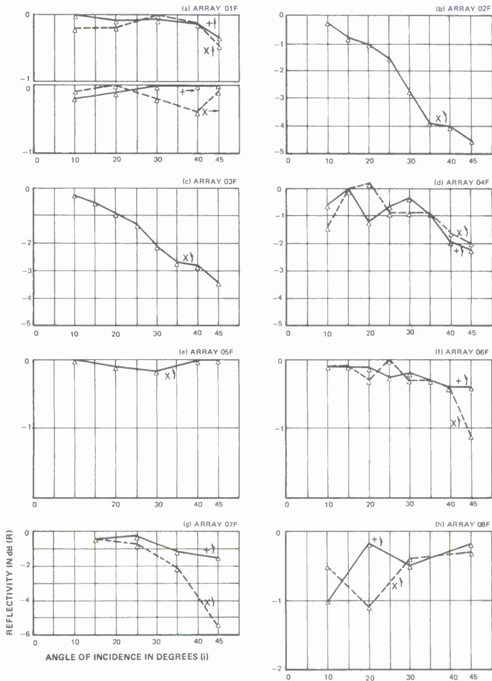
Figure A-3 Reflectivity as a Function of Angle of Incidence for Flat-Element Arrays
