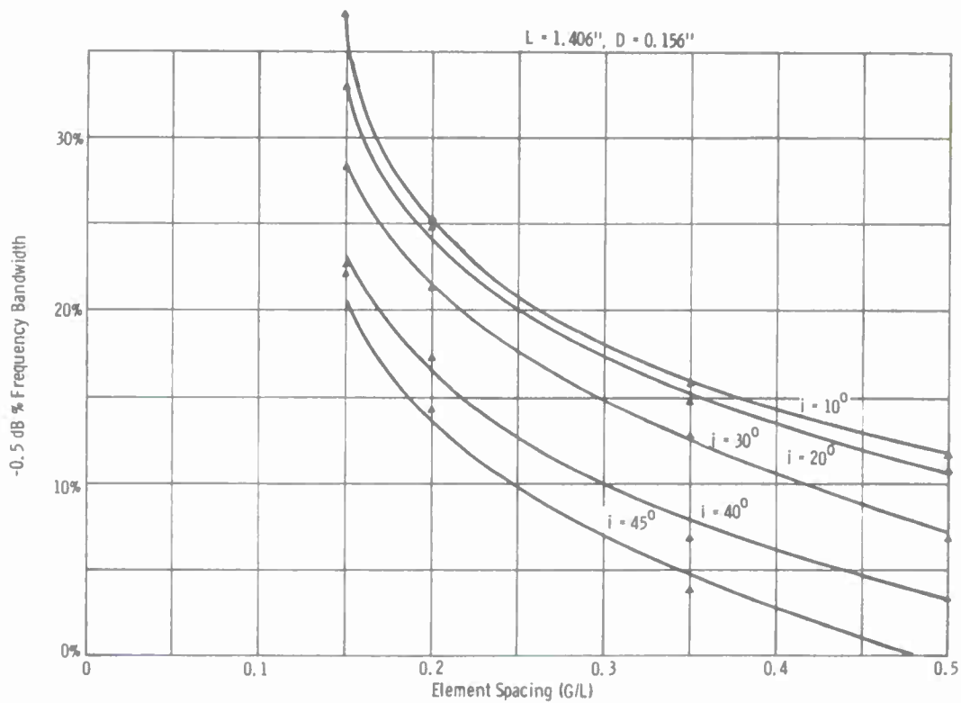
Figure 7 Bandwidth vs Element Spacing ( G/L )
