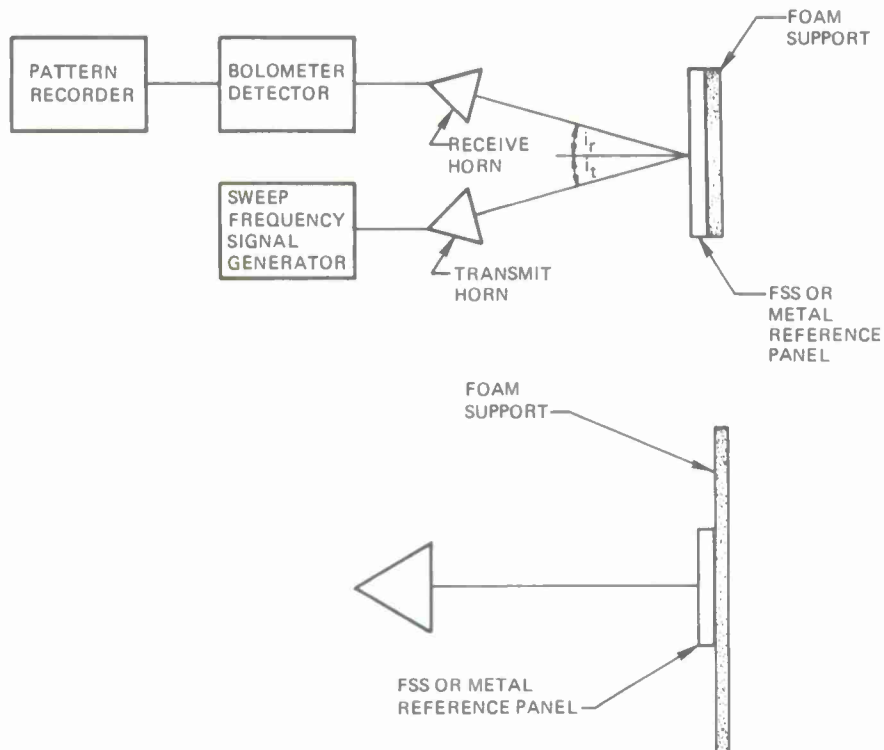
Figure 3 Reflectivity Test Set-Up
