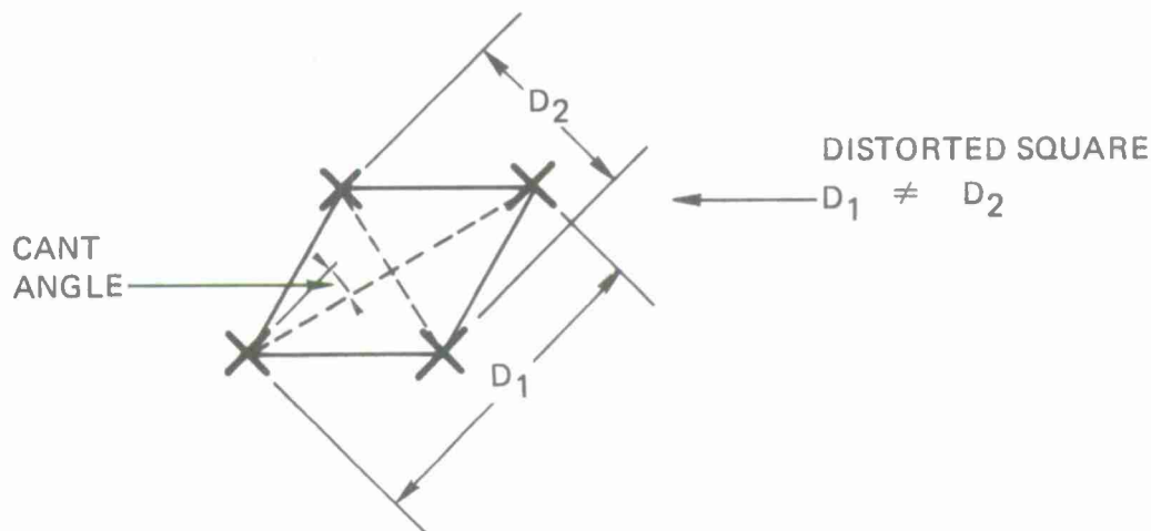
Figure 18 Effect of Distorted Grid
