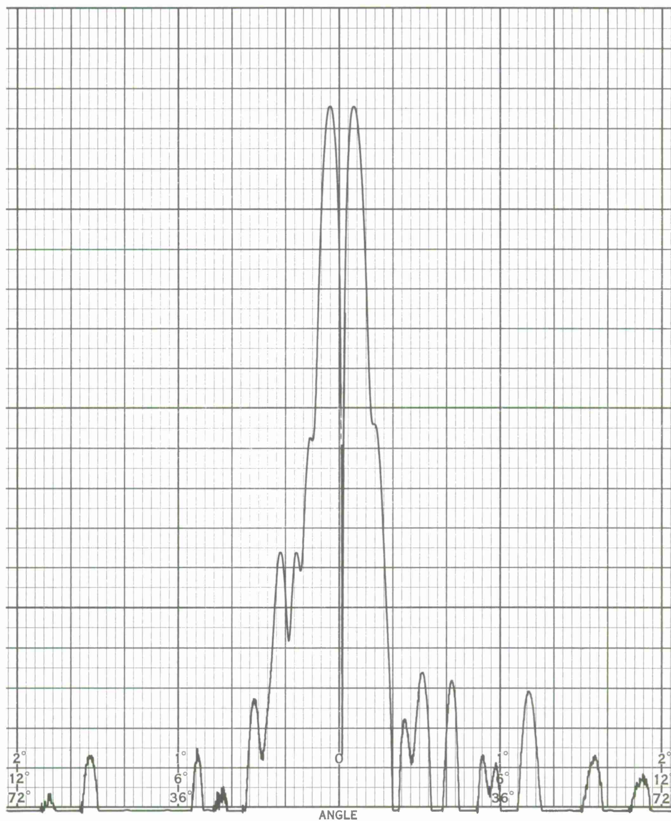
Figure C-2(a) Full Scale L-Band Secondary Difference Patterns at 1295 MHz with FSS No. 2, AZ Scan, Transmit Source - Horizontal Polarization, Receive - RHCP.
