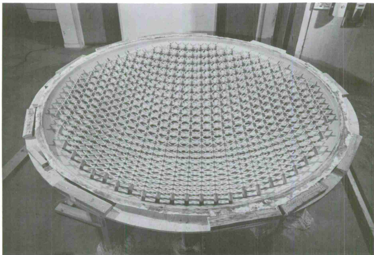
Figure 16 Completed Interior of M.I.T. - FSS
