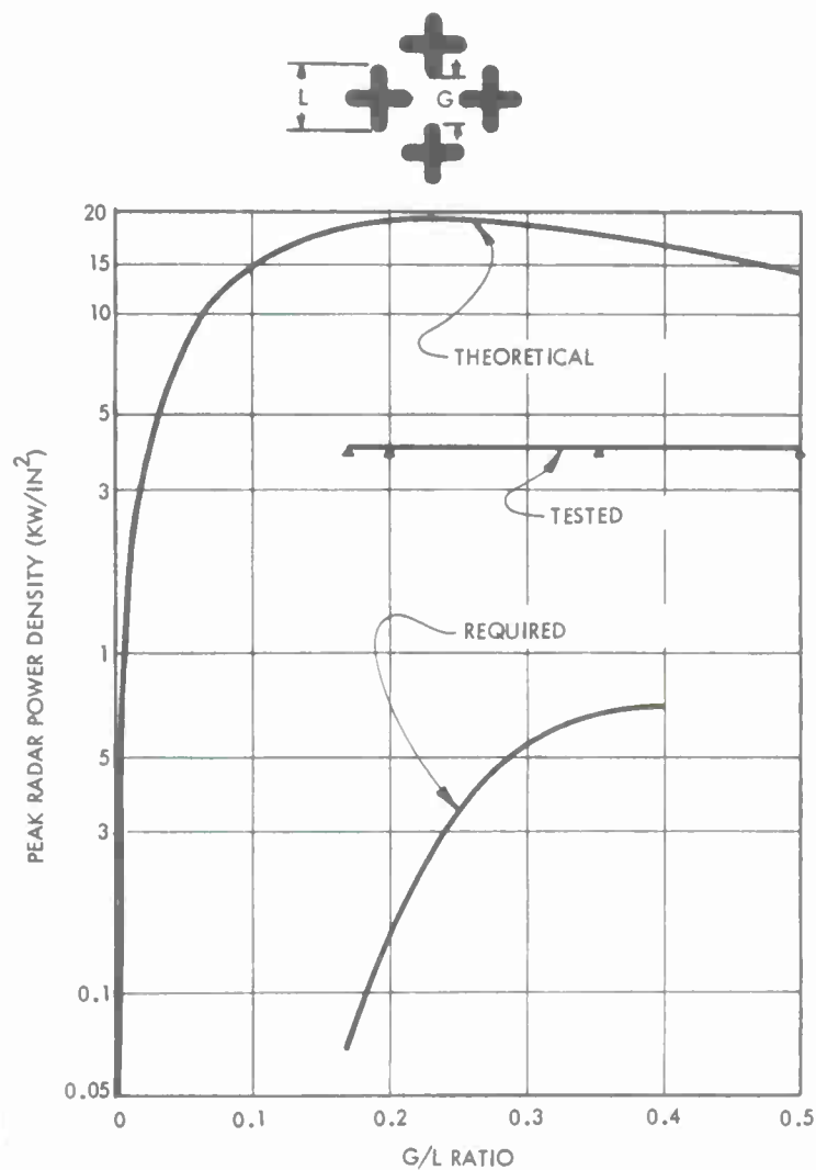
Figure 26 Power Density vs Element Spacing
