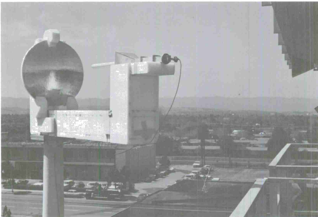
Figure 20 Scatter Pattern Test Set-Up with Metal Reference Subreflector
