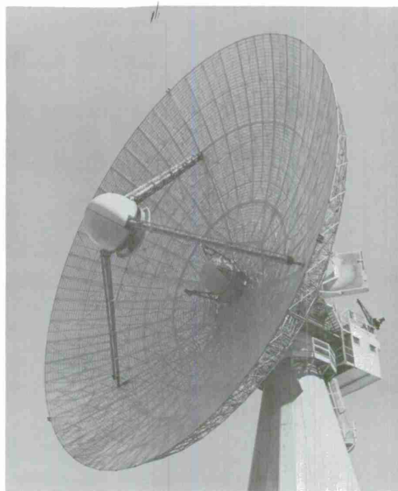
Figure 17 M.I.T. Millstone Hill Antenna with FSS Subreflector
