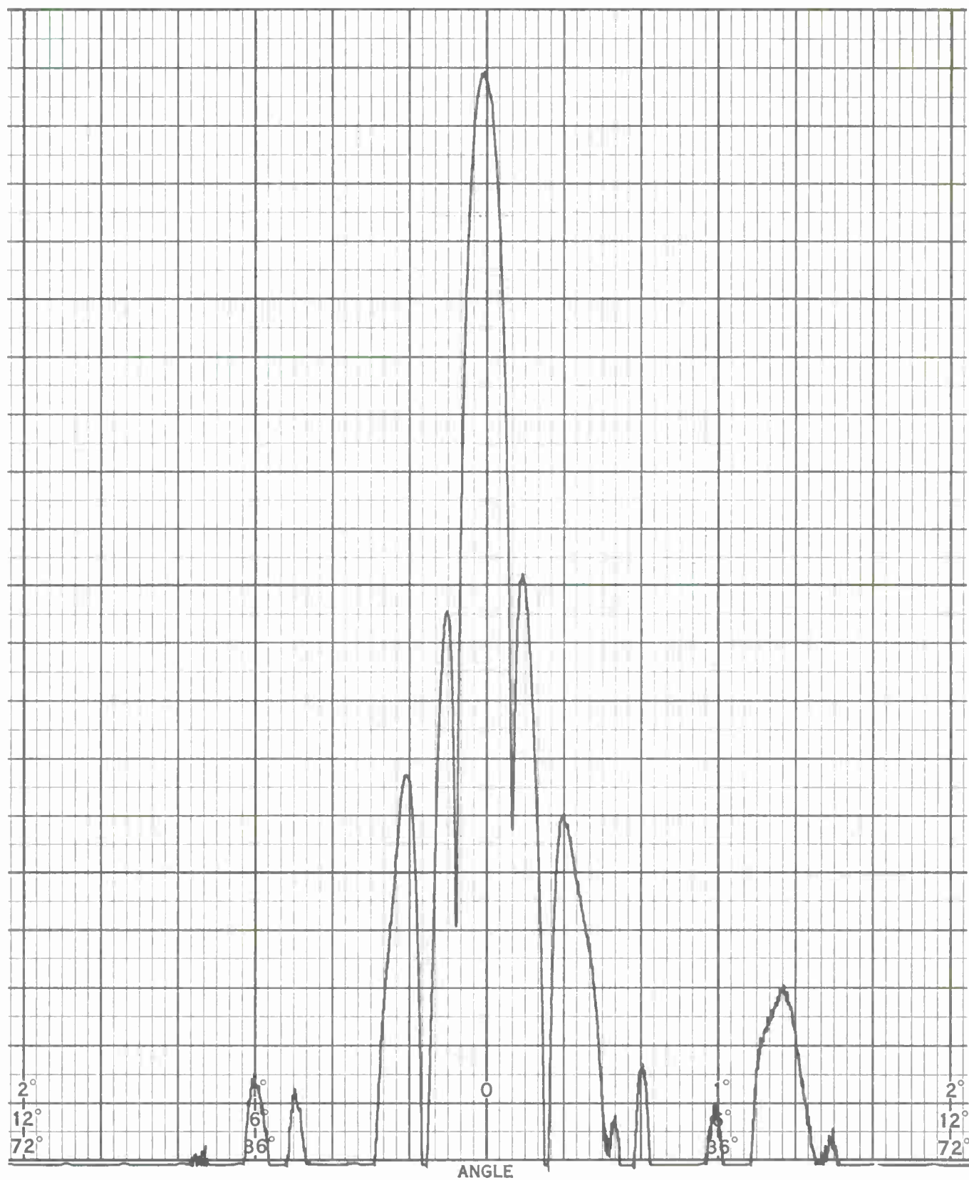
Figure C-1(b) Full Scale L-Band Sum Patterns at 1295 MHz with FSS No. 2, AZ Scan, Transmit Source - Vertical Polarization, Receive-RHCP.
