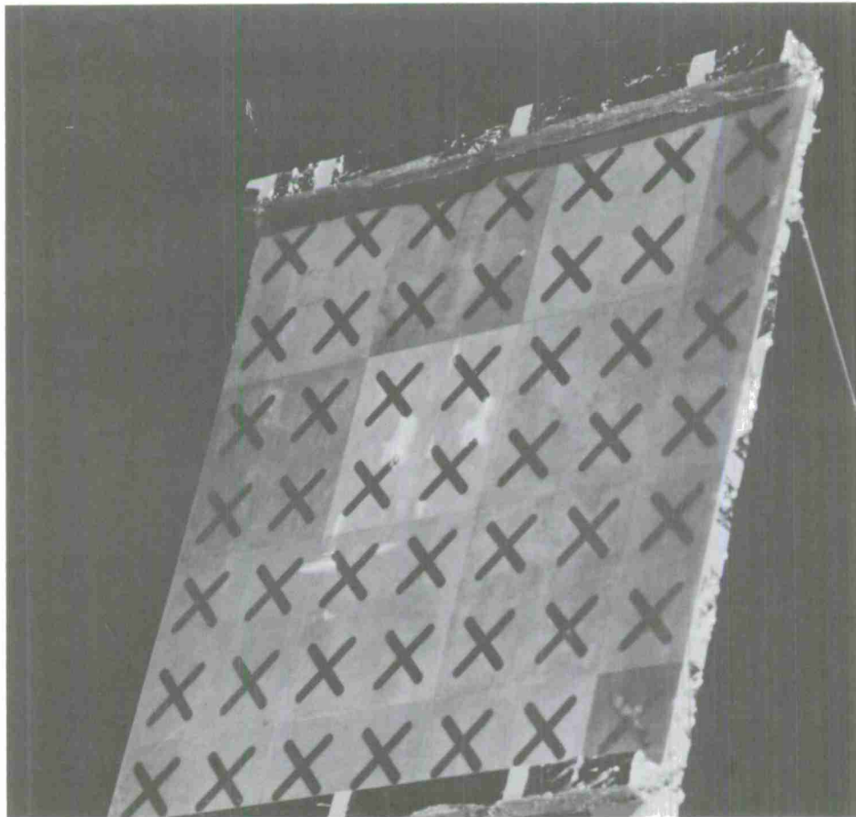
Figure 24 FSS Test Panel During RF Power Failure
