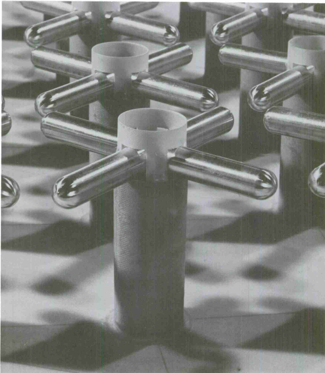
Figure 25 Cross-Dipole and Standoff Assembly
