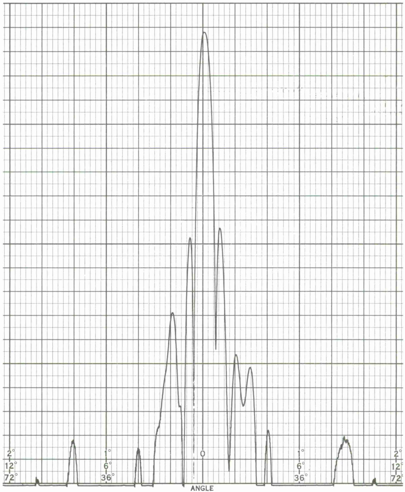
Figure C-2(b) Full Scale L-Band Sum Patterns at 1295 MHz with FSS No. 2, AZ Scan, Transmit Source - Horizontal Polarization, Receive-RHCP.
