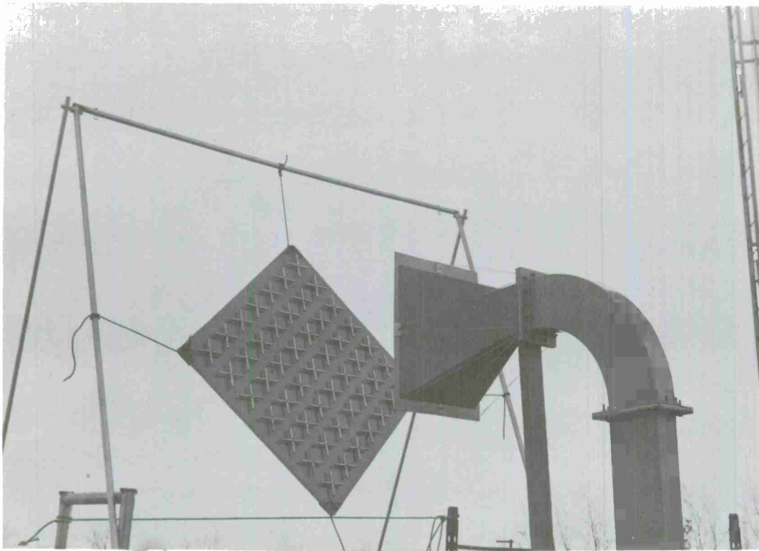
Figure 27 High-Power Test Range
