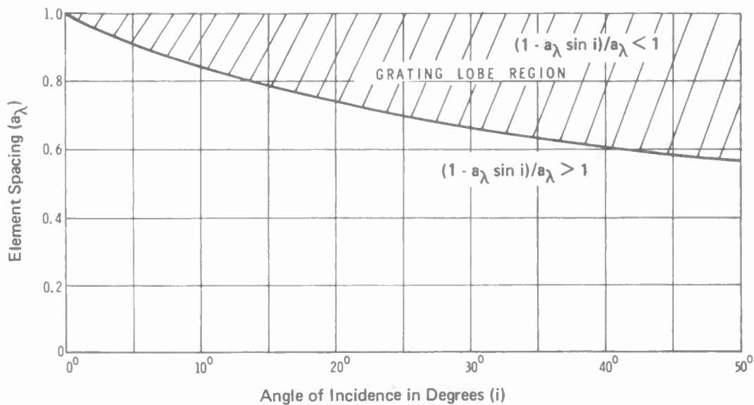
Figure 8 Grating Lobe Spacing vs Angle of Incidence ( i )
