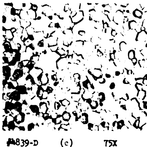
Figure 7. Microstructure of Three High Purity \text{MgO} Hot Pressed Specimens Pressed from \text{Mg}(\text{OH})_2 Derived Powder after Various Hot Pressing Cycles.
