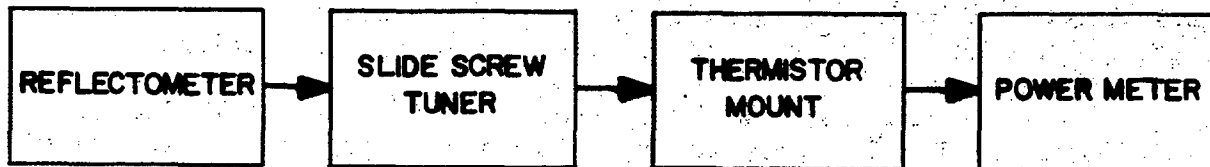
Figure 2. Test configuration for measuring average power. Tuner eliminates mismatch between exciter and thermistor mount, removing reflection coefficient terms from measurements.
