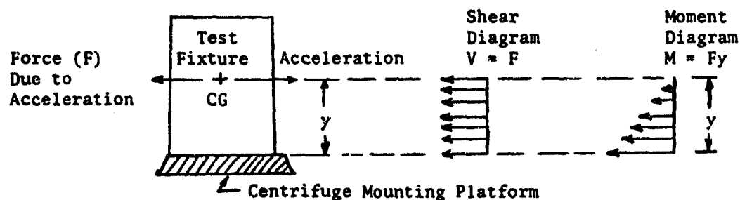
Typical Installation Utilizing a Fixture
