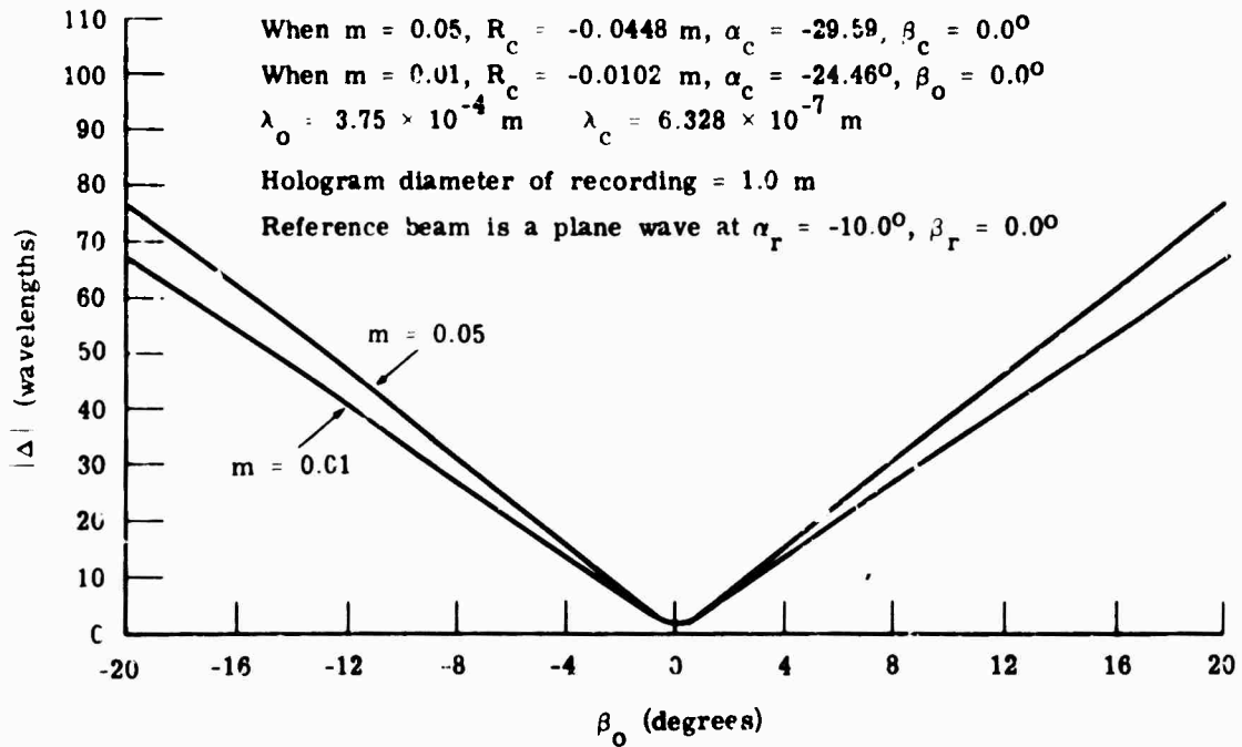
FIGURE 26. MAGNITUDE OF THE WAVE ABERRATION |\Delta| VS. \beta_o USING ABERRATION BALANCING. The reconstruction geometry is calculated for the object point R_o = 0.5 m, \alpha_o = 75.00^\circ , \beta_o = 0.00^\circ , according to the aberration-balancing technique. For each value of m , R_c and \alpha_c , the wave aberration is calculated as a function of \beta_o , with R_o = 0.5 m, and \alpha_o = 75.00^\circ .
