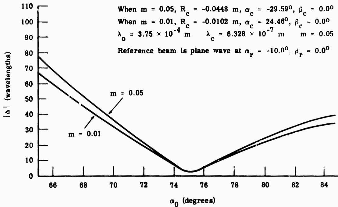
FIGURE 25. MAGNITUDE OF THE WAVE ABERRATION |\Delta| VS. \alpha_o USING ABERRATION BALANCING. The reconstruction geometry is calculated for the object point R_r = 0.5 m, \alpha_o = 75.0^\circ , \beta_o = 0.0^\circ , according to the aberration-balancing technique. For each value of m , R_c and \alpha_c , the wave aberration is calculated as a function of \alpha_o , with R_o = 0.5 m, and \beta_o = 0.0^\circ .
