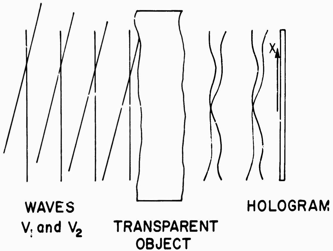
FIGURE 8. OPTICAL ARRANGEMENT FOR RECCRING THE HOLOGRAM
