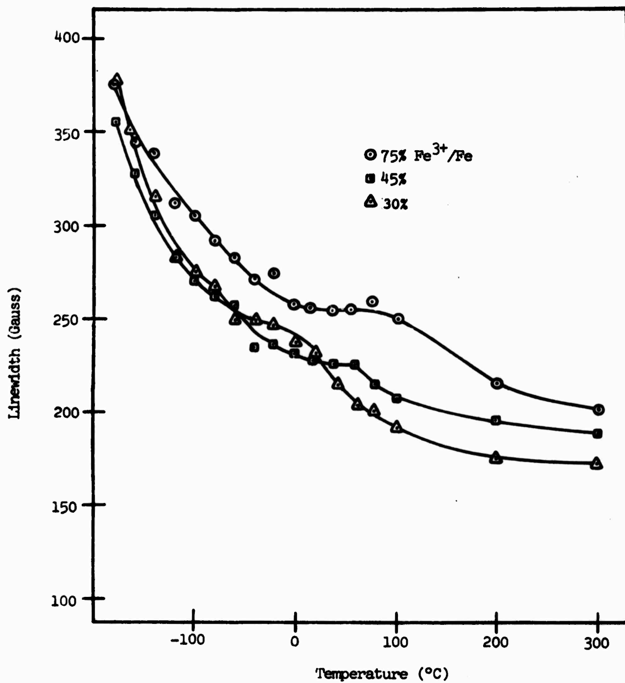
FIGURE 7. ESR Linewidth of the g'=2.00 Line as a Function of Experiment Temperature for Glass Samples Heat-Treated at 600°C for One Hour.
