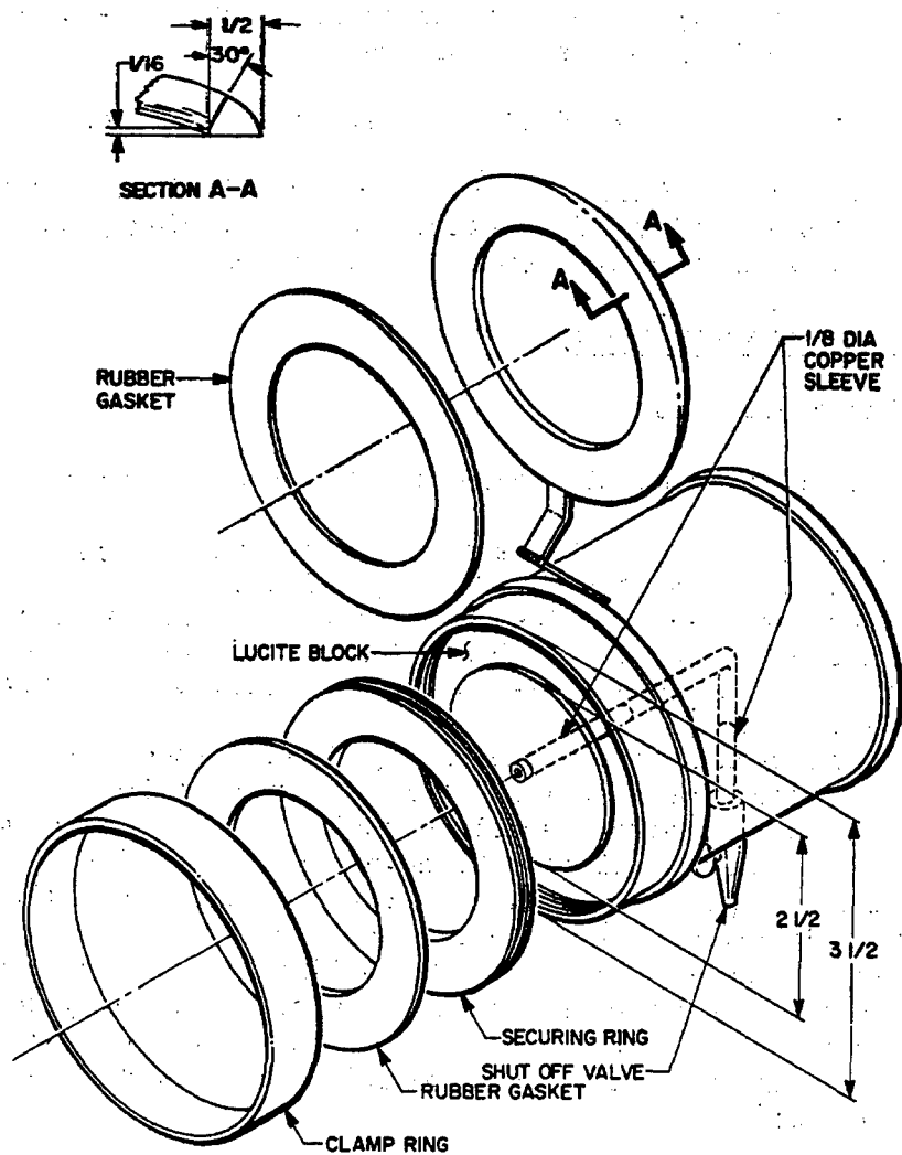
Figure 1 - Patch Box
