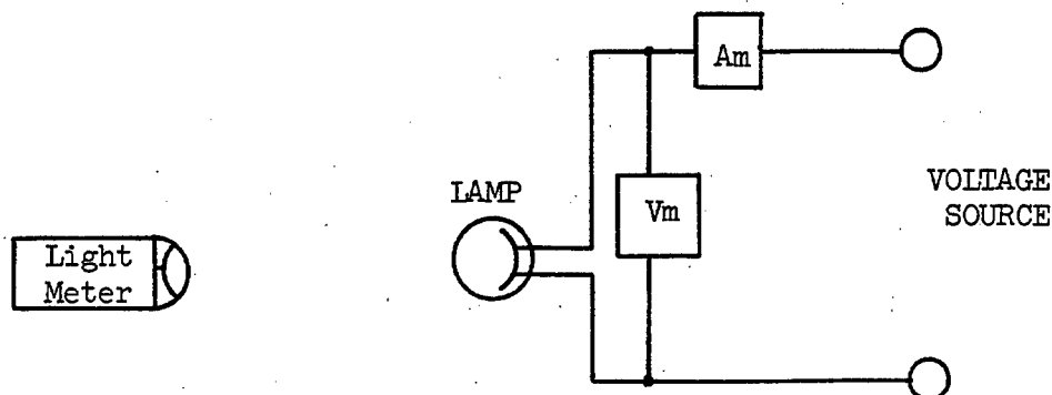
Figure 1. Connection of Calibrated Voltmeter and Ammeter.
