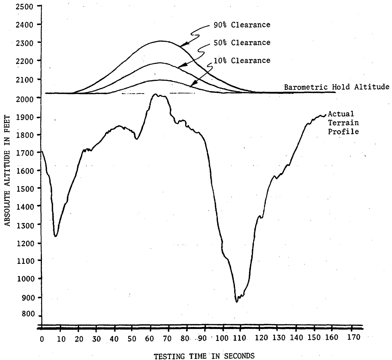
FIGURE 2. Hypothetical Terrain Clearance Accuracy Curve.
