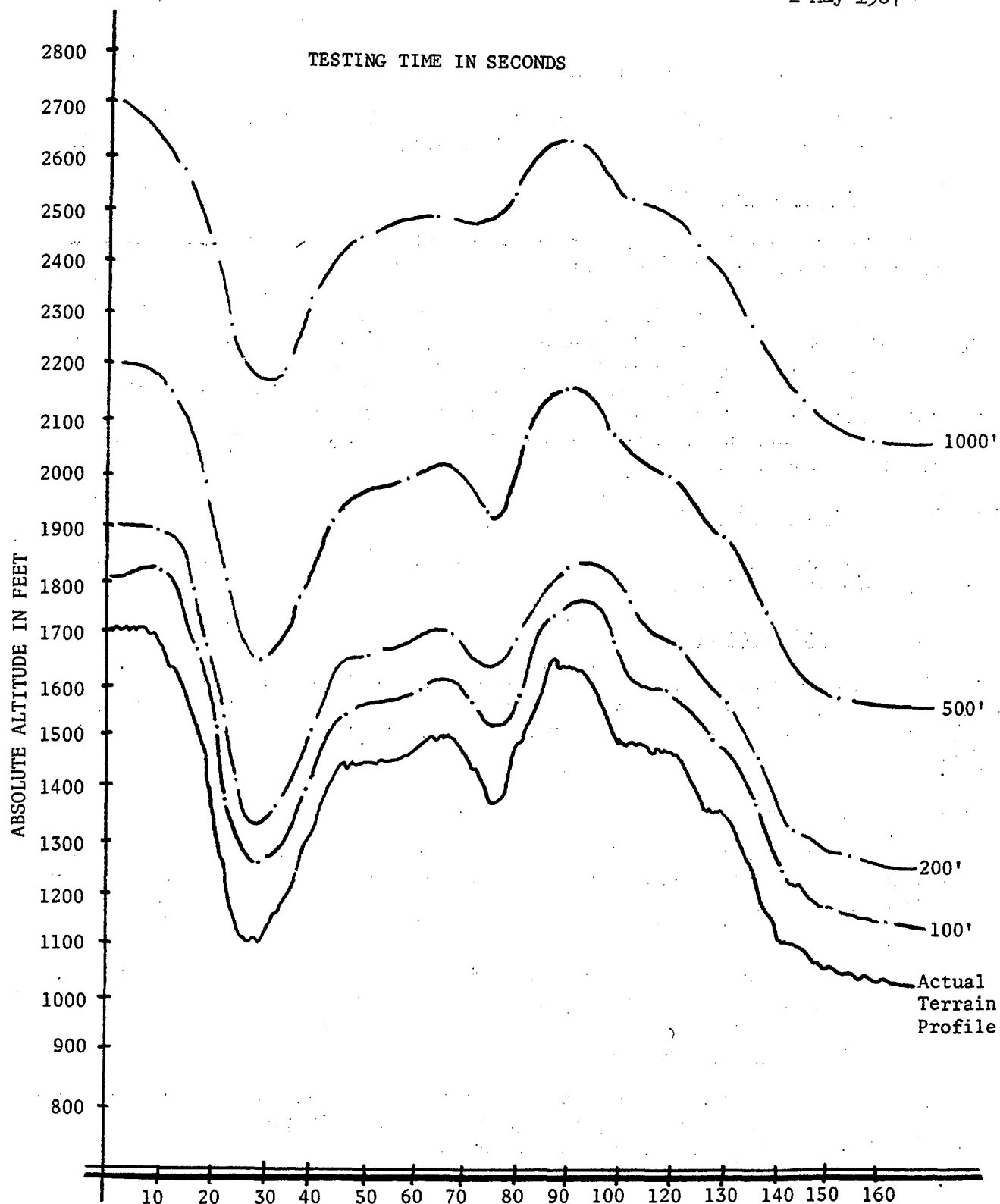
FIGURE 3. Hypothetical Profile Following Test Accuracy Curve.
