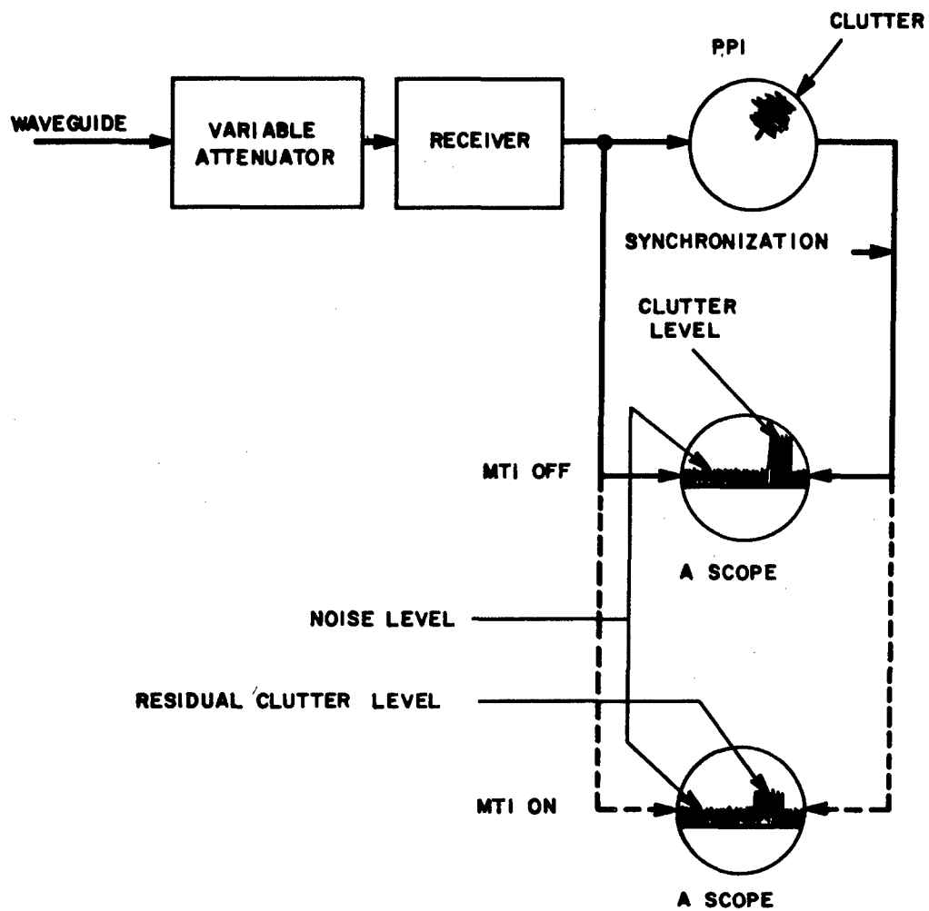
Figure 2. Signal Attenuation Method of Measuring Clutter Amplitude
