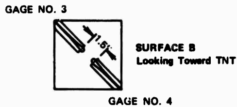
FIGURE 1 GAGE ARRANGEMENT FOR SHOT NO. 3
