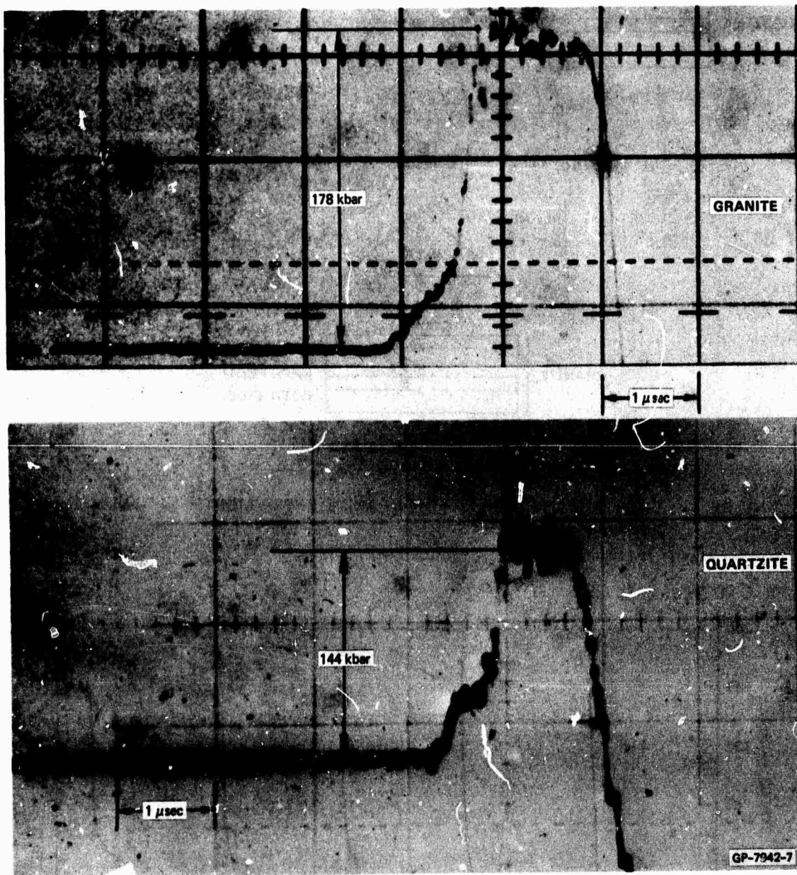
FIGURE 6 PRECURSOR IN GRANITE COMPARED WITH PRECURSOR IN QUARTZITE BOTH AT 2 INCH DEPTH. Shot No. 12 and 3.
