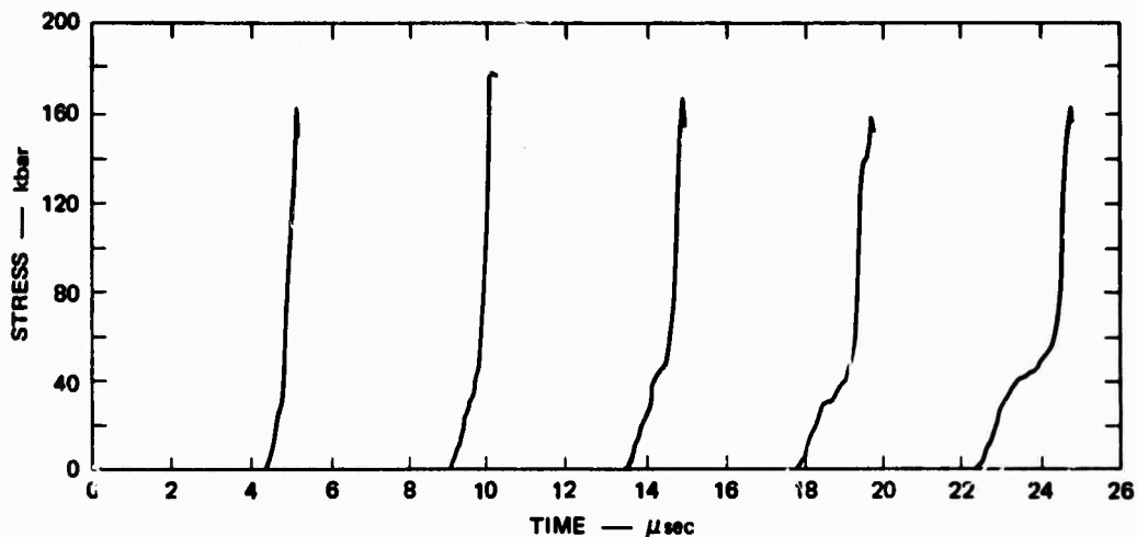
FIGURE 5 PRECURSOR DEVELOPMENT IN GRANITE. Gages at 1 inch intervals. Shot No. 12.
