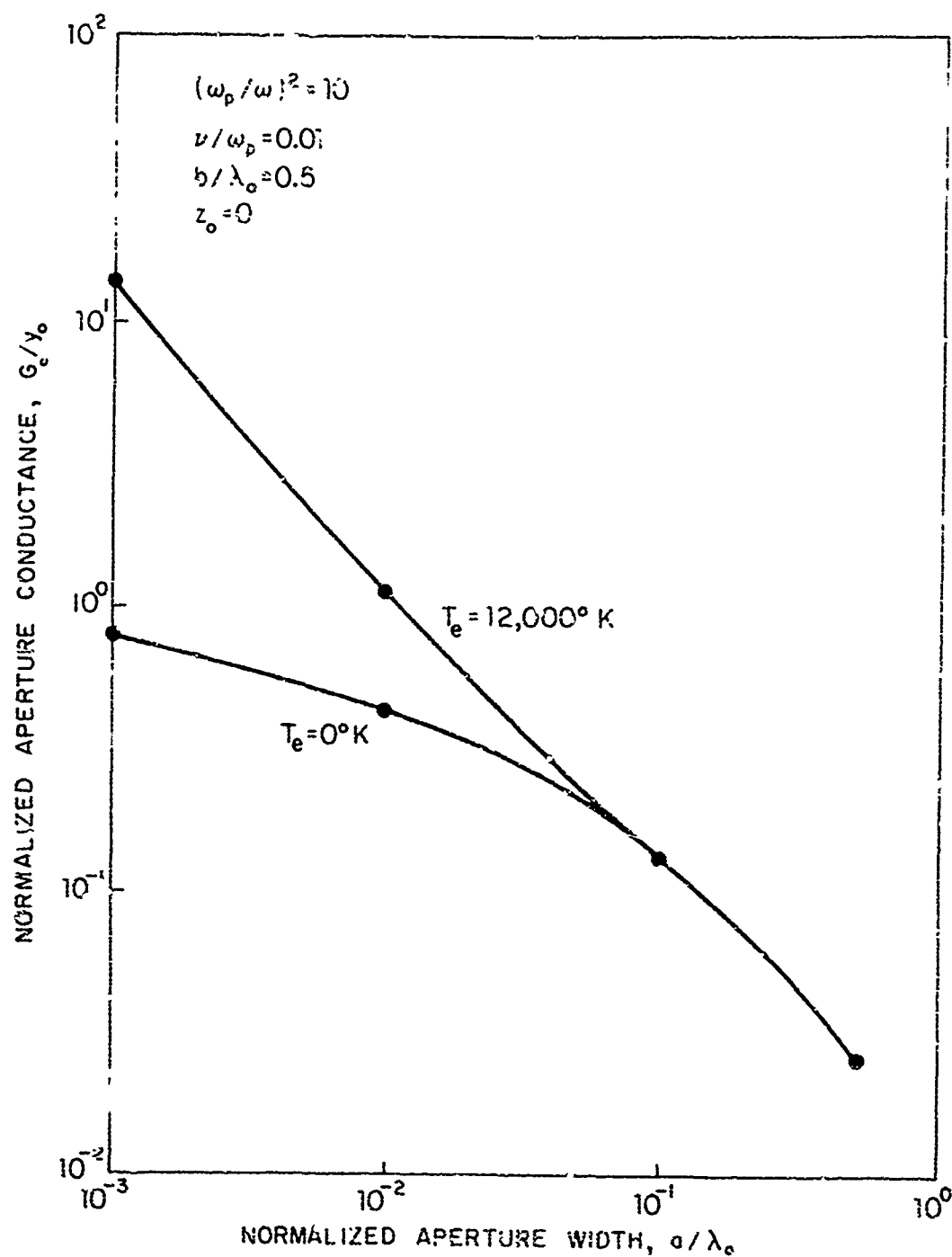
Figure II-13. Normalized conductance of aperture radiating into overdense plasma; effect of aperture width.
