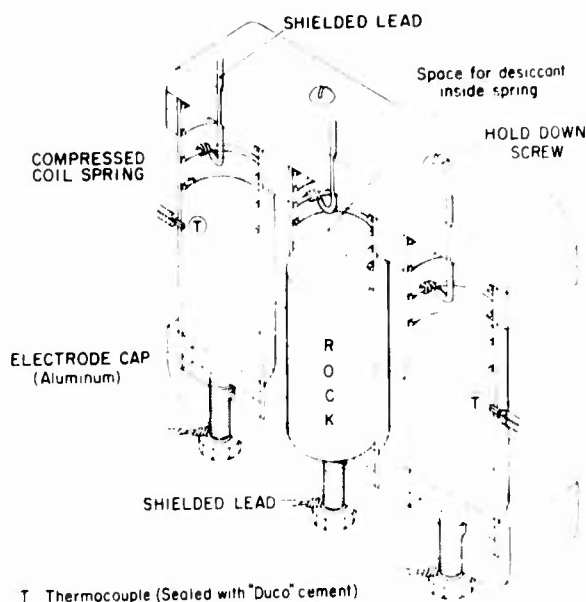
Figure 20. Test cell used for low temperature electrical conductivity measurements.
