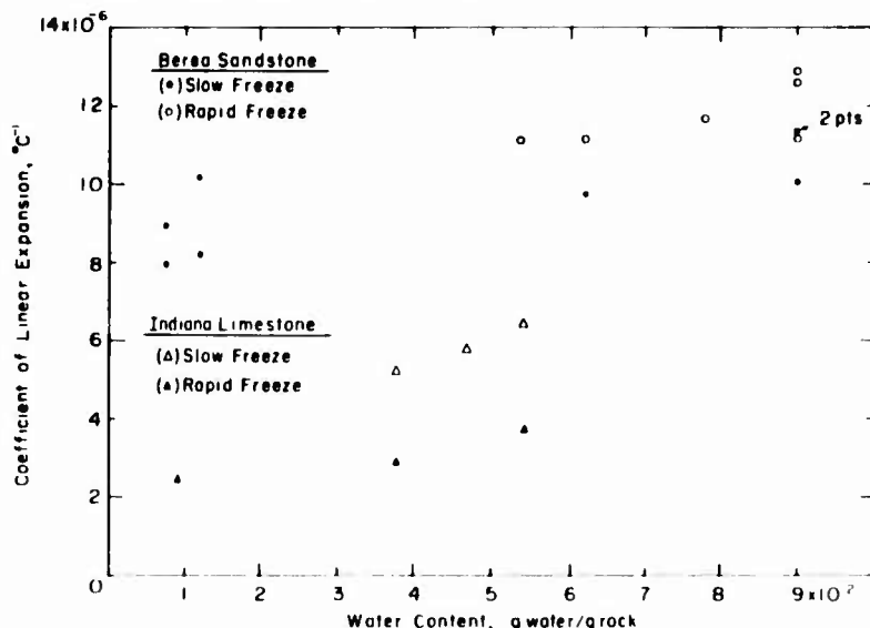
Figure 42. Coefficient of linear expansion (approximately -15° to -90°C) plotted against water content for Berea sandstone and Indiana limestone.
