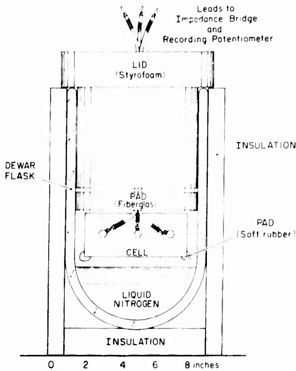
Figure 21. Arrangement of test cell in Dewar flask.
