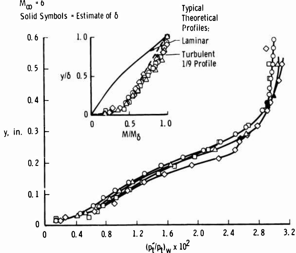
Fig. 41 Effect of Reynolds Number on Boundary-Layer Profiles at M_w = 6.0
