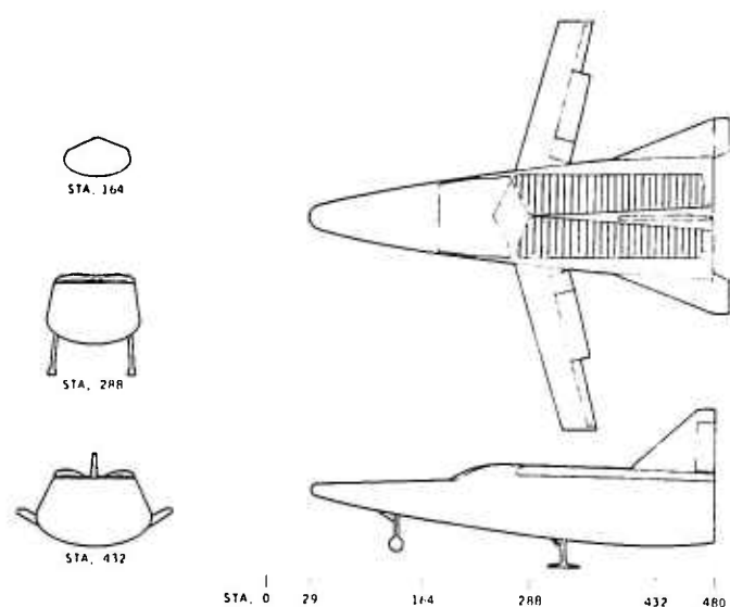
Hypersonic L/D ≈ 2 Vehicle.
