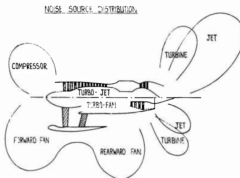
Fig. 20 Noise source distribution
