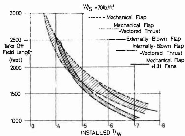
Fig.4 Take-off performance
