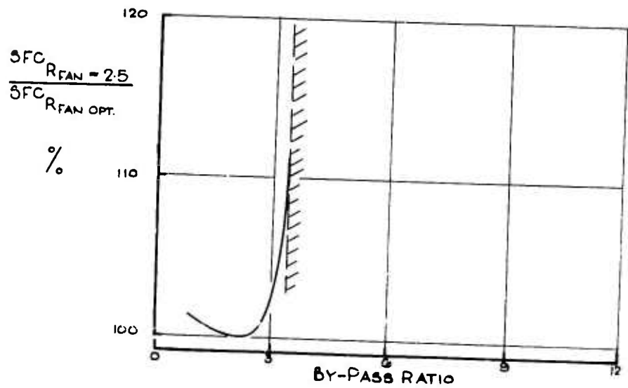
Fig.6 Performance penalty for maintaining fan pressure ratio constant at 2.5
