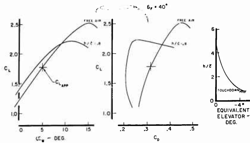
Fig. 30 Ground effect. Tail on, s_{FR1} = -10^\circ
