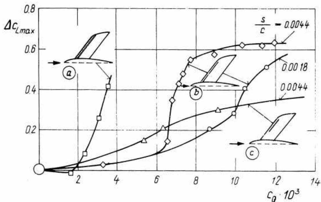
Fig.6 "Increment in C_{Lmax} due to nose suction for a 40 deg swept-back wing" Wind-tunnel tests after E.D.Poppleton [10] (a) porous leading-edge, (b) leading-edge slot (full span) (c) leading-edge slot (half span)
