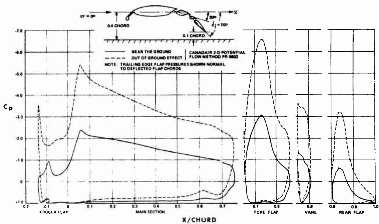
Fig.4 Theoretical pressure distributions on a modified NACA 4418 with deflected triple slotted flap and Krüger flap close to the ground and out of ground effect
