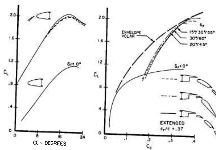
Fig.9 Trailing-edge effects
