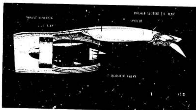
Fig.4 Externally-blown jet-flap
