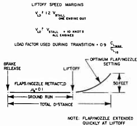
Fig.14 Takeoff profile
