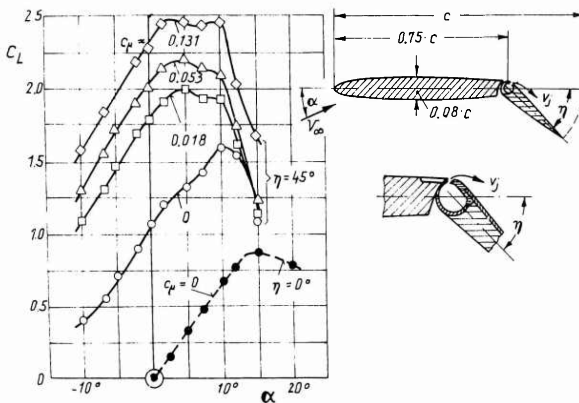
Fig.16 Effect of blowing over the trailing-edge flap on the lift coefficient Wind-tunnel tests after J.Williams [13]
