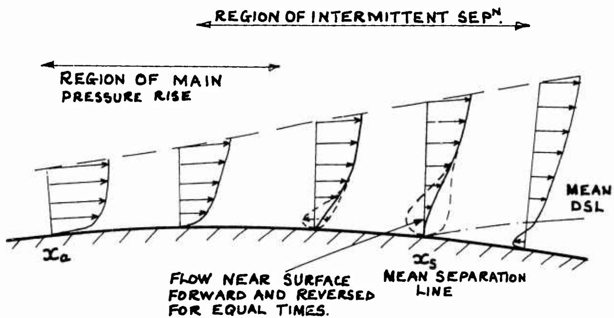
Fig.2 Turbulent separation
