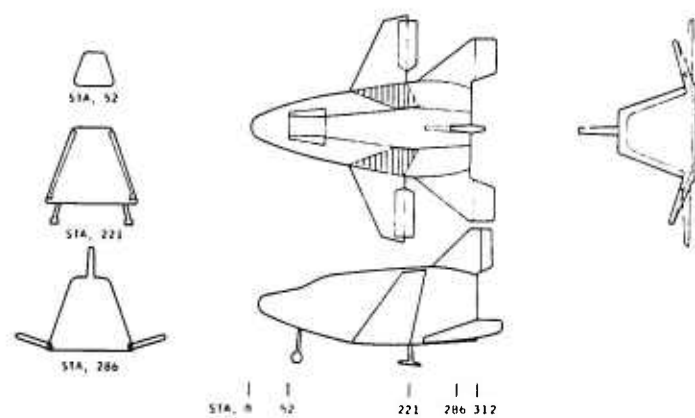
Hypersonic L/D ≈ 1 Vehicle.
