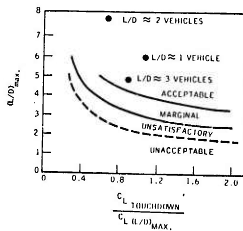
L/D Versus C_L/C_L (L/D \text{ max.}) Requirements.
