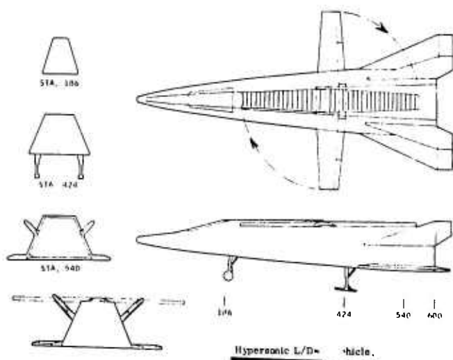
Hypersonic L/D ≈ 3 Vehicle.
