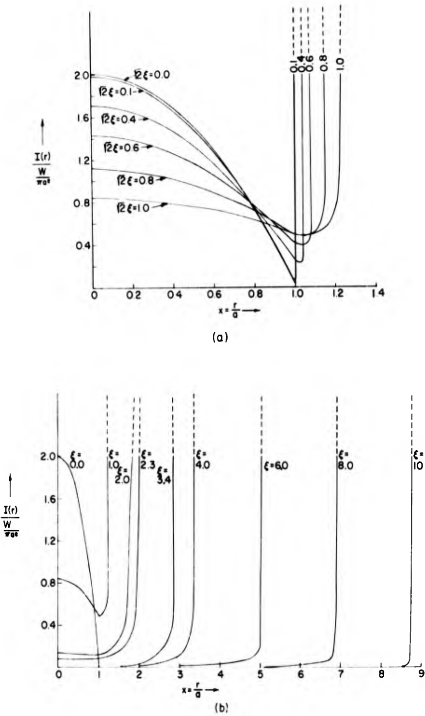
Fig. 6 - Reduced intensity as a function of reduced radial distance x for a parabolic intensity distribution. The parameter \xi has the range of values (a) 0.0 < \sqrt{2}\xi < 1.0 and (b) 0.0 < \xi < 10
