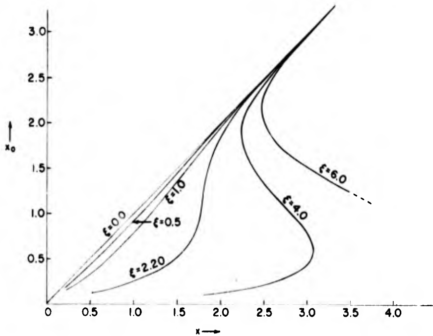
Fig. 8 - Plot of x_0 vs. x for the Gaussian intensity distribution with \xi as a parameter
