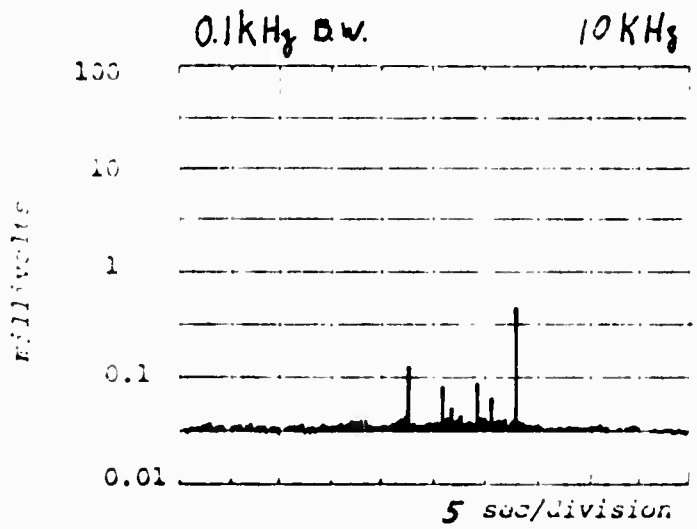
Figure 3. Emission output vs. time similar to that in Figure 2, but observed through a 10 KHz, 0.1 KHz bandwidth filter.
