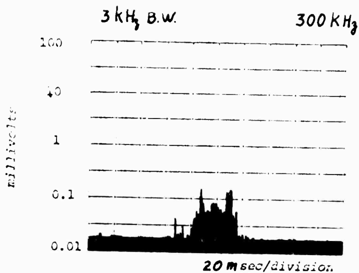
Figure 28. Emission output vs. time of very late stage near failure (20 m Sec/div.).
