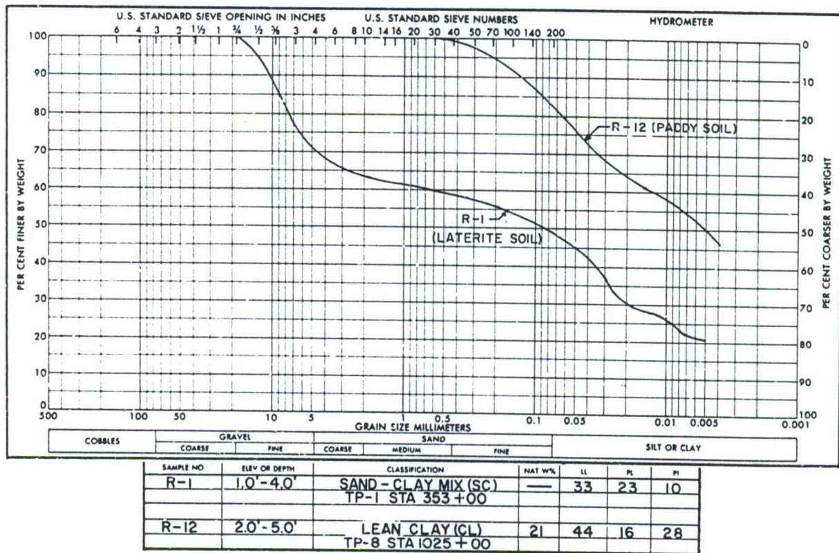
Figure IIA. Gradation curves.
