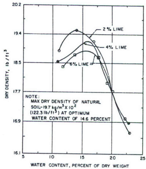
Figure 5. Lime-laterite soil.
