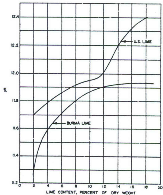
Figure 1B. Correlation of pH vs lime content of Burma and U. S. lime.
