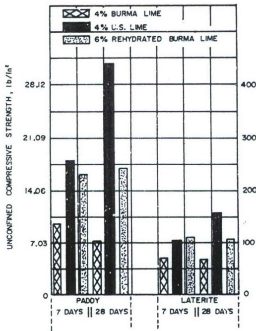
Figure 1A. Comparison of unconfined compressive strength for Burma and U. S. lime.
