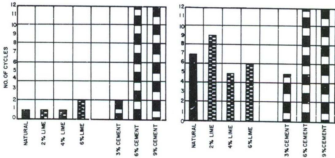
Figure 10. Laterite soil.
