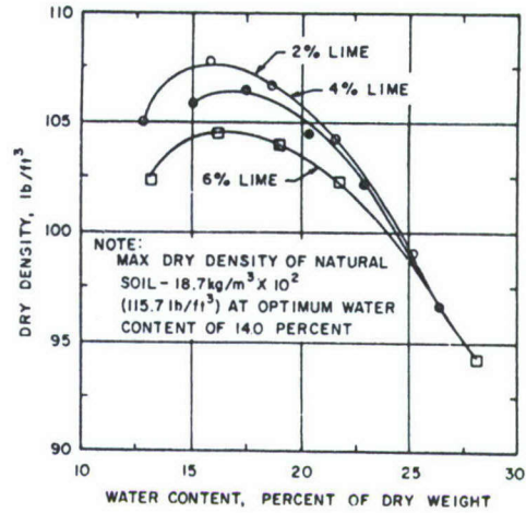
Figure 3. Lime-paddy soil.
