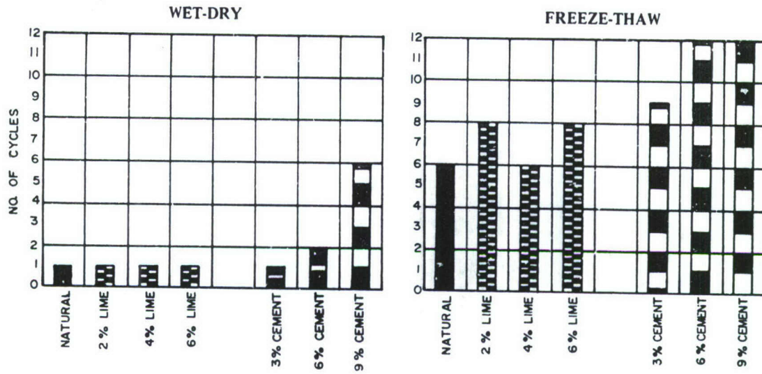
Figure 9. Paddy soil.
