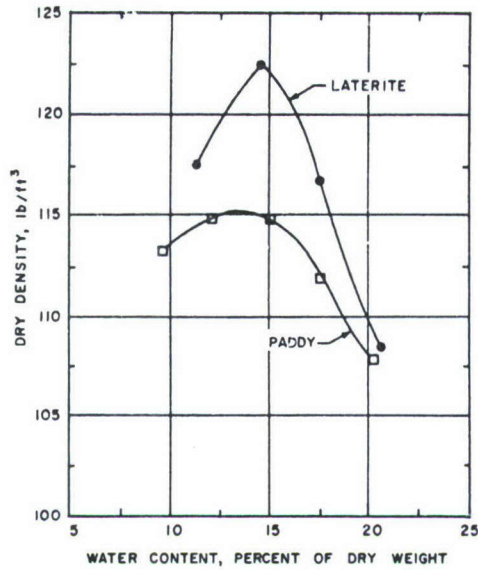
Figure 2. Natural soil.
