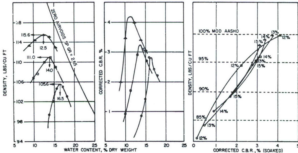
Figure IIC. Laterite soil: project 63-20; test pit #1; station 353+00; sample #R-1; depth 1.0 – 4.0 ft.
