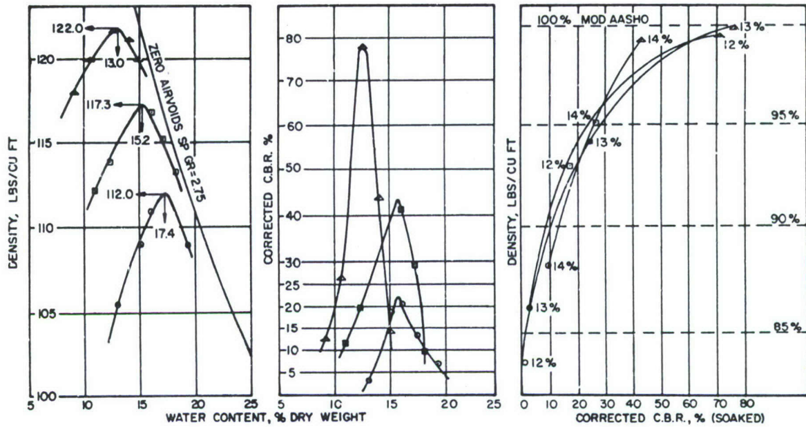
Figure IIB. Paddy soil: project 63-02; test pit #8; station 1025+00; sample #R-12; depth 2.0 – 5.0 ft.
