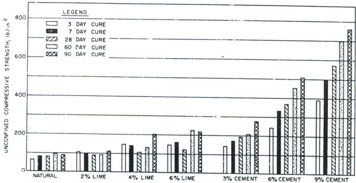
Figure 7. Paddy soil.
