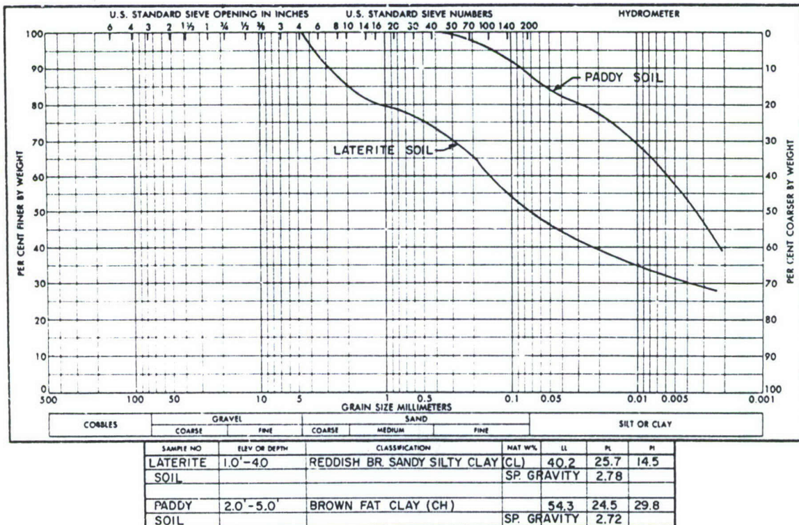
Figure 1. Burma soils gradation curves.
