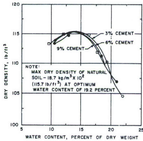
Figure 4. Cement-paddy soil.
