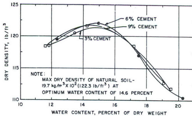
Figure 6. Cement-laterite soil.
