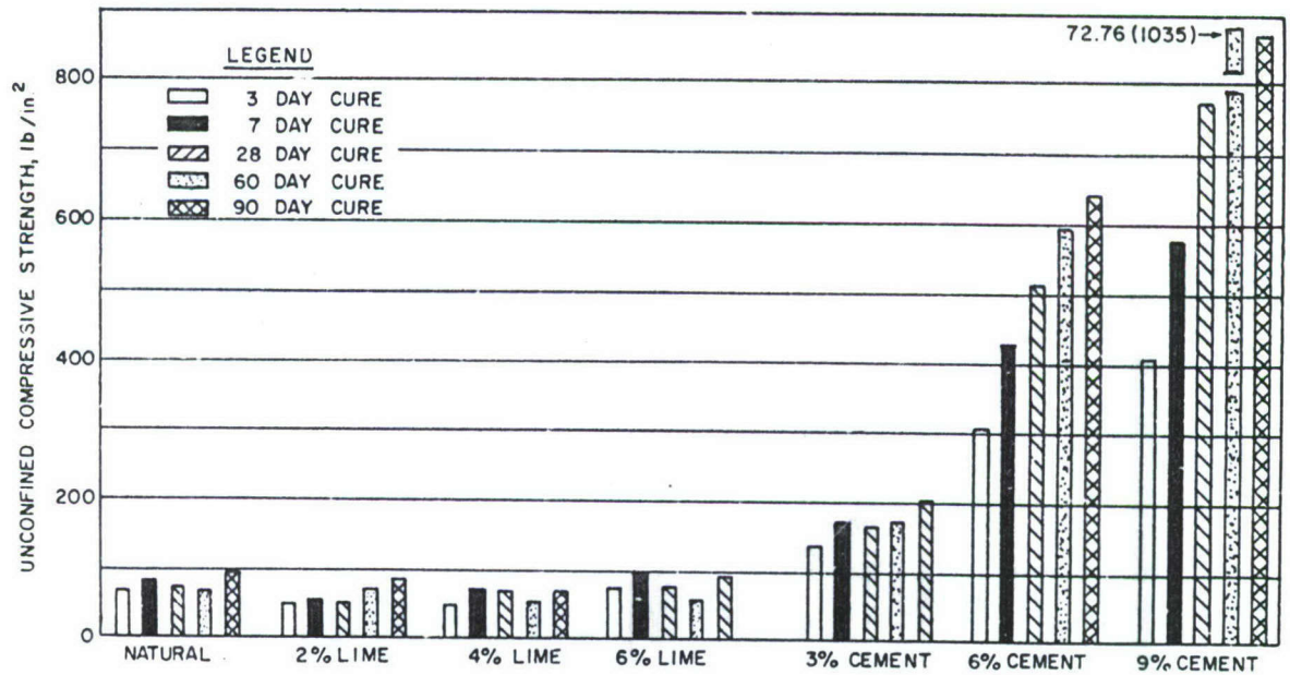
Figure 8. Laterite soil.
