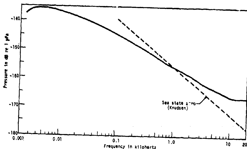
Fig. 8. Equivalent noise pressure, type H48 hydrophone.
