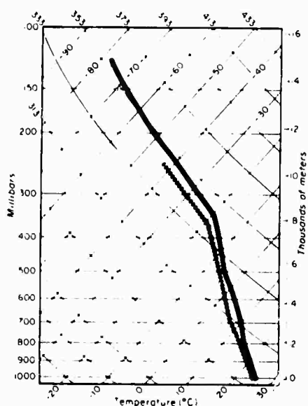
Figure 14.--Skew T, Log P Diagram for Koror Island at 1200 GMT, 25 November 1962. Temperatures given by solid line and dewpoint by dashed line.
