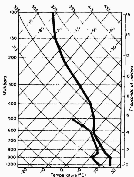
Figure 90.--Skew T, Log P Diagram for Saigon, Vietnam at 0000 GMT, 9 March 1963. Temperatures given by solid line and dewpoints by the dashed line.
