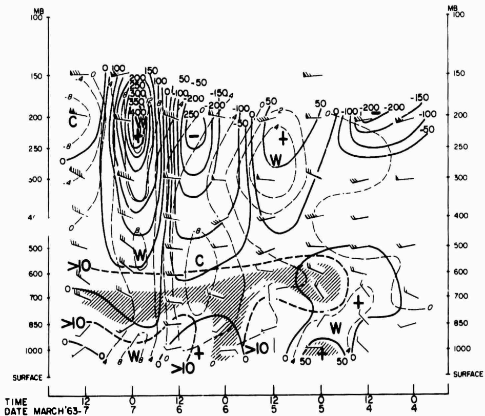
Figure 82.--Vertical time cross-section at Calcutta, India, 4-7 March 1963. Heavy solid lines are 24-hour height change in meters, with the 24-hour temperature change in °C (thin dashed lines), the boundary of more than 10°C dewpoint depression (heavy dashed lines), and less than 5°C dewpoint depression (shaded).
