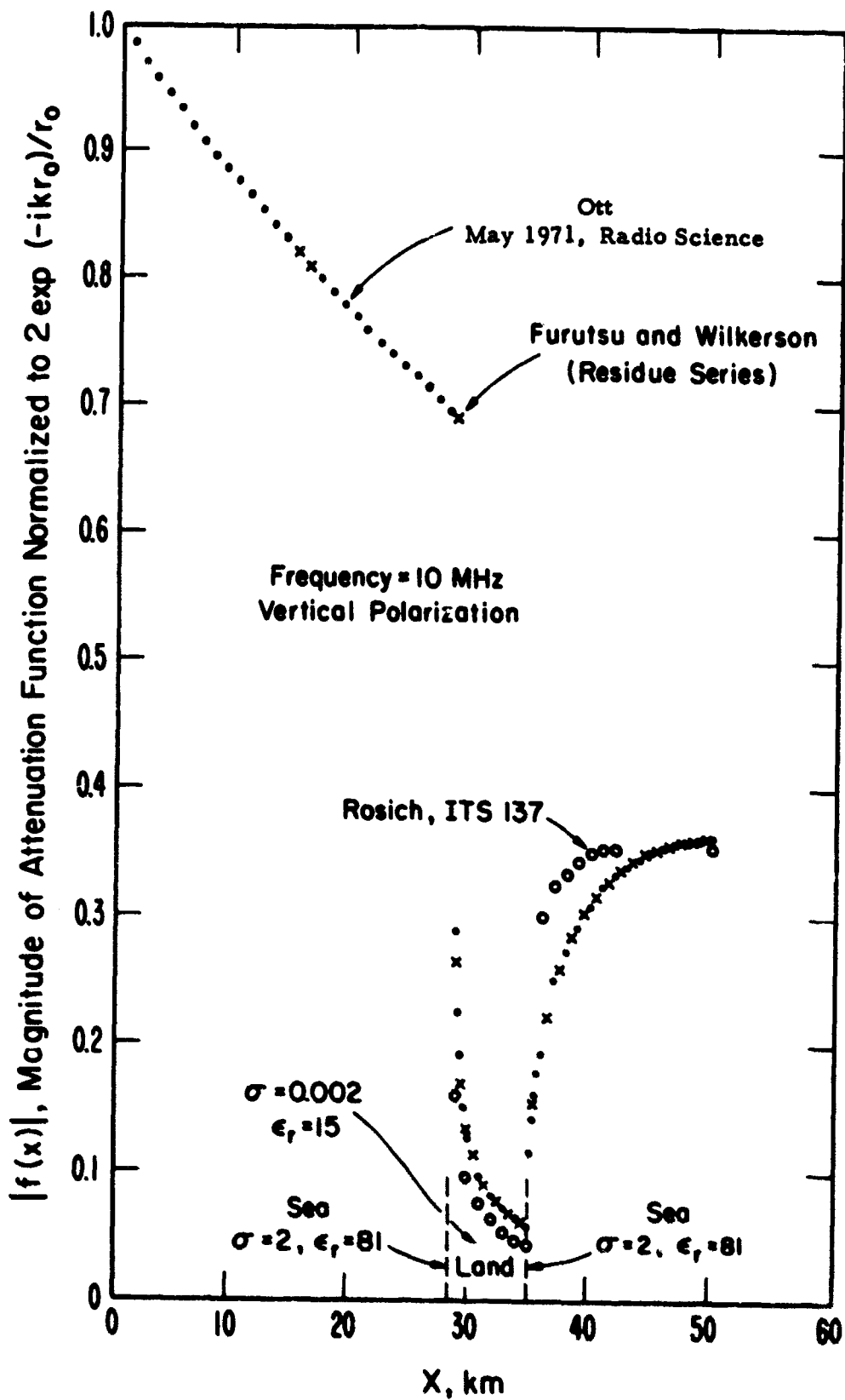
Figure 5. A sea-land-sea path. The profile is flat.
