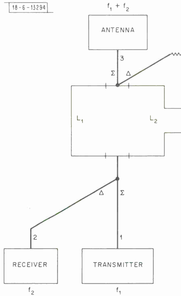
Fig. 1. A differential line length diplexer arrangement.
