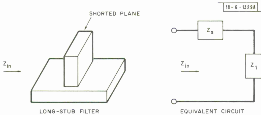
Fig. 4. Configuration and equivalent circuit of a long-stub filter.
