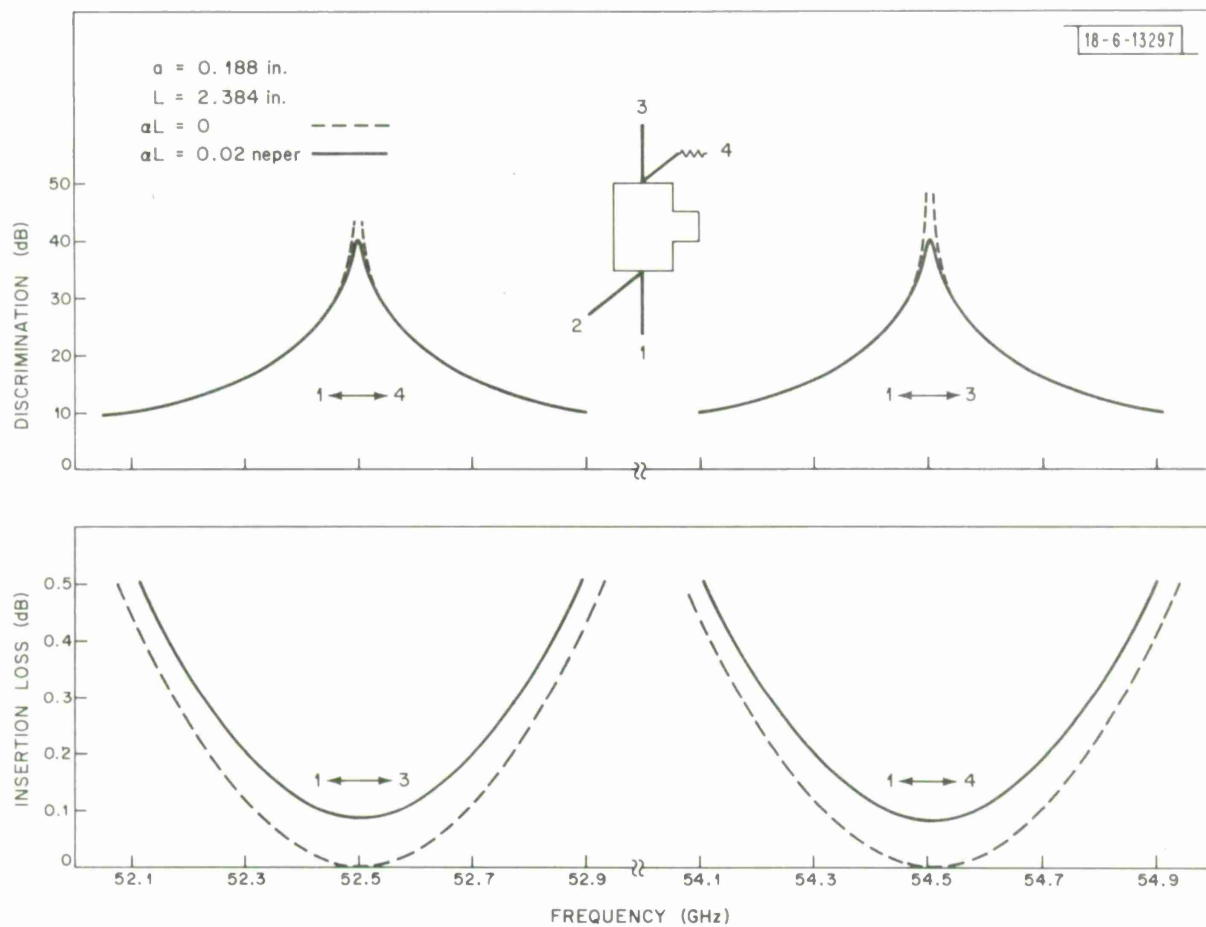
Fig. 3. An EHF differential line length diplexer characteristics.
