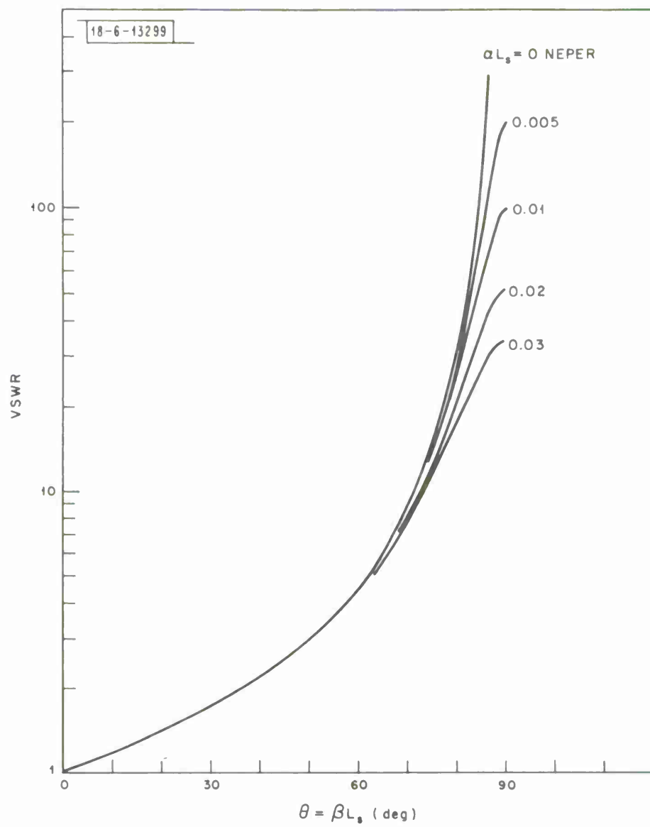
Fig. 5(a). Long-stub filter VSWR characteristics.
