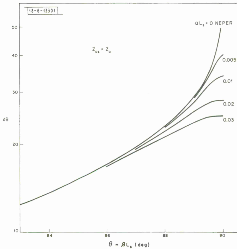
Fig. 5(c). Long-stub filter rejection characteristics.
