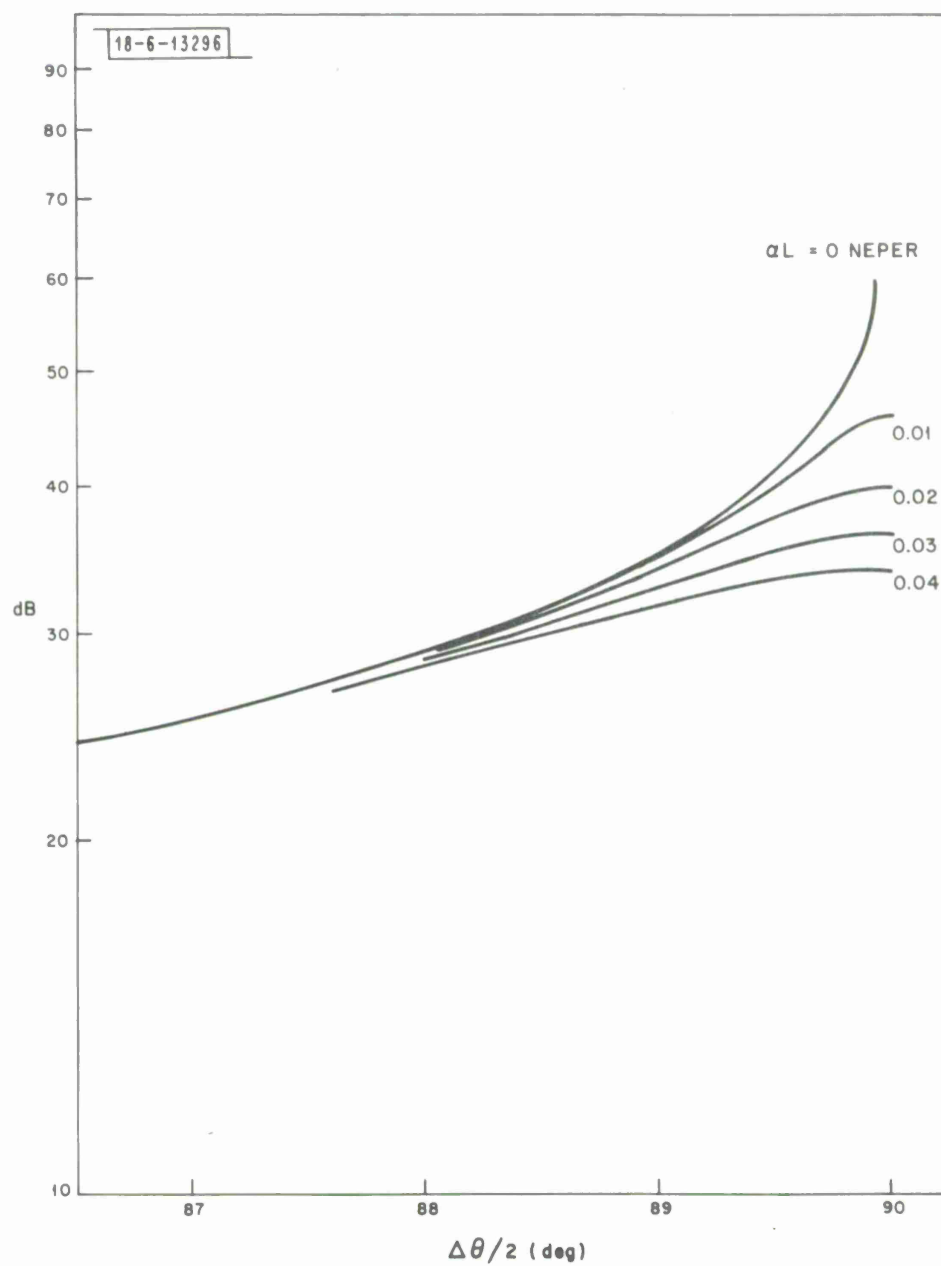
Fig. 2(b). Differential line length duplexer discrimination characteristics.
