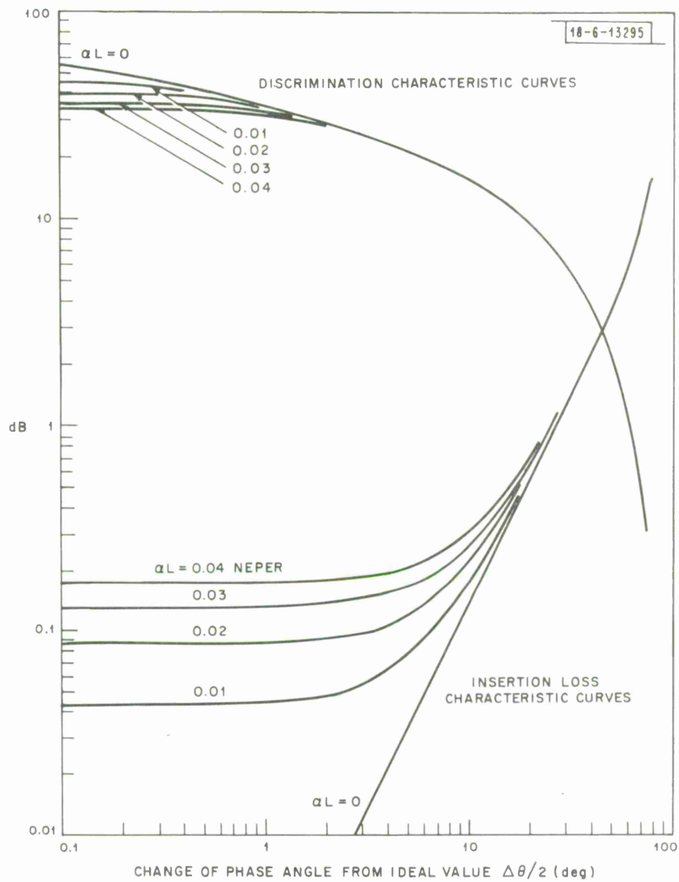
Fig. 2(a). Differential line length diplexer general characteristics.
