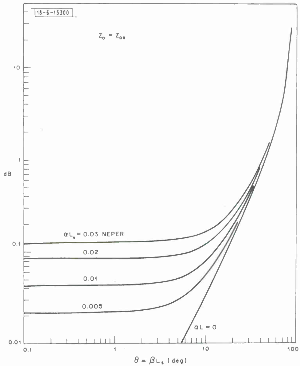
Fig. 5(b). Long-stub filter insertion loss characteristics.
